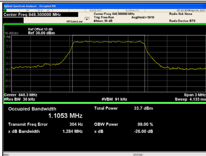
Band5-1.4MHz-QPSK-20643-6RB#0
