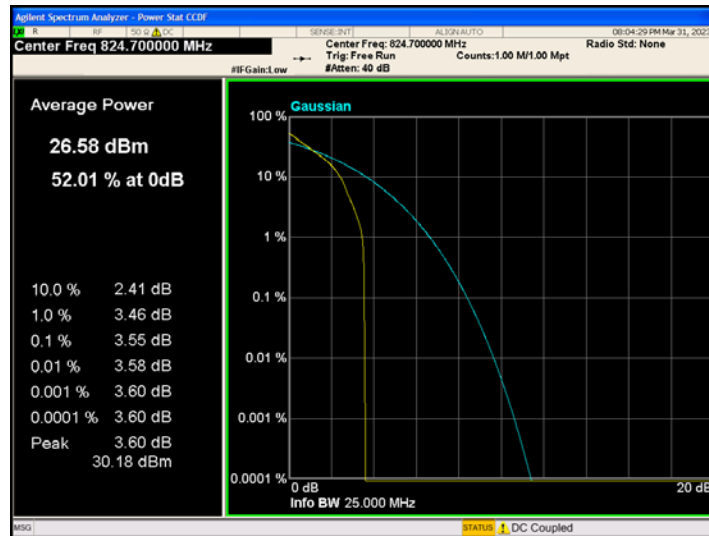
Band5-1.4MHz-QPSK-20407-6RB#0
