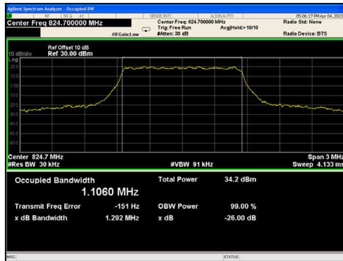
Band5-1.4MHz-QPSK-20525-6RB#0
