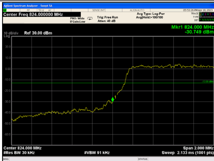
Band5-1.4MHz-QPSK-20407-6RB#0
