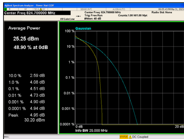
Band5-1.4MHz-QPSK-20525-1RB#0
