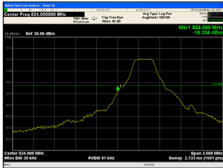
Band5-1.4MHz-QPSK-20407-1RB#5
