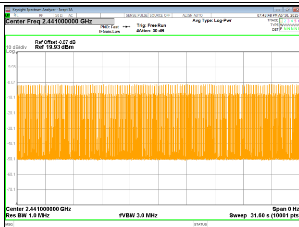
2DH3-2441MHz-Accumulated
