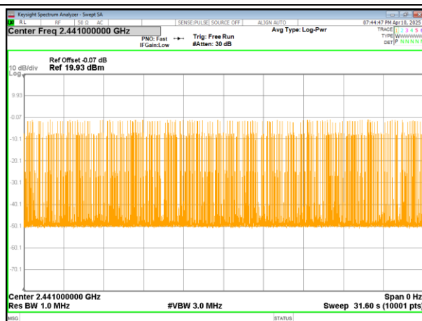
2DH5-2441MHz-Accumulated
