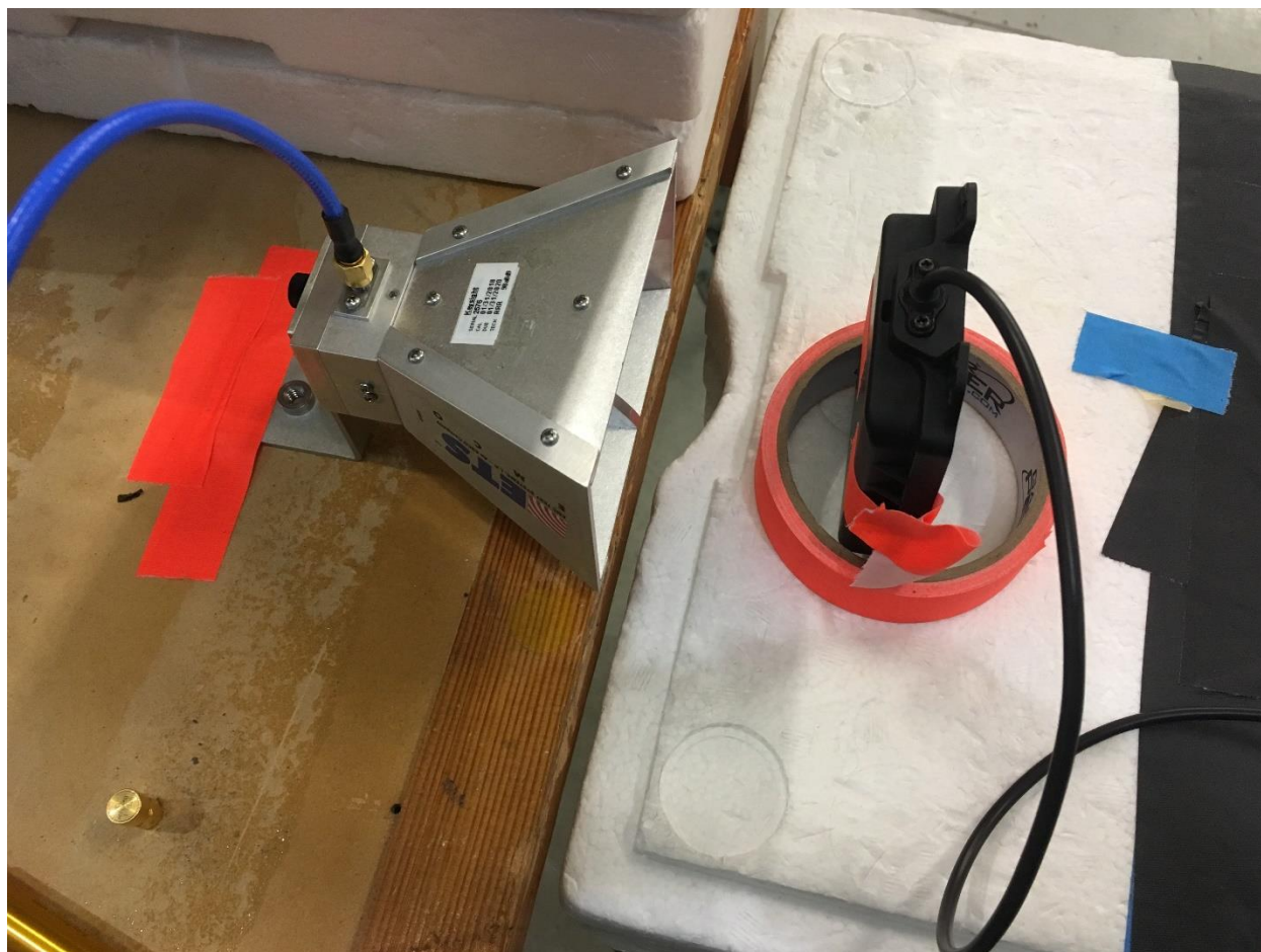
Test setup for band edge measurements
