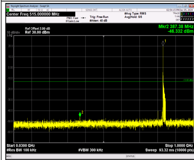
Band26-15MHz-16QAM-26965-1RB#0-Range1:30~1000MHz
