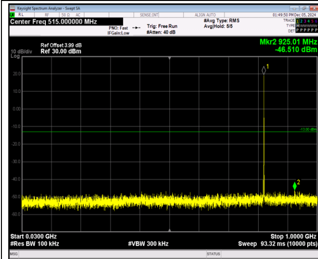
Band26-1.4MHz-64QAM-26915-1RB#0-Range1:30~1 000MHz
