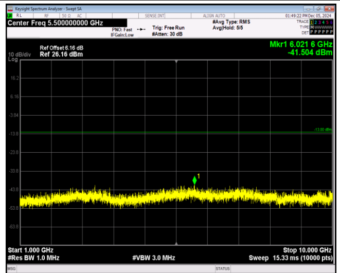
Band26-1.4MHz-QPSK-26915-1RB#0-Range2:1000~10000MHz
