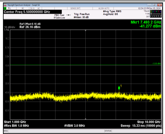
Band26-15MHz-16QAM-26965-1RB#0-Range2:1000~10000MHz
