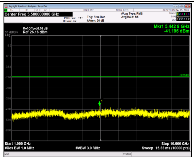
Band26-15MHz-16QAM-26915-1RB#0-Range2:1000~10000MHz
