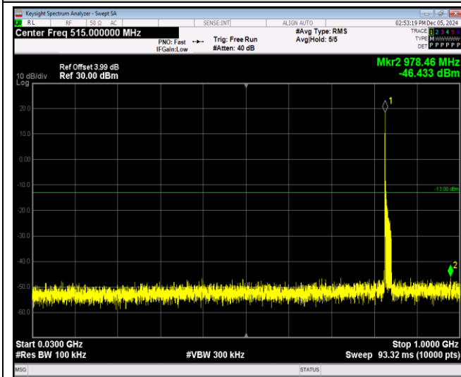
Band26-15MHz-16QAM-26965-1RB#0-Range1:30~1000MHz
