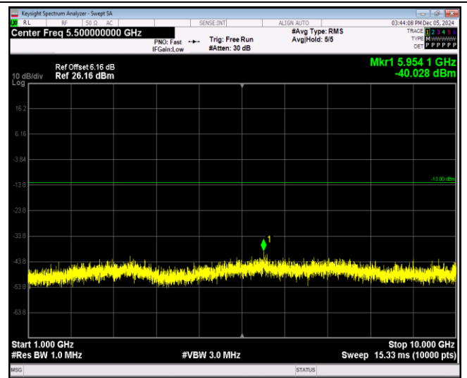
Band26-1.4MHz-64QAM-26797-1RB#0-Range2:1000 ~10000MHz
