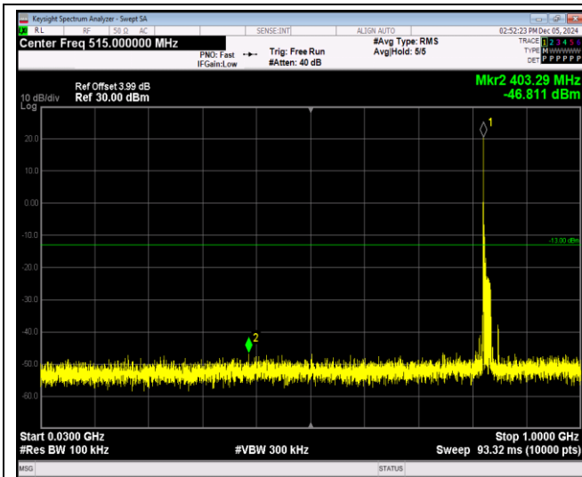
Band26-15MHz-16QAM-26915-1RB#0-Range1:30~1000MHz
