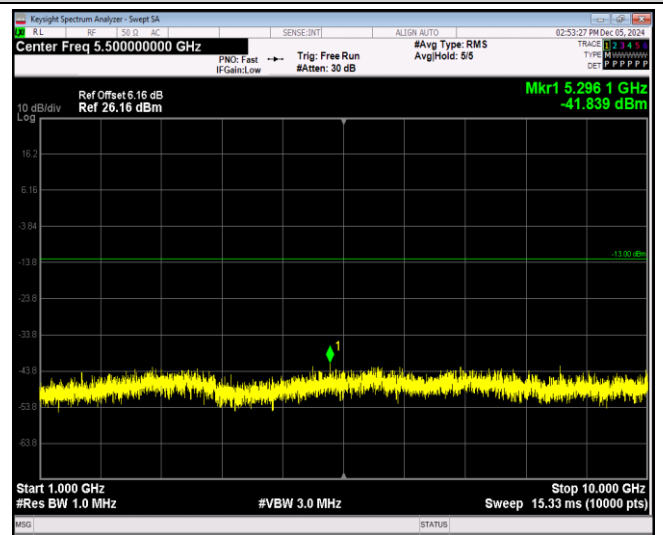
Band26-15MHz-16QAM-26965-1RB#0-Range2:1000~10000MHz
