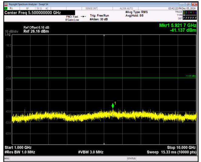
Band26-1.4MHz-16QAM-26783-1RB#0-Range2:1000 ~10000MHz
