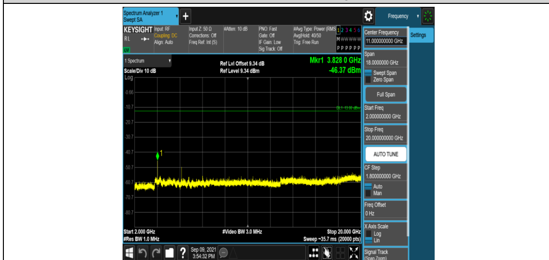
Band25-1.4MHz-QPSK-26683-1RB#0-Range5:2000~20000MHz
