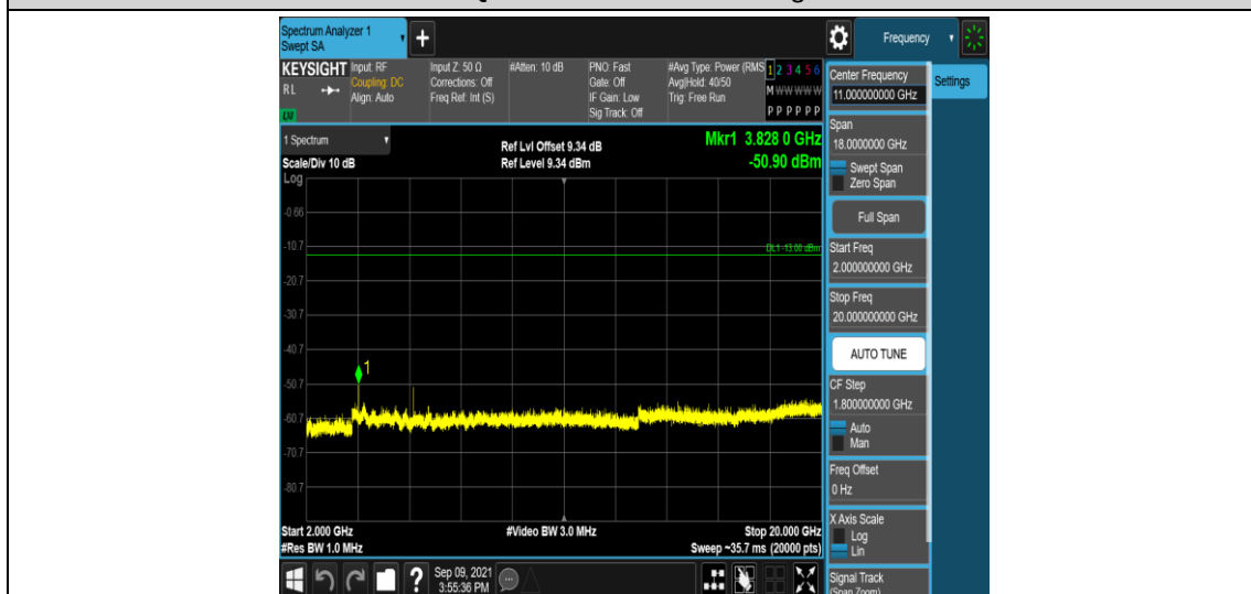
Band25-1.4MHz-16QAM-26683-1RB#0-Range5:2000~20000MHz
