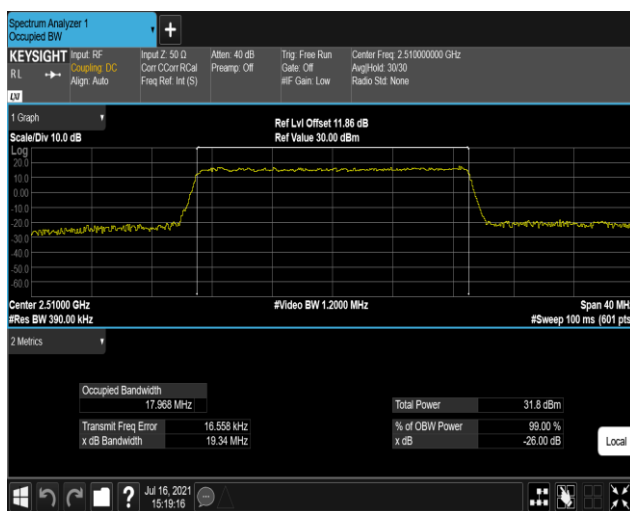
Band7-20MHz-QPSK-21350-100RB#0
