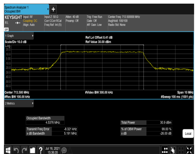
Band17-5MHz-16QAM-23825-25RB#0
