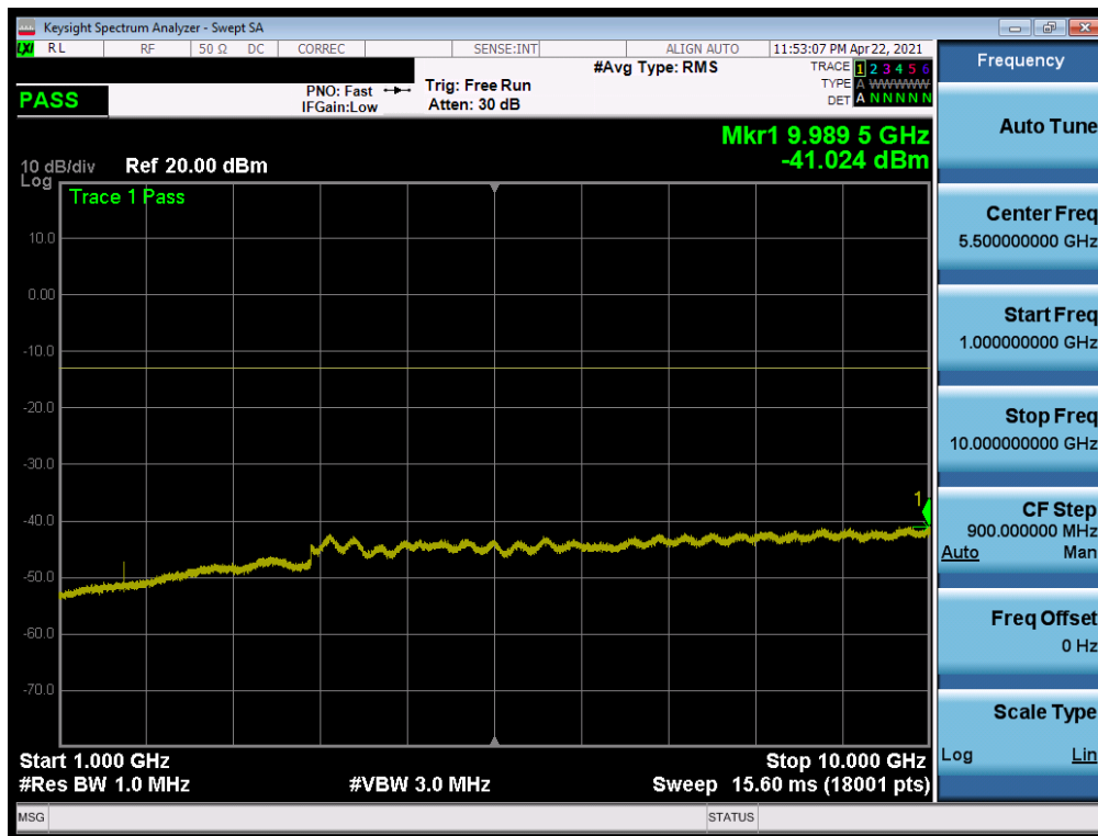
Plot 7-32. Conducted Spurious Plot (LTE Band 26/5 10MHz QPSK 1 RB Mid Channel)
