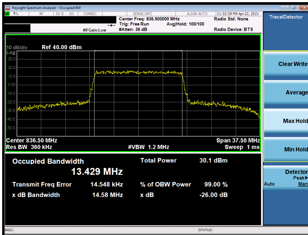
Plot 7-2. Occupied Bandwidth Plot (LTE Band 26 15MHz 16-QAM Full RB)
