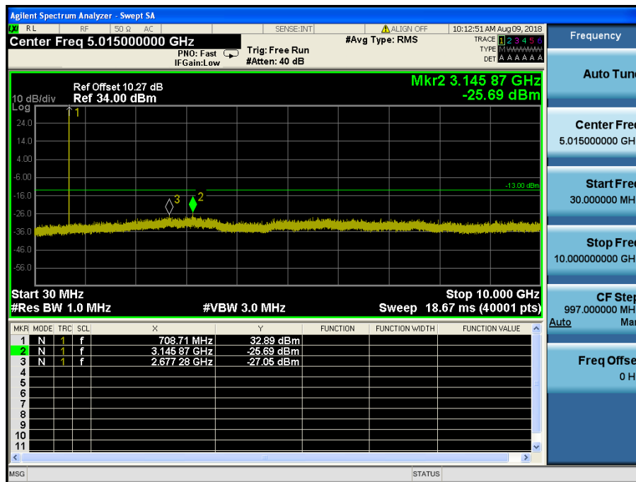
LTE Band 12,17 / 10MHz / 16QAM - RB Size/Offset (1/49) – Low Channel
