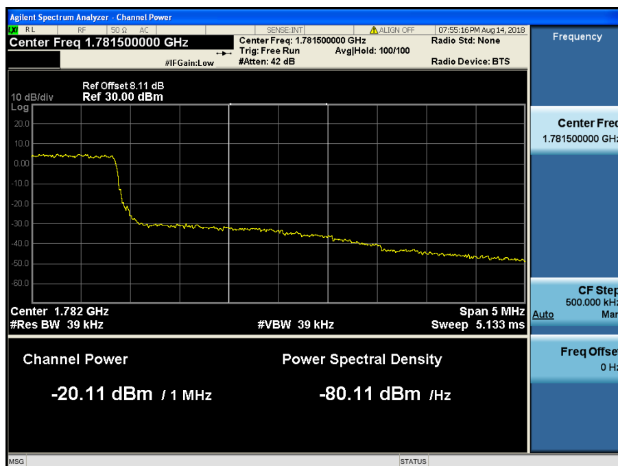
LTE Band 4,66 / 3MHz / 16QAM - RB Size/Offset (15/0)
