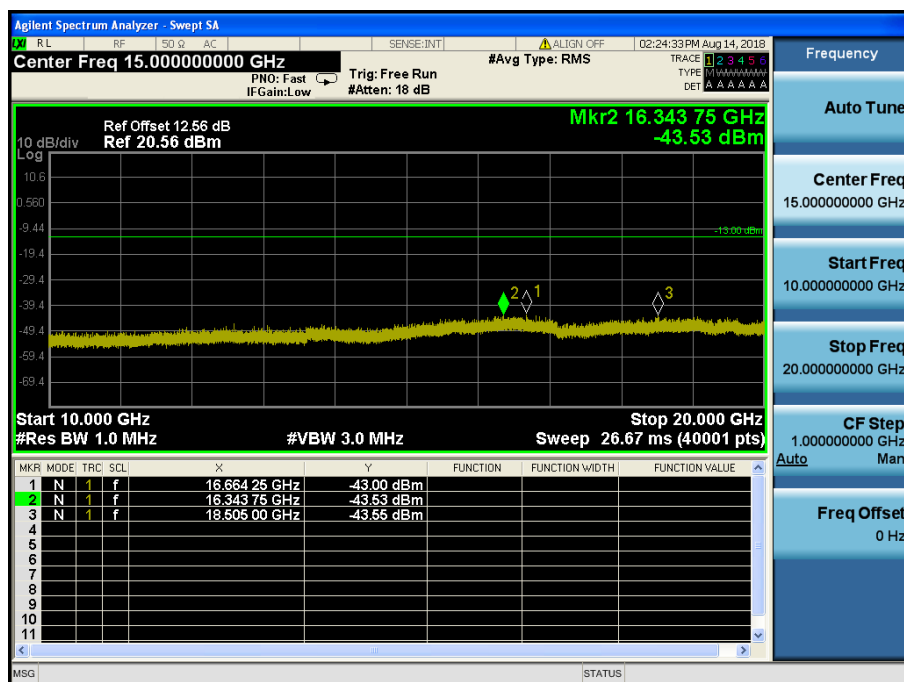
LTE Band 4,66 / 15MHz / QPSK - RB Size/Offset (1/36) – Mid Channel
