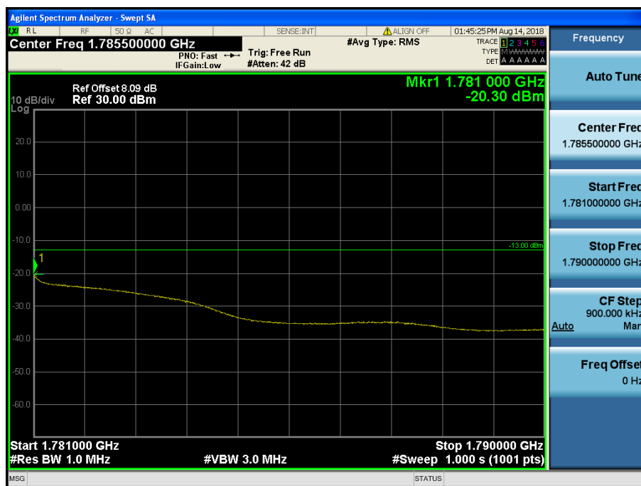
LTE Band 4,66 / 10MHz / QPSK - RB Size/Offset (25/25)
