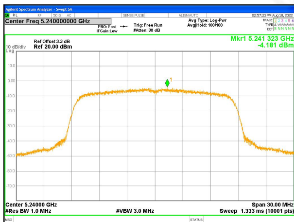
(802.11a20) PSD plot on channel 48
