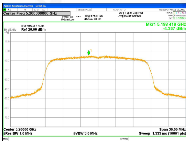
(802.11a20) PSD plot on channel 40
