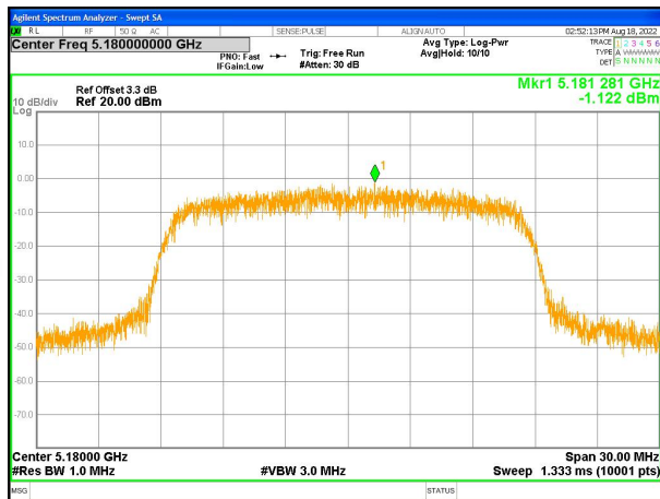
(802.11a20) PSD plot on channel 36
