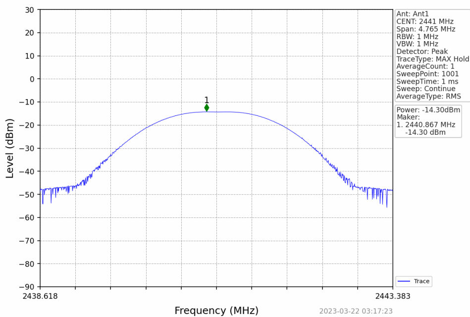
GFSK_DH5_MCH_2441MHz
