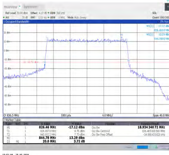
1-N26-824-849-15-20-M-7-CP-16QAM-Outter_Full-1 06@0-Ant1-18.934-20.000-≤20-PASS
