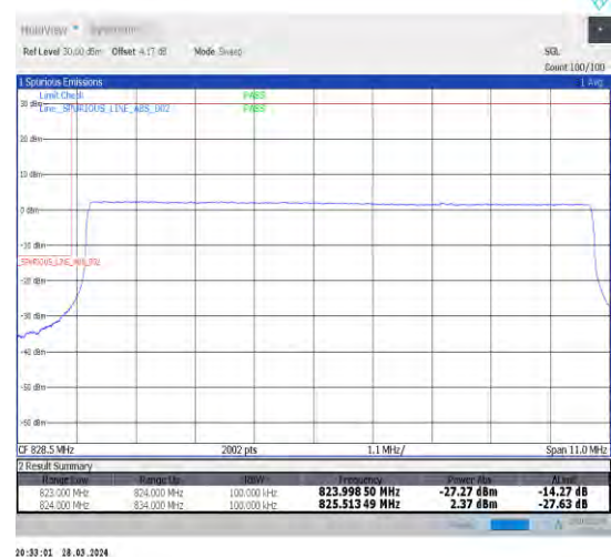
1-N26-824-849-15-10-L-6-CP-QPSK-Outer_Full-5 2@0-Ant1-1-seegraph-PASS-see graph
