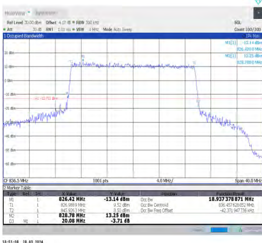
1-N26-824-849-15-20-M-8-CP-64QAM-Outter_Full-10 6@0-Ant1-18.937-20.080-≤20-PASS
