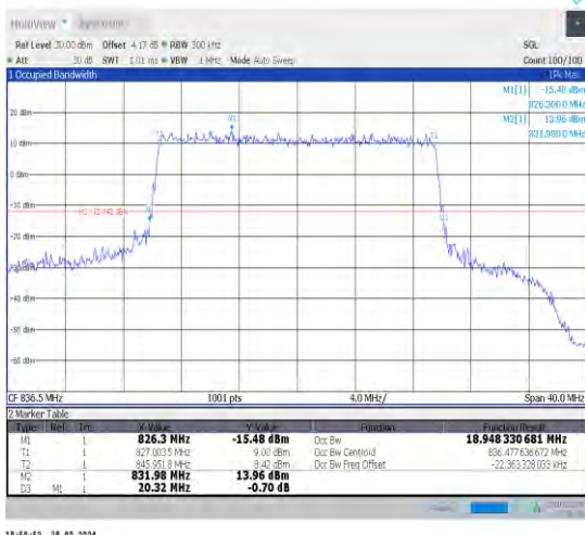
1-N26-824-849-15-20-M-6-CP-QPSK-Outter_Full-106 @0-Ant1-18.948-20.320-≤20-PASS
