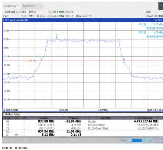
1-N26-824-849-15-5-M-9-CP-256QAM-Outer_Full-25 @0-Ant1-4.475-5.120-≤5-PASS
