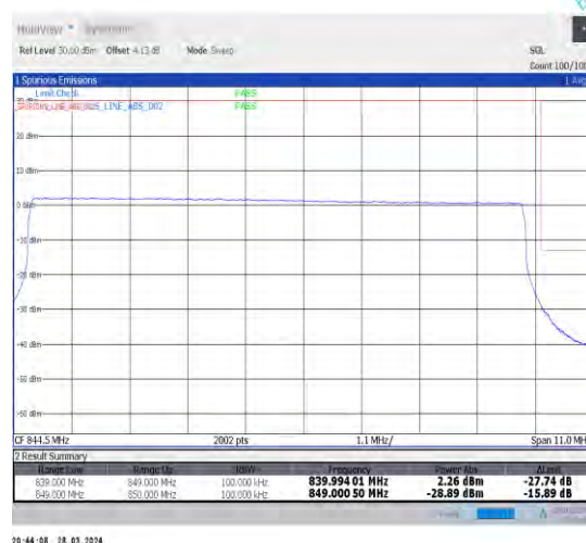
1-N26-824-849-15-10-H-6-CP-QPSK-Outer_Full-52@0-Ant1-1-seegraph-PASS-see graph
