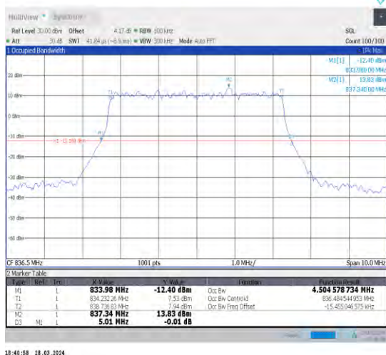
1-N26-824-849-15-5-M-5-DFT-256QAM-Outer_Full-2 5@0-Ant1-4.505-5.010-≤5-PASS
