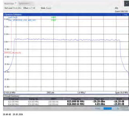
1-N26-824-849-15-15-L-3-DFT-PI2BPSK-Outer_F ull-75@0-Ant1-1-seegraph-PASS-see graph
