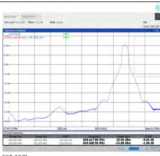
1-N26-824-849-15-5-H-2-DFT-PI2BPSK-Edge_1RB_Right-1@24-Ant1-1-seegraph-PASS-see graph
