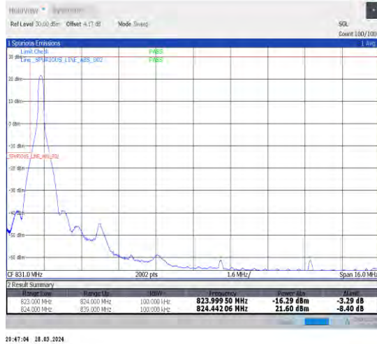
1-N26-824-849-15-15-L-1-DFT-PI2BPSK-Edge_1RB_L eft-1@0-Ant1-1-seegraph-PASS-see graph
