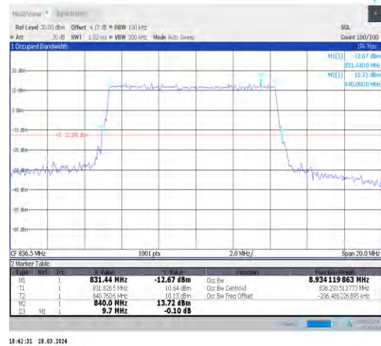
1-N26-824-849-15-10-M-1-DFT-QPSK-Outer_Full-50 @0-Ant1-8.934-9.700-≤10-PASS
