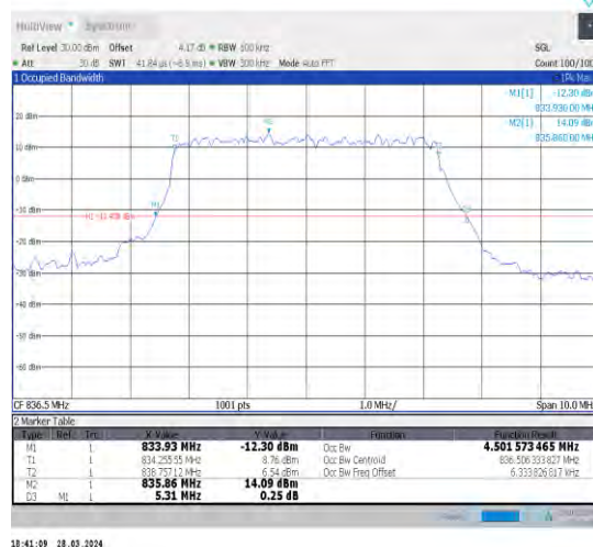
1-N26-824-849-15-5-M-6-CP-QPSK-Outer_Full-25@ 0-Ant1-4.502-5.310-≤5-PASS
