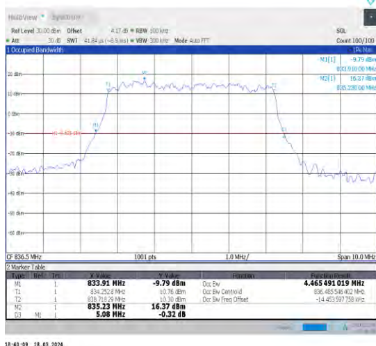
1-N26-824-849-15-5-M-1-DFT-QPSK-Outet_Full-25 @0-Ant1-4.465-5.080-≤5-PASS
