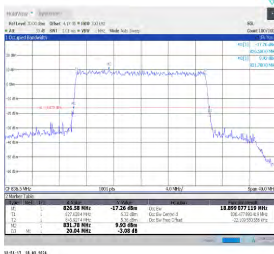
1-N26-824-849-15-20-M-9-CP-256QAM-Outter_Full- 106@0-Ant1-18.899-20.040-≤20-PASS
