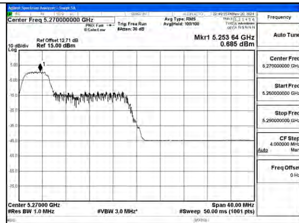
Mode:802.11ax HE40 Tone:52T Frequency:5270MHz Ant:Chain0
