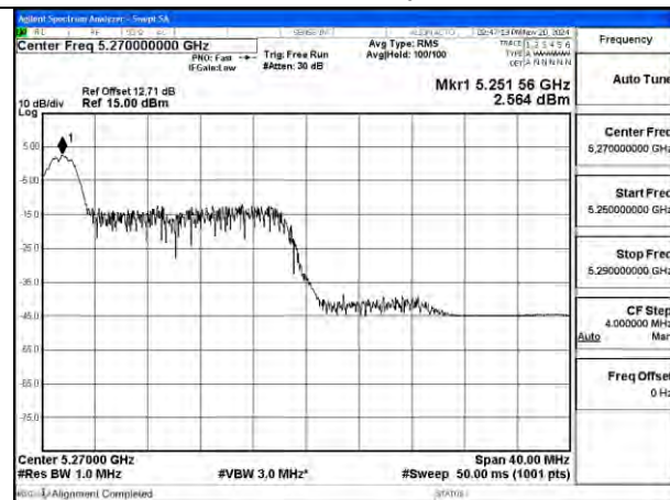
Mode:802.11ax HE40 Tone:26T Frequency:5270MHz Ant:Chain1
