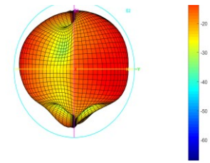
Total_Polar_E2_922MHz
