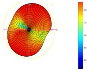
Total_Polar_H_922MHz
