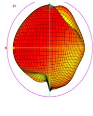
Total_Polar_E1_912MHz
