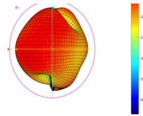
Total_Polar_E1_922MHz
