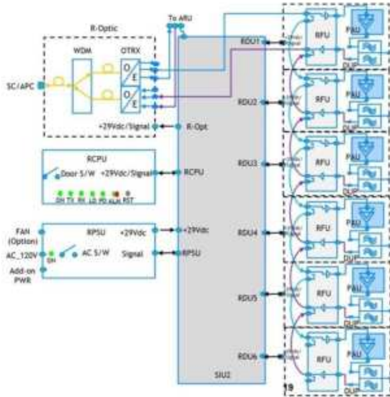
Figure 3.1 – Remote Unit Block Diagram
