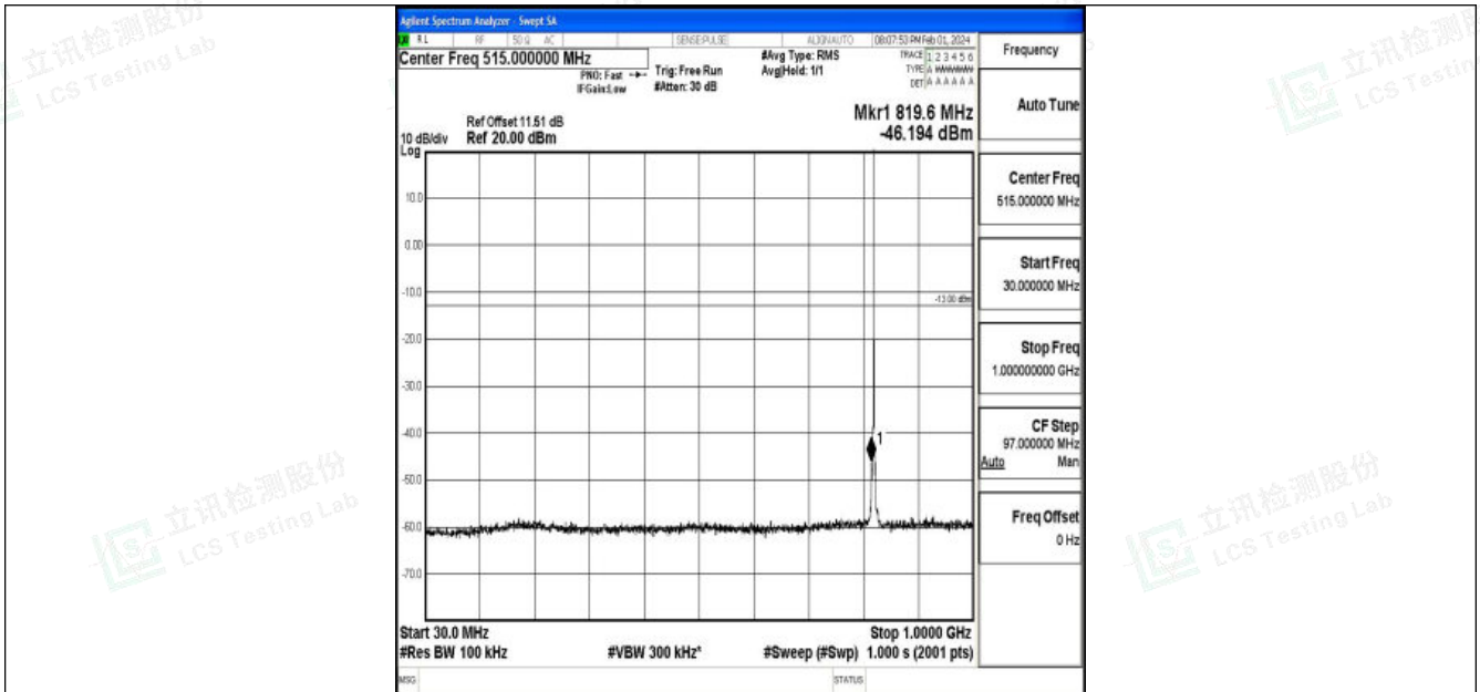
Band26_1.4MHz_QPSK_26783_1RB#0_30~1000_30~1000
