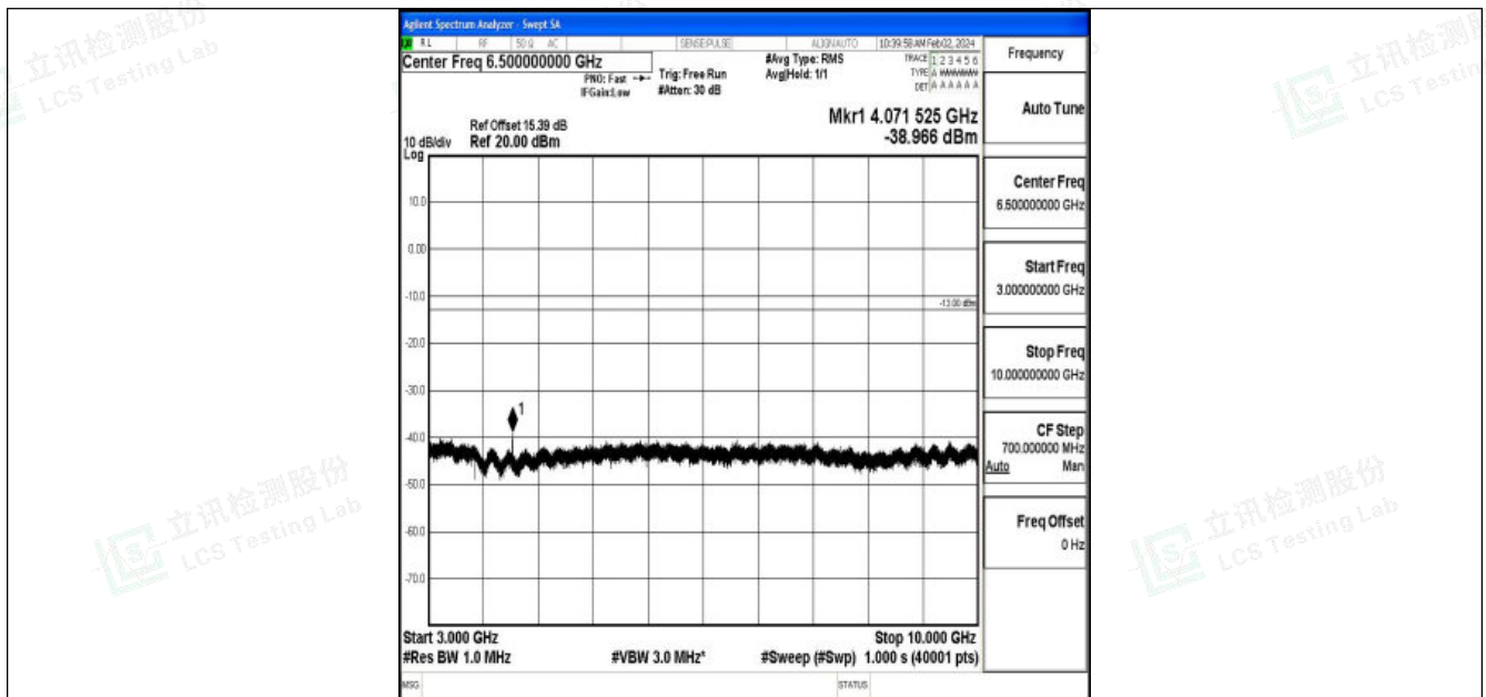
Band26_5MHz_QPSK_26715_1RB#0_3000~10000_3000~10000
