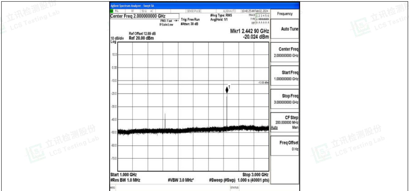
Band26_5MHz_16QAM_26715_1RB#0_1000~3000_1000~3000
