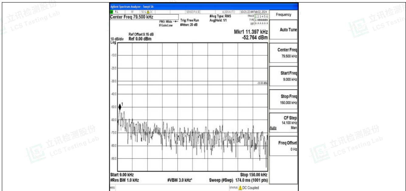
Band26_3MHz_QPSK_26775_1RB#0_0.009~0.15_0.009~0.15
