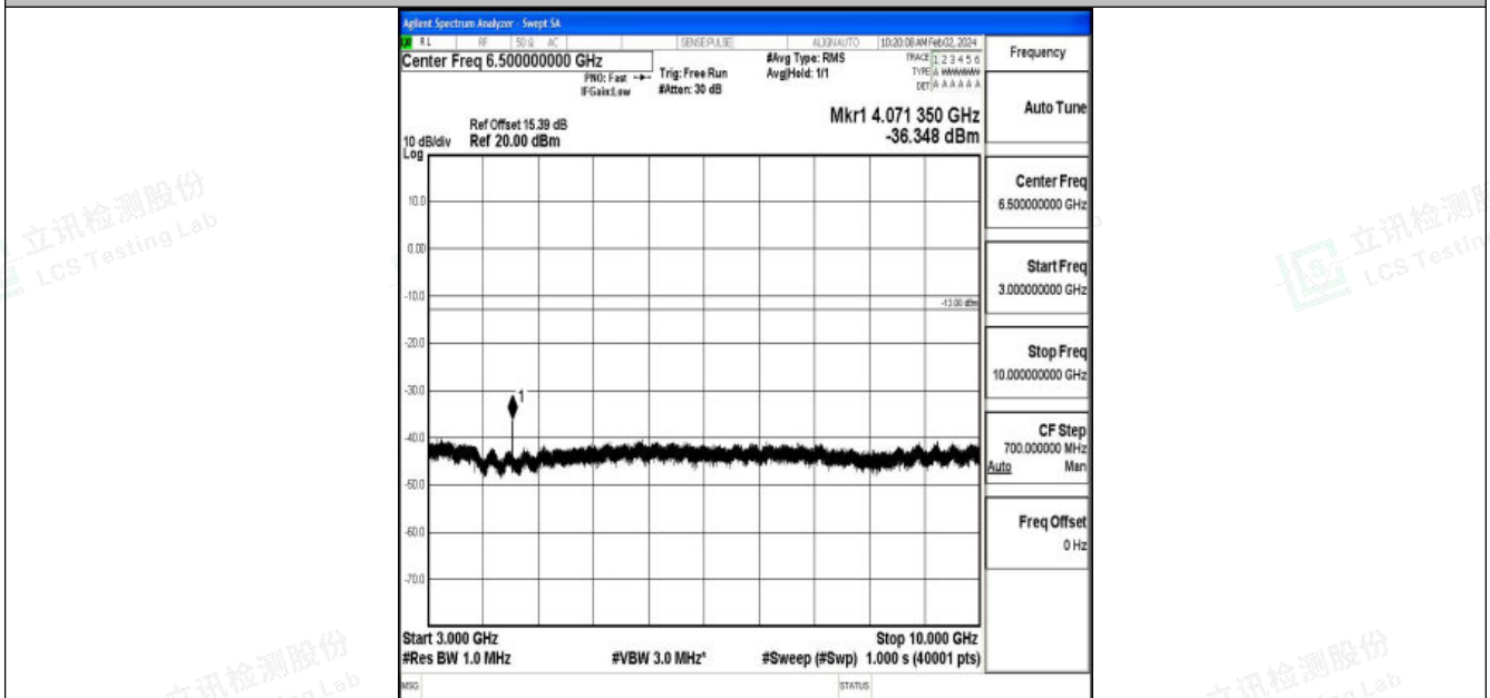
Band26_3MHz_16QAM_26705_1RB#0_3000~10000_3000~10000
