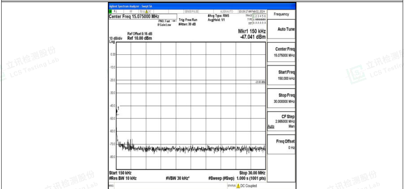
Band26_3MHz_QPSK_26705_1RB#0_0.15~30_0.15~30
