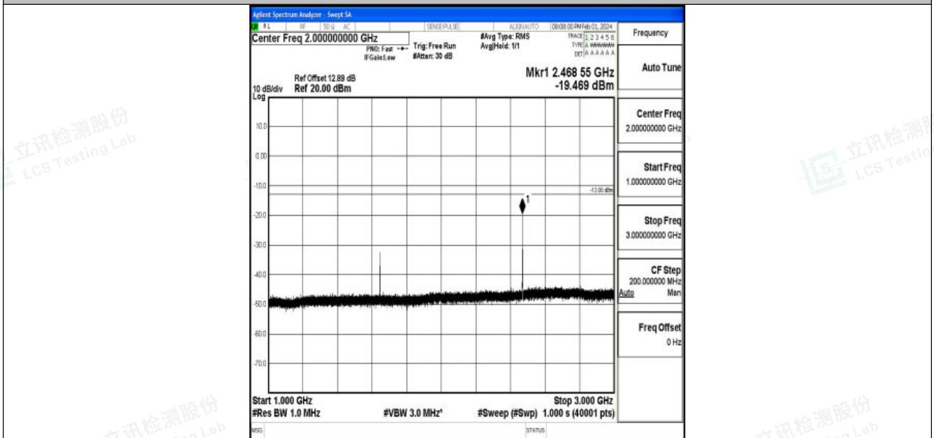
Band26_1.4MHz_QPSK_26783_1RB#0_1000~3000_1000~3000
