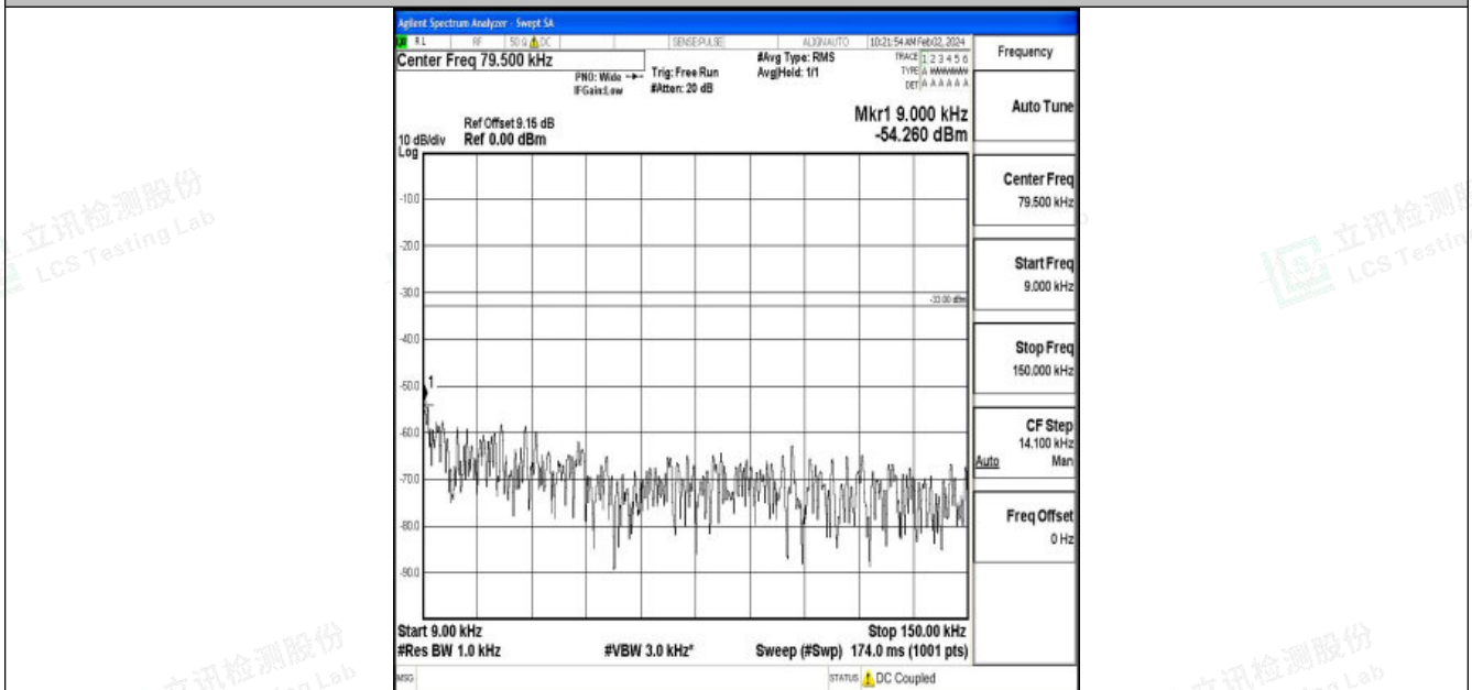
Band26_3MHz_16QAM_26775_1RB#0_0.009~0.15_0.009~0.15
