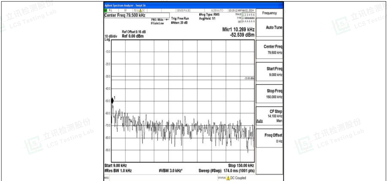
Band26_3MHz_QPSK_26705_1RB#0_0.009~0.15_0.009~0.15
