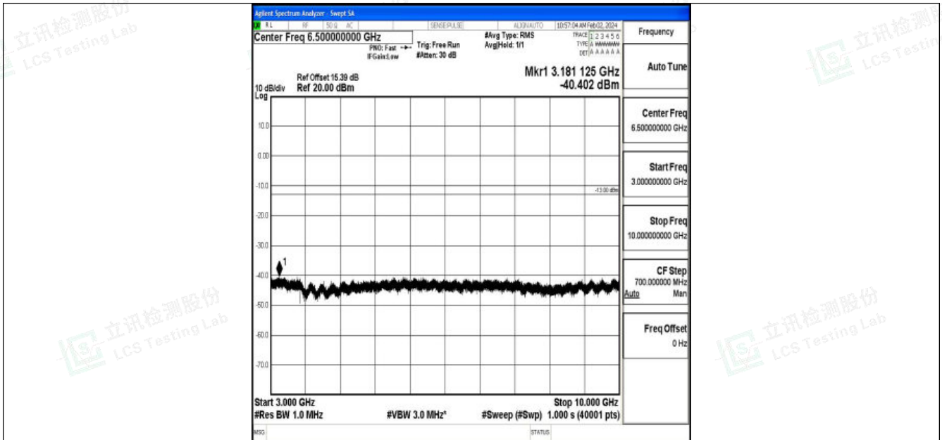
Band26_10MHz_QPSK_26740_1RB#0_3000~10000_3000~10000
