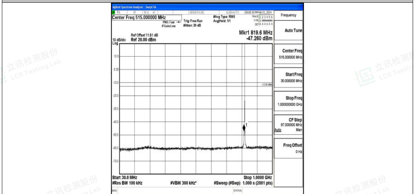
Band26_1.4MHz_16QAM_26783_1RB#0_30~1000_30~1000
