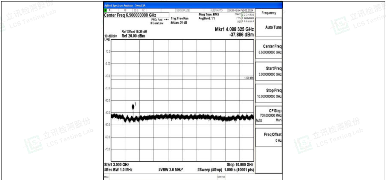
Band26_3MHz_QPSK_26740_1RB#0_3000~10000_3000~10000
