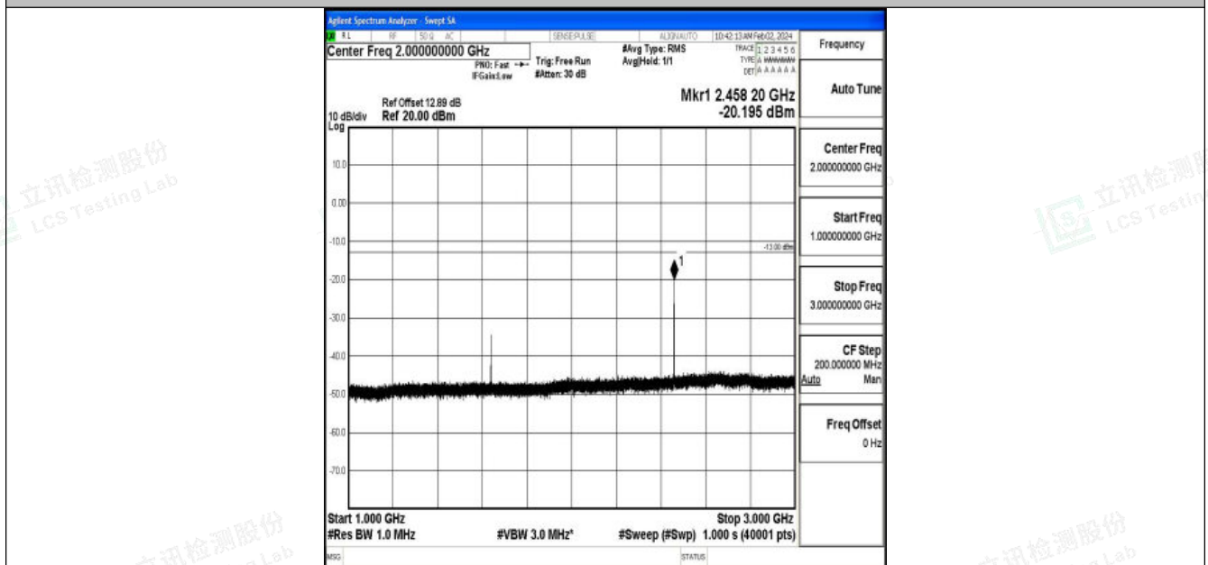
Band26_5MHz_QPSK_26765_1RB#0_1000~3000_1000~3000
