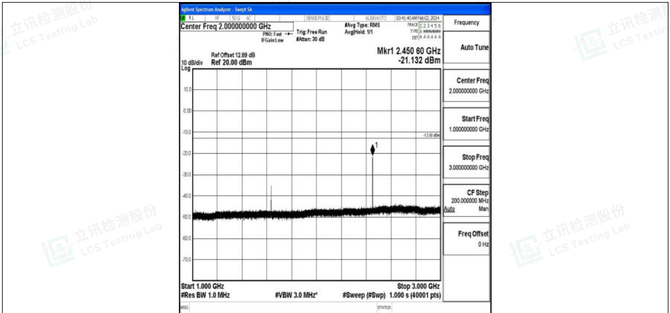
Band26_5MHz_16QAM_26740_1RB#0_1000~3000_1000~3000
