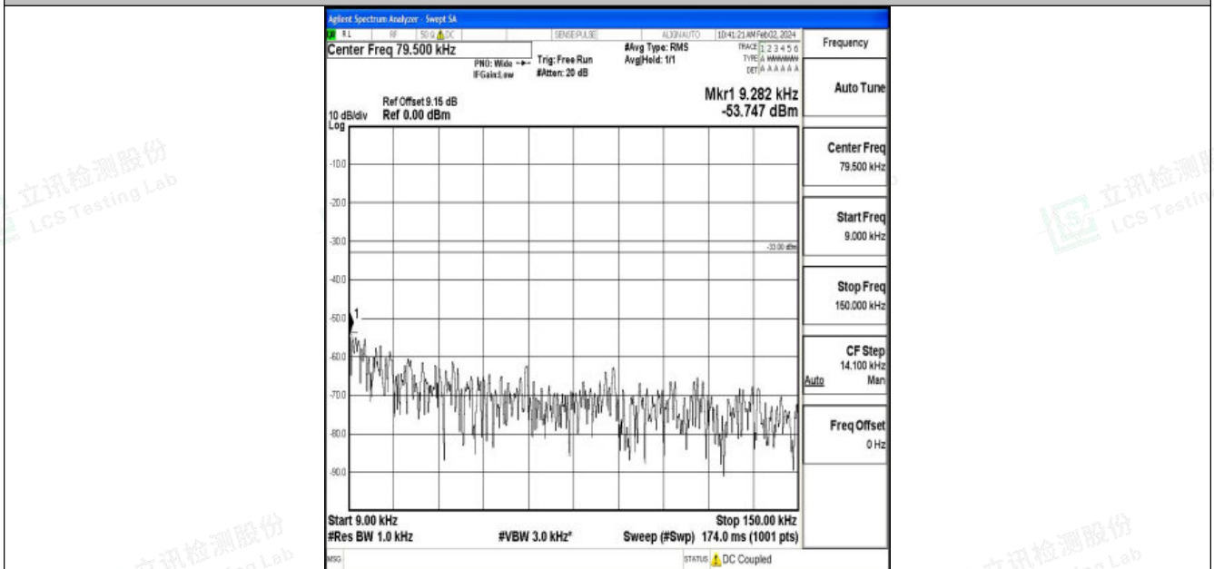
Band26_5MHz_16QAM_26740_1RB#0_0.009~0.15_0.009~0.15
