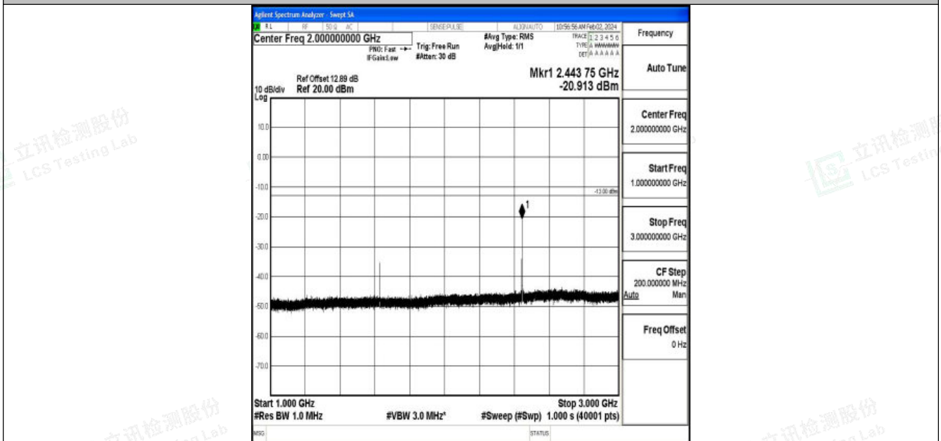
Band26_10MHz_QPSK_26740_1RB#0_1000~3000_1000~3000
