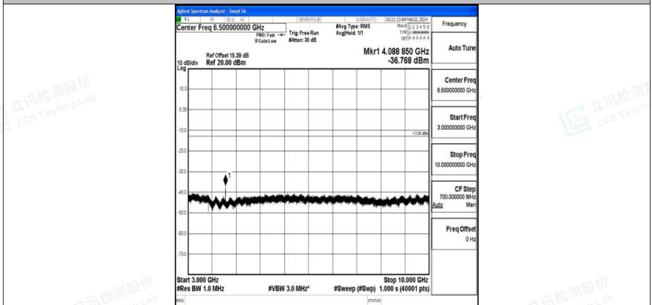
Band26_3MHz_16QAM_26740_1RB#0_3000~10000_3000~10000
