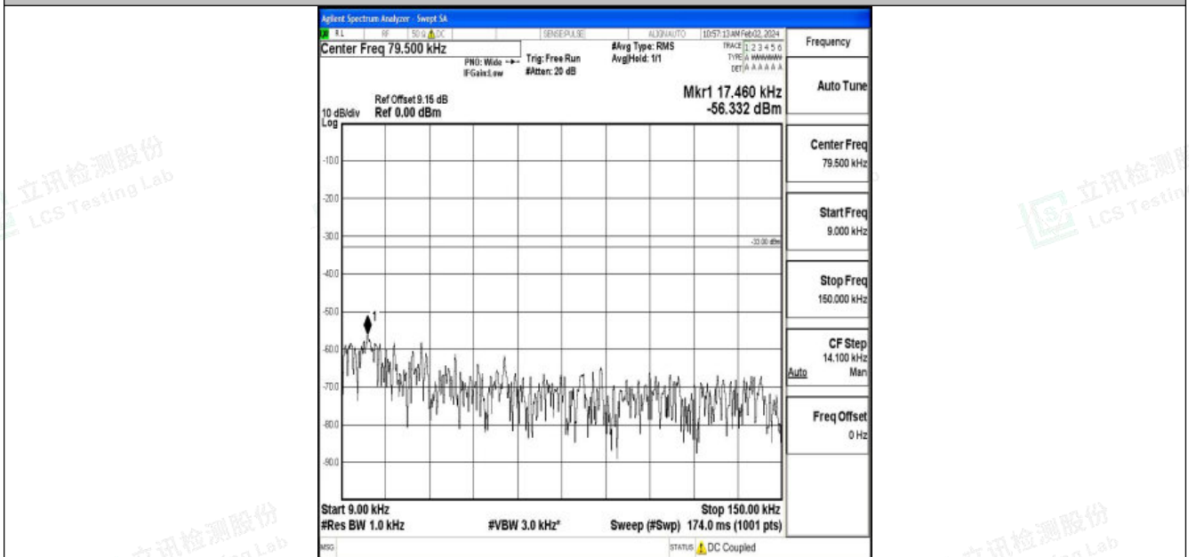
Band26_10MHz_16QAM_26740_1RB#0_0.009~0.15_0.009~0.15
