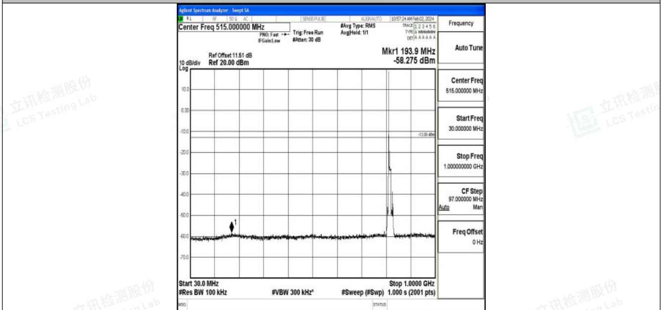
Band26_10MHz_16QAM_26740_1RB#0_30~1000_30~1000
