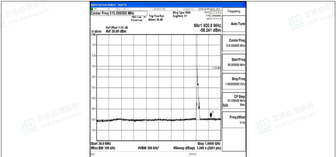
Band26_10MHz_QPSK_26740_1RB#0_30~1000_30~1000
