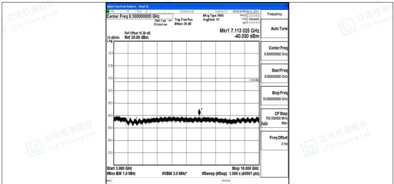
Band26_1.4MHz_QPSK_26783_1RB#0_3000~10000_3000~10000
