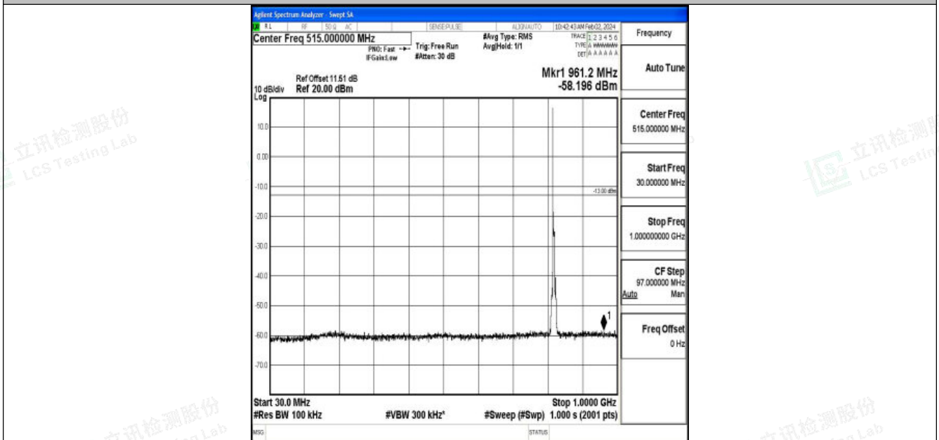
Band26_5MHz_16QAM_26765_1RB#0_30~1000_30~1000
