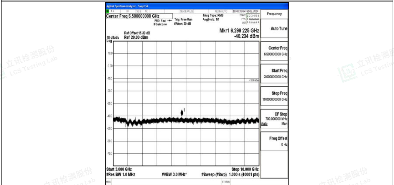
Band26_5MHz_16QAM_26715_1RB#0_3000~10000_3000~10000
