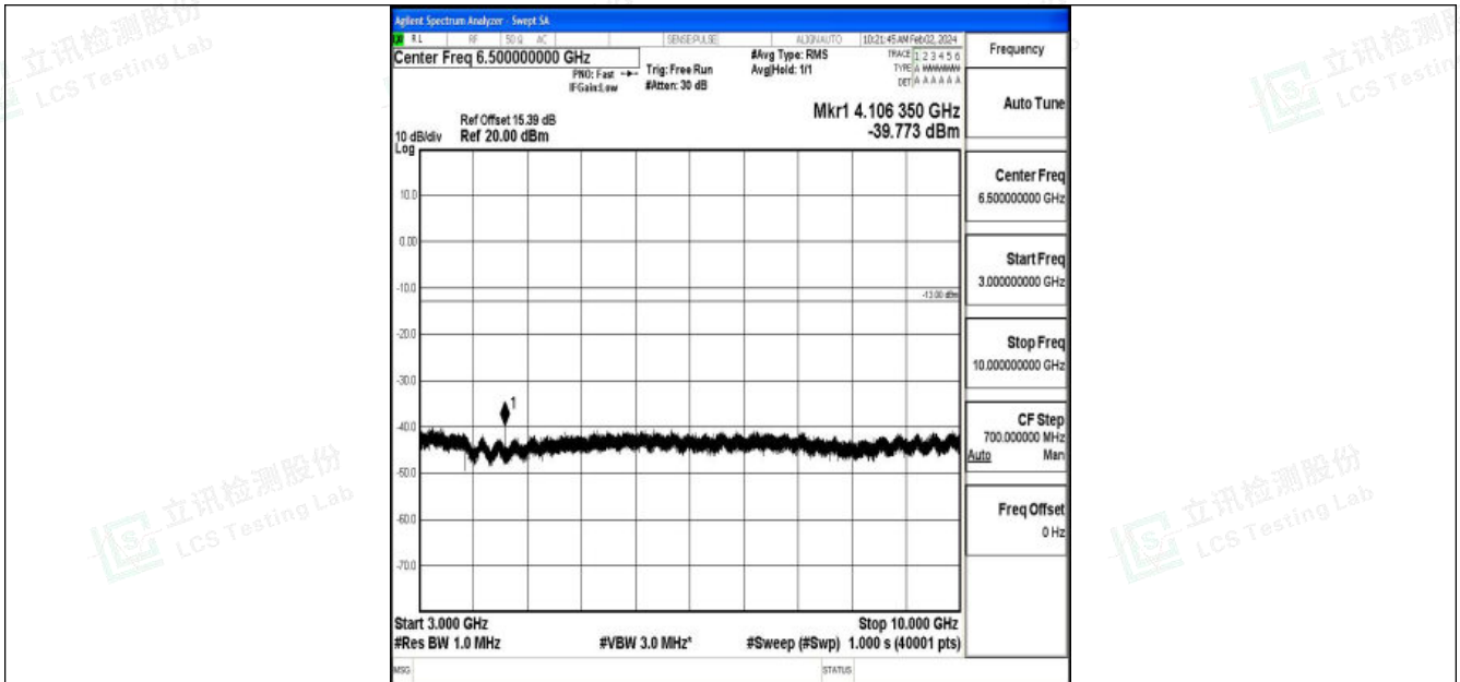
Band26_3MHz_QPSK_26775_1RB#0_3000~10000_3000~10000
