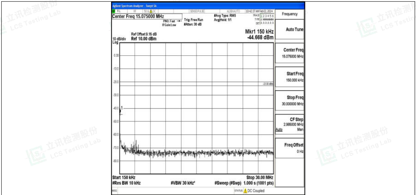
Band26_5MHz_16QAM_26765_1RB#0_0.15~30_0.15~30
