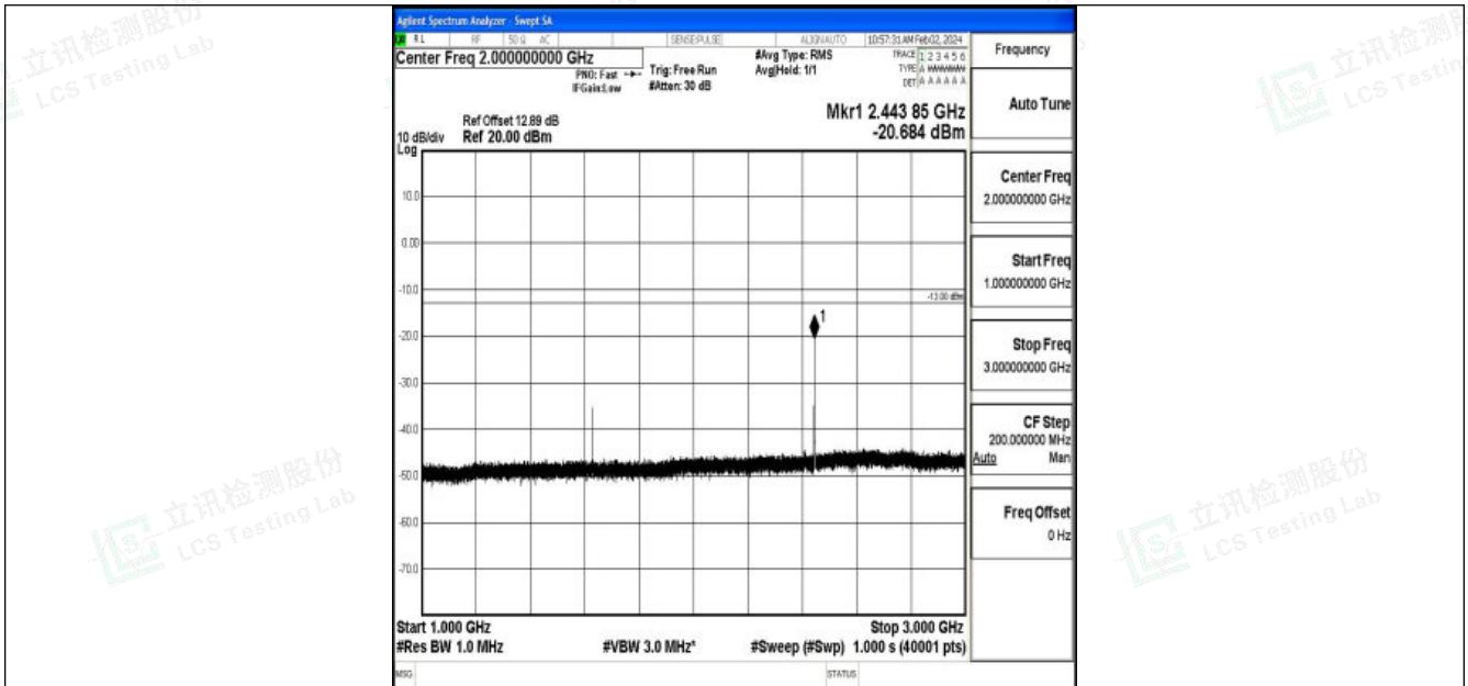
Band26_10MHz_16QAM_26740_1RB#0_1000~3000_1000~3000
