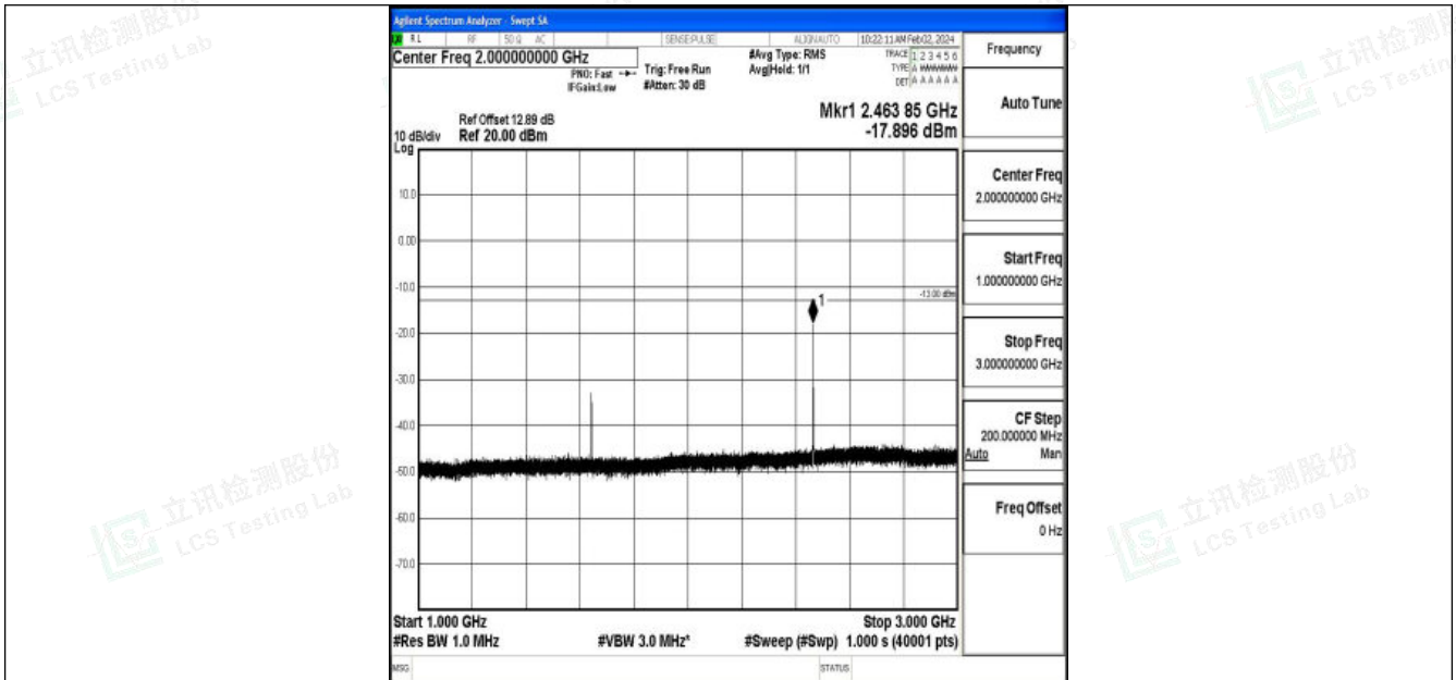
Band26_3MHz_16QAM_26775_1RB#0_1000~3000_1000~3000
