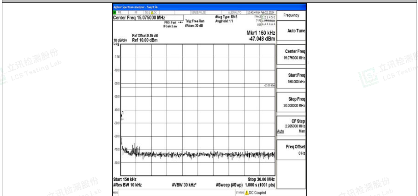
Band26_5MHz_QPSK_26740_1RB#0_0.15~30_0.15~30
