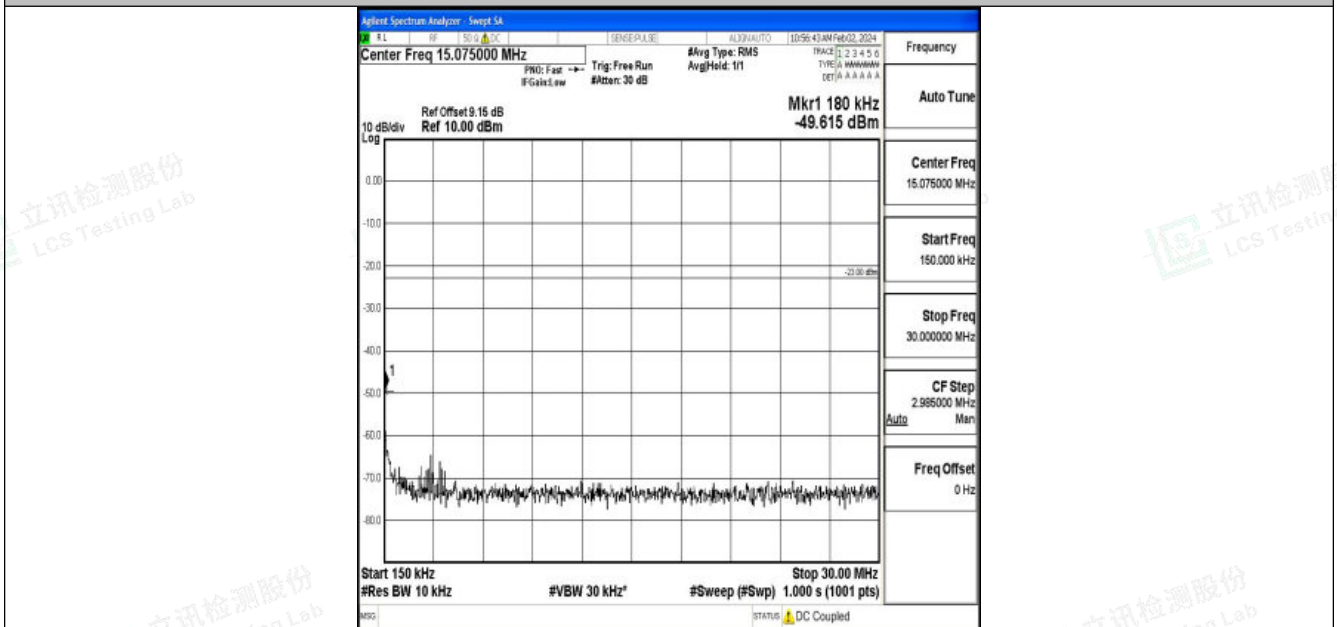
Band26_10MHz_QPSK_26740_1RB#0_0.15~30_0.15~30
