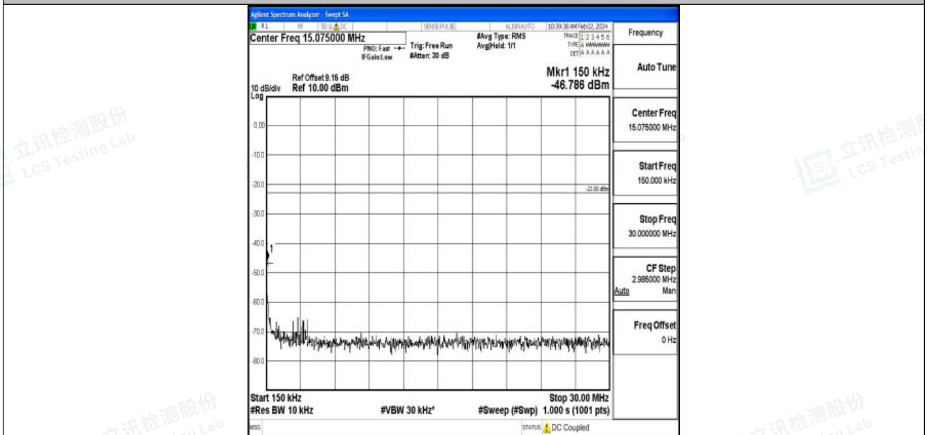
Band26_5MHz_QPSK_26715_1RB#0_0.15~30_0.15~30
