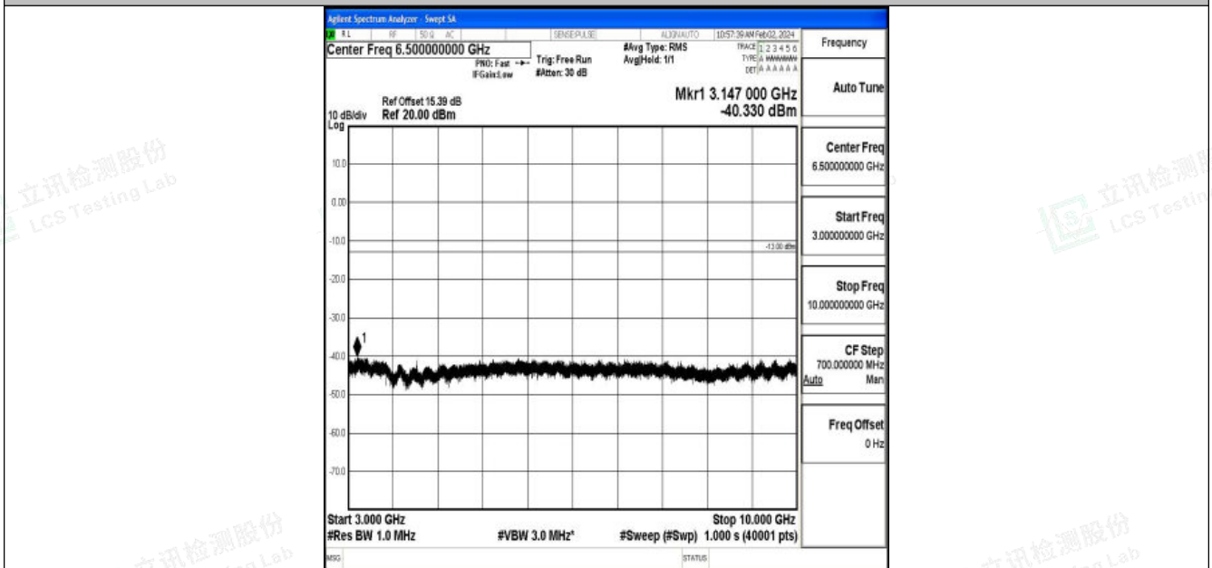
Band26_10MHz_16QAM_26740_1RB#0_3000~10000_3000~10000
