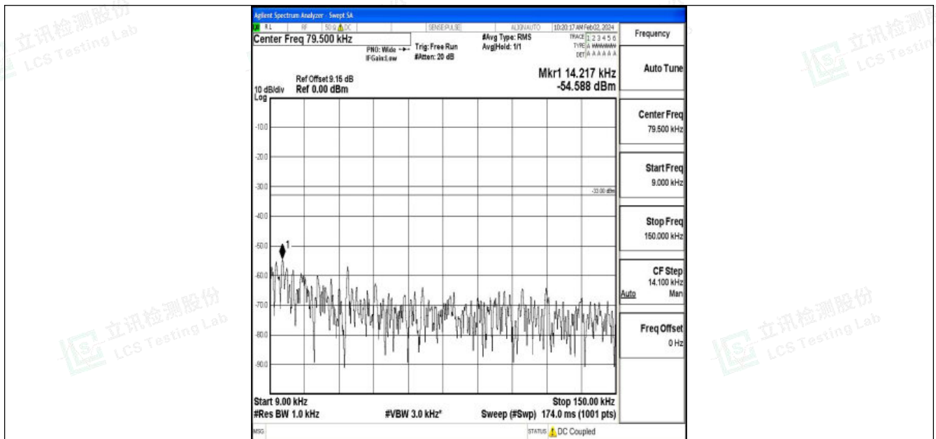
Band26_3MHz_QPSK_26740_1RB#0_0.009~0.15_0.009~0.15
