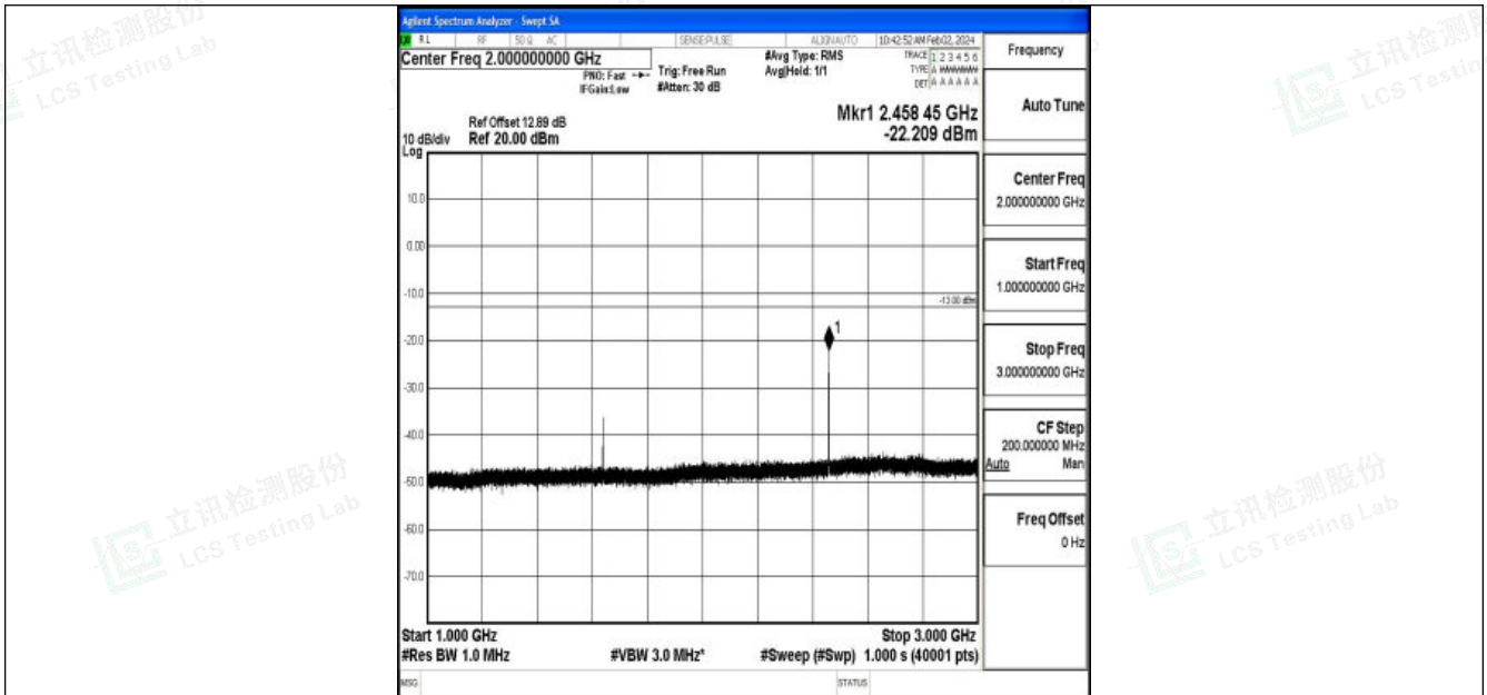
Band26_5MHz_16QAM_26765_1RB#0_1000~3000_1000~3000
