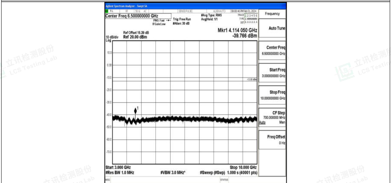
Band26_1.4MHz_16QAM_26783_1RB#0_3000~10000_3000~10000
