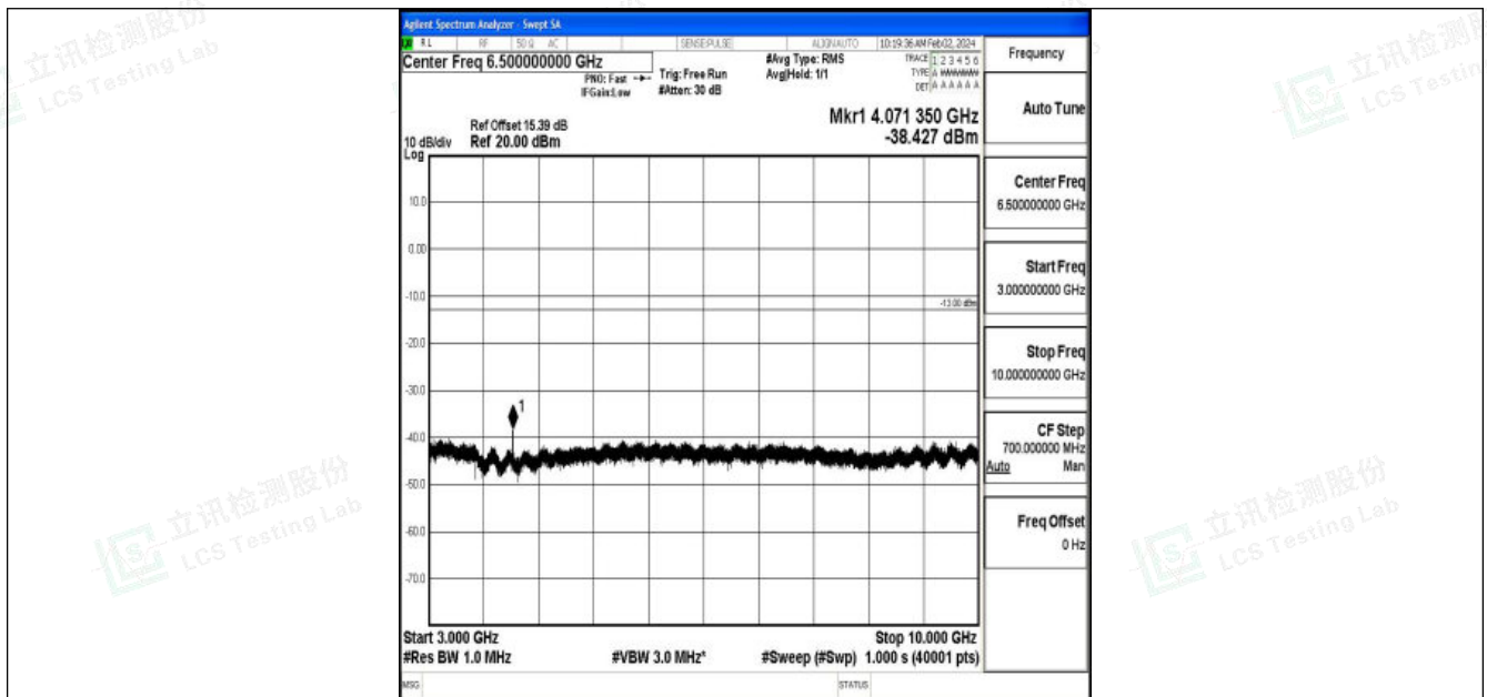
Band26_3MHz_QPSK_26705_1RB#0_3000~10000_3000~10000
