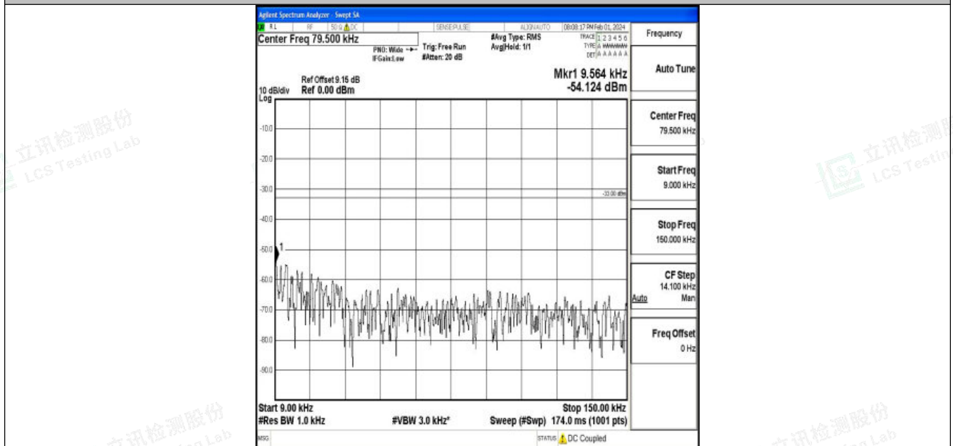
Band26_1.4MHz_16QAM_26783_1RB#0_0.009~0.15_0.009~0.15
