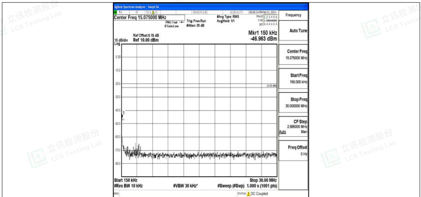
Band26_1.4MHz_16QAM_26783_1RB#0_0.15~30_0.15~30
