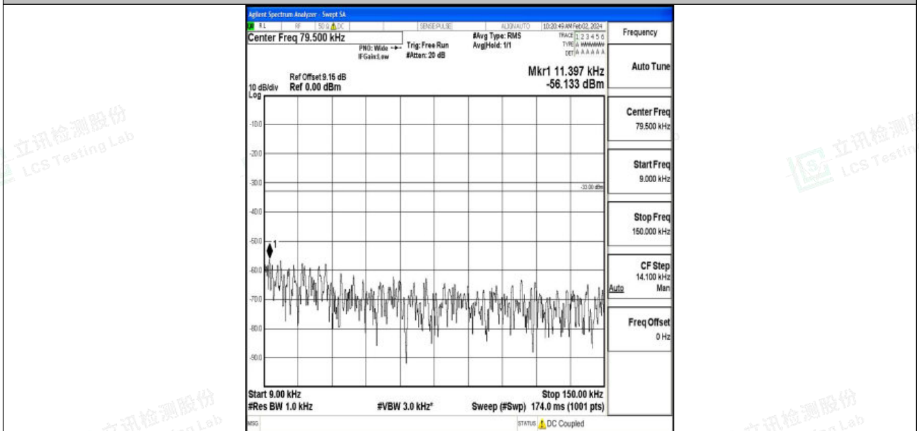
Band26_3MHz_16QAM_26740_1RB#0_0.009~0.15_0.009~0.15
