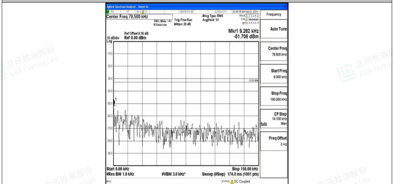
Band26_5MHz_16QAM_26715_1RB#0_0.009~0.15_0.009~0.15
