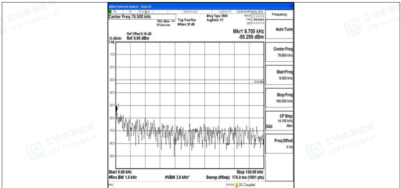
Band26_5MHz_QPSK_26740_1RB#0_0.009~0.15_0.009~0.15
