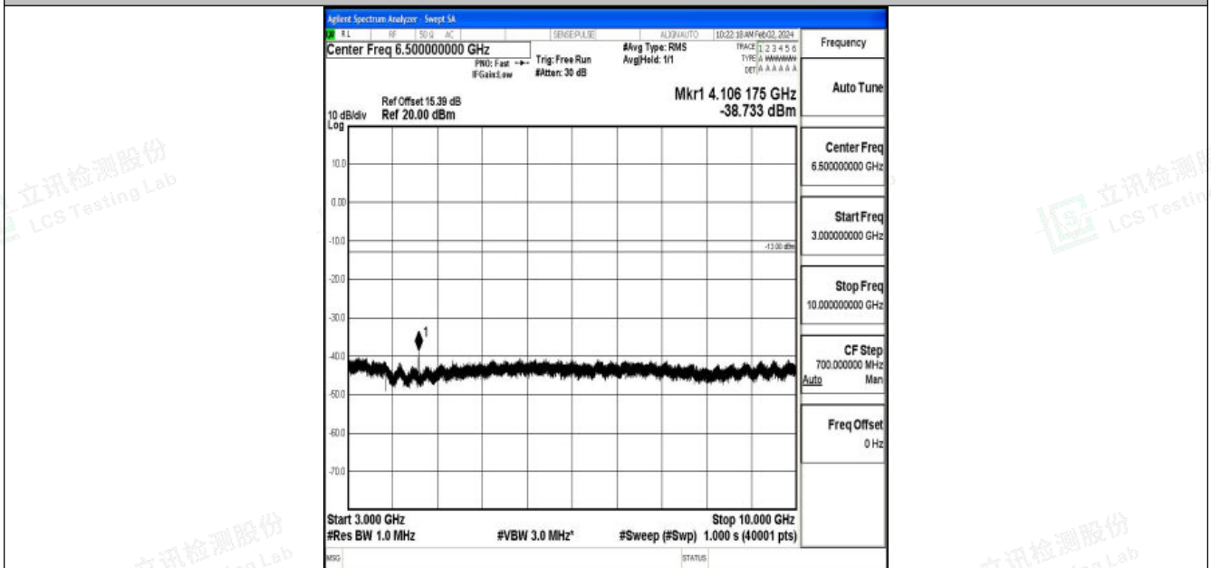
Band26_3MHz_16QAM_26775_1RB#0_3000~10000_3000~10000
