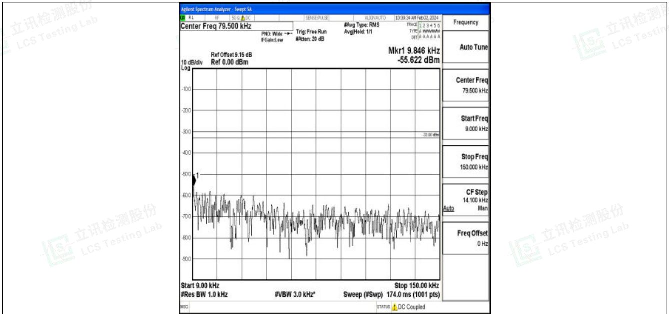
Band26_5MHz_QPSK_26715_1RB#0_0.009~0.15_0.009~0.15
