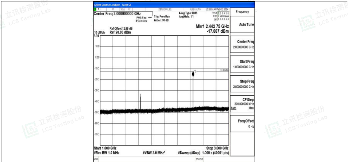
Band26_3MHz_16QAM_26705_1RB#0_1000~3000_1000~3000
