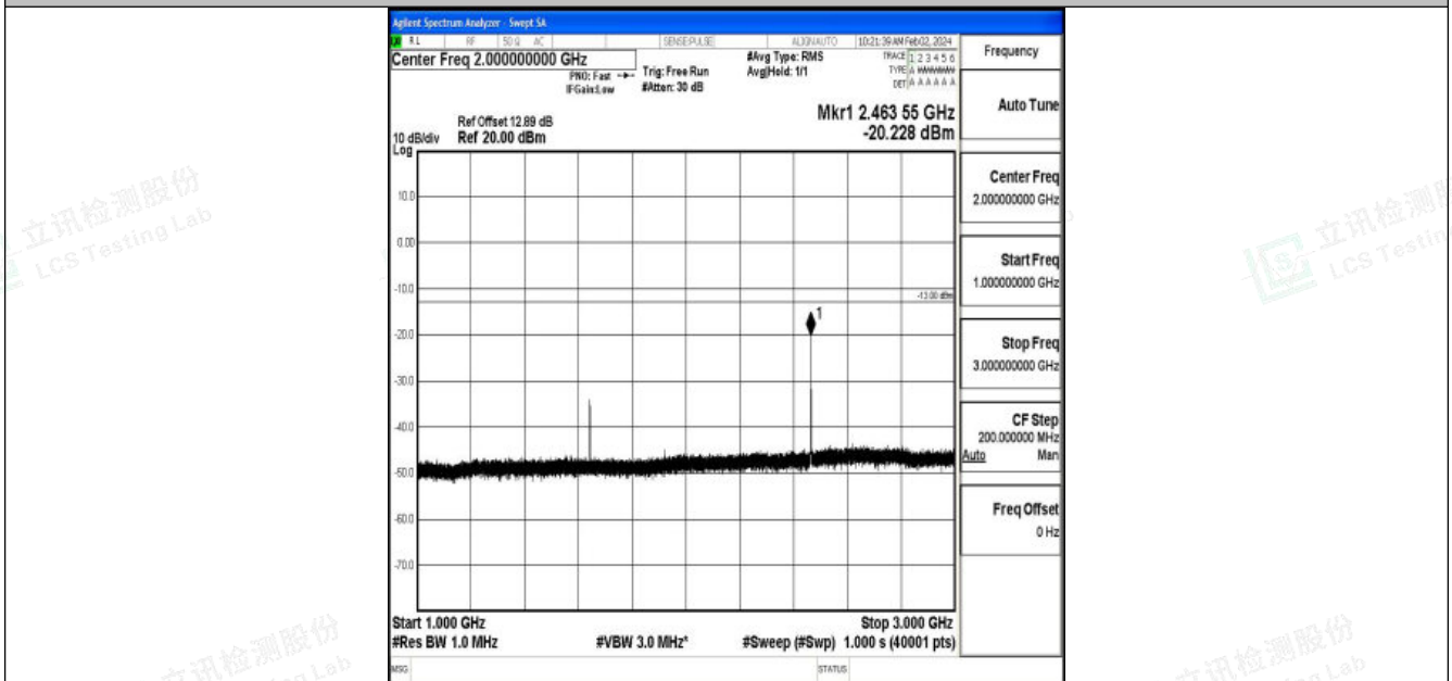
Band26_3MHz_QPSK_26775_1RB#0_1000~3000_1000~3000
