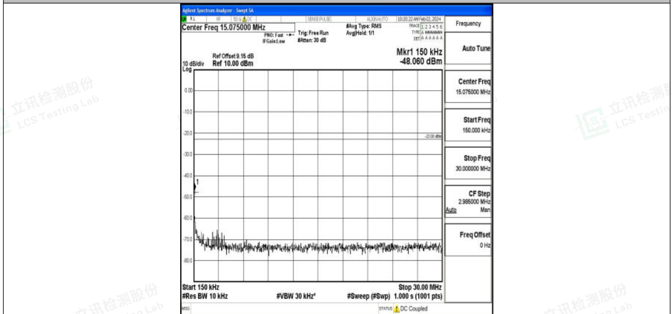
Band26_3MHz_QPSK_26740_1RB#0_0.15~30_0.15~30
