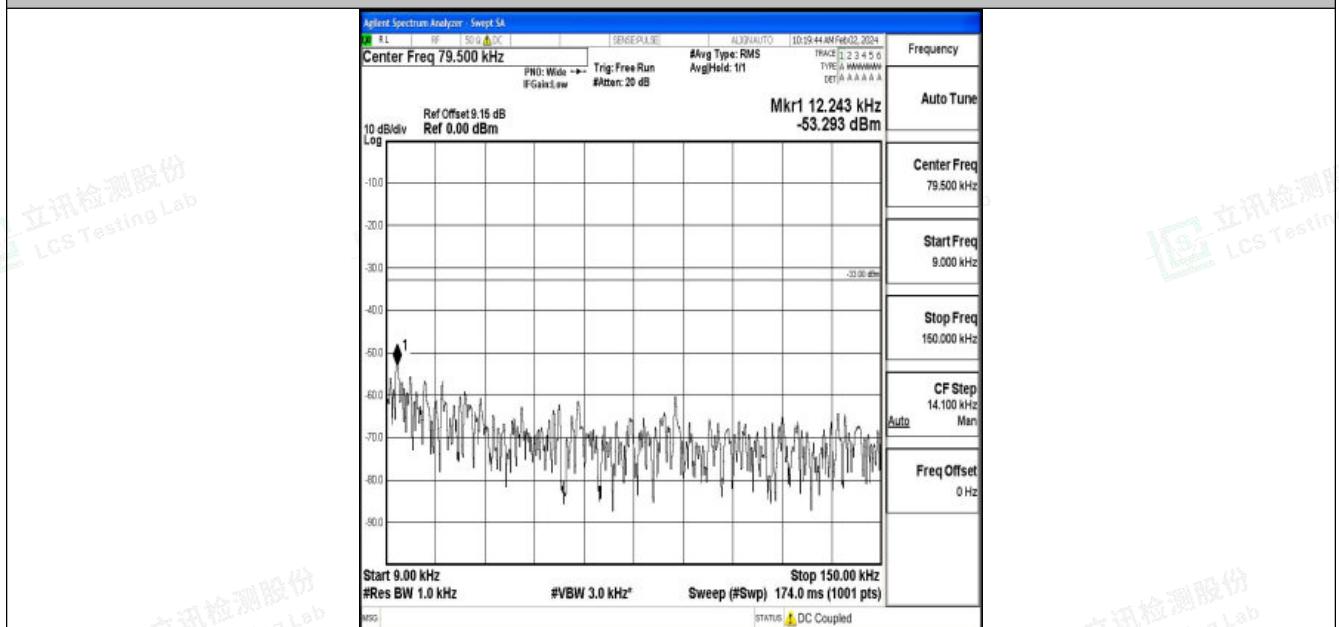
Band26_3MHz_16QAM_26705_1RB#0_0.009~0.15_0.009~0.15
