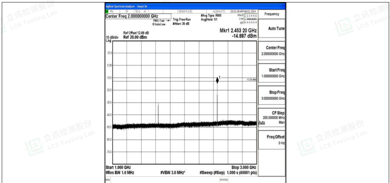
Band26_3MHz_16QAM_26740_1RB#0_1000~3000_1000~3000
