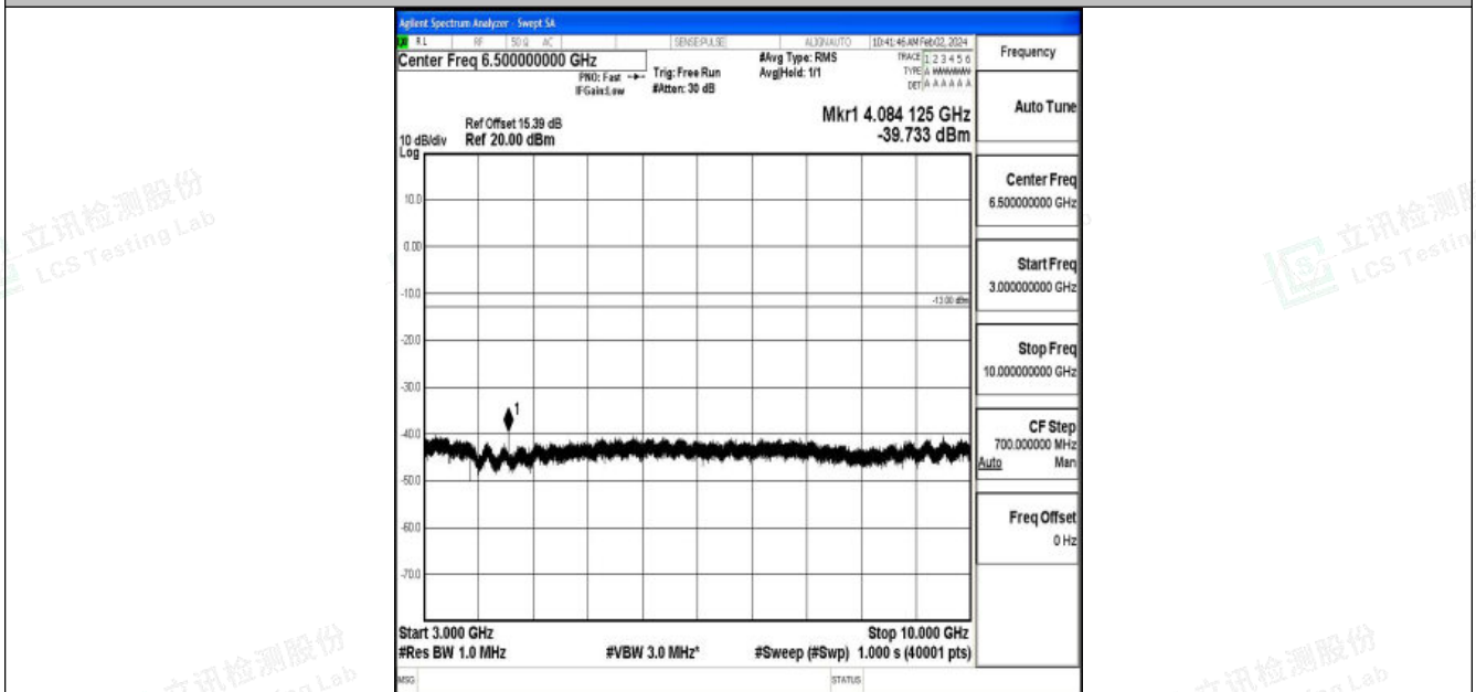
Band26_5MHz_16QAM_26740_1RB#0_3000~10000_3000~10000
