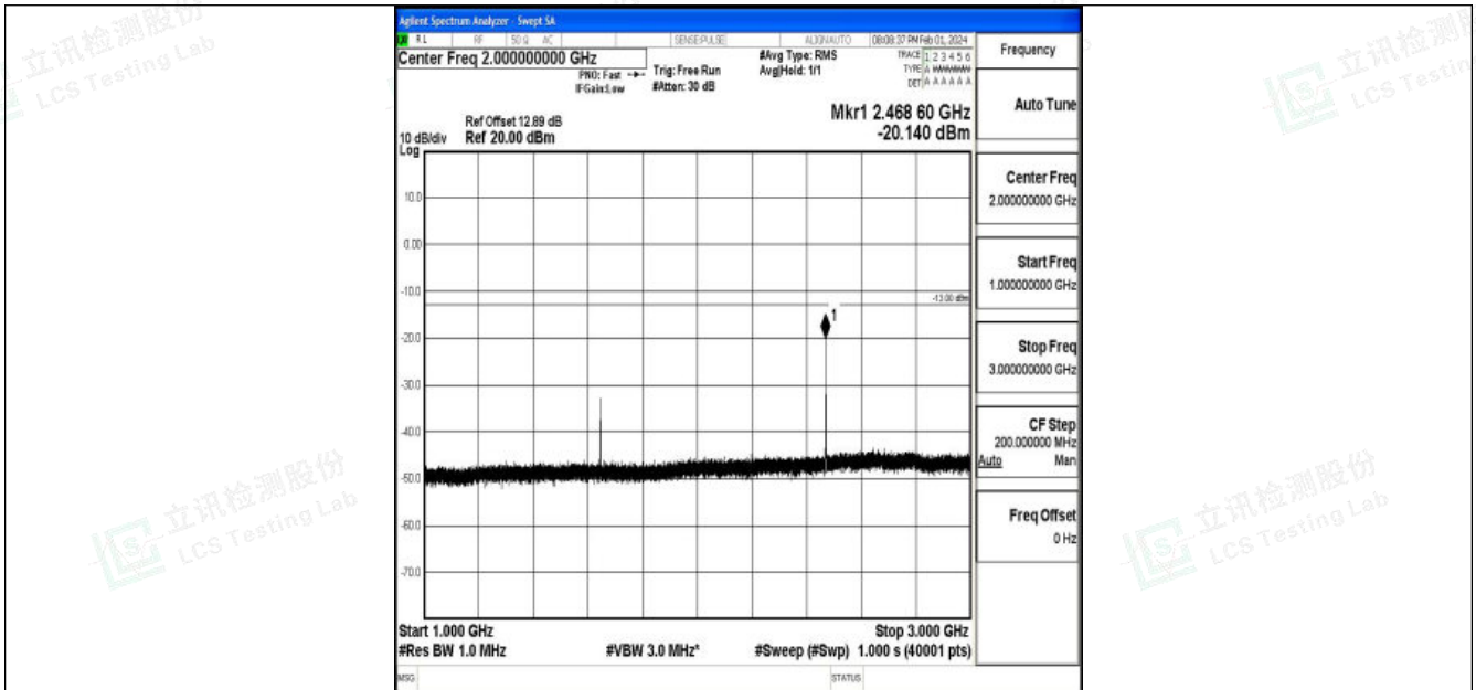
Band26_1.4MHz_16QAM_26783_1RB#0_1000~3000_1000~3000
