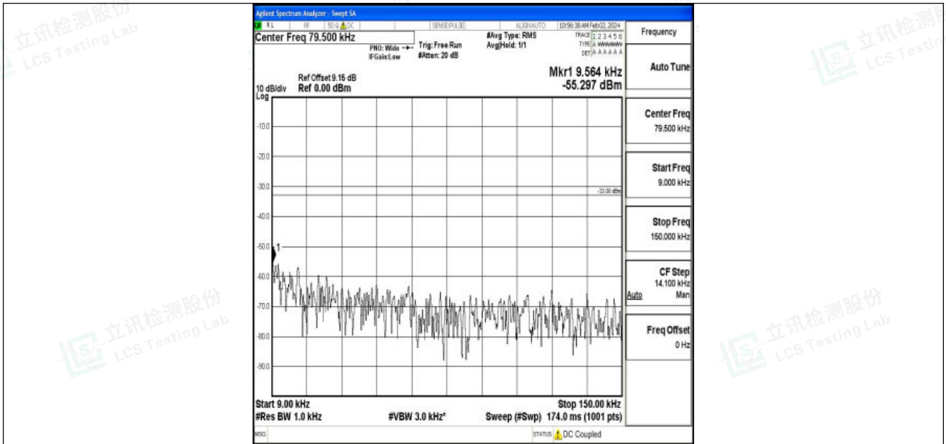
Band26_10MHz_QPSK_26740_1RB#0_0.009~0.15_0.009~0.15
