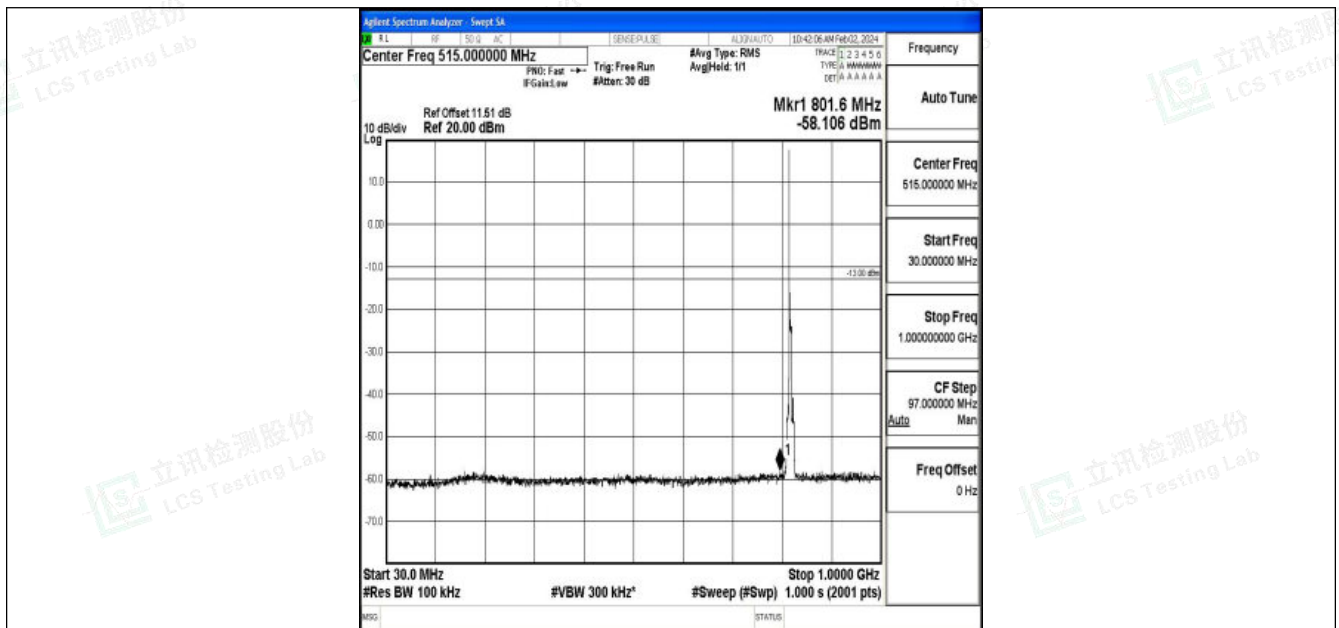
Band26_5MHz_QPSK_26765_1RB#0_30~1000_30~1000
