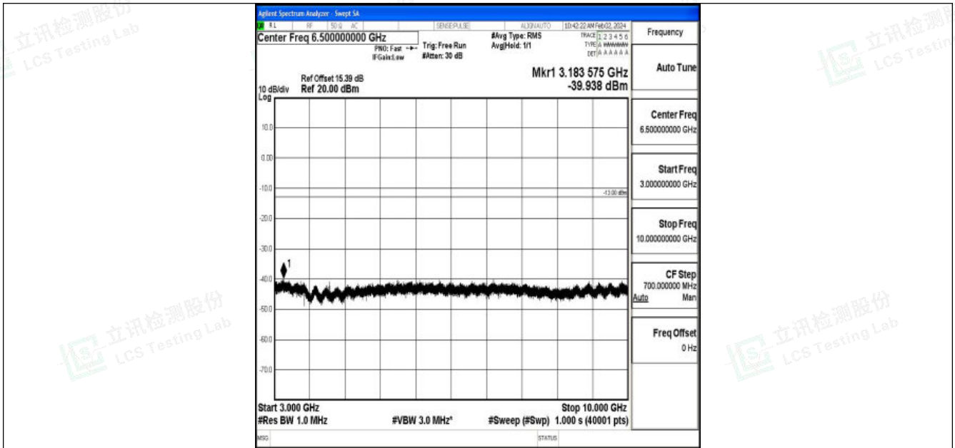
Band26_5MHz_QPSK_26765_1RB#0_3000~10000_3000~10000
