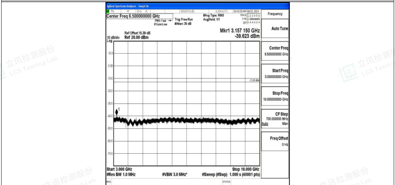
Band26_5MHz_16QAM_26765_1RB#0_3000~10000_3000~10000
