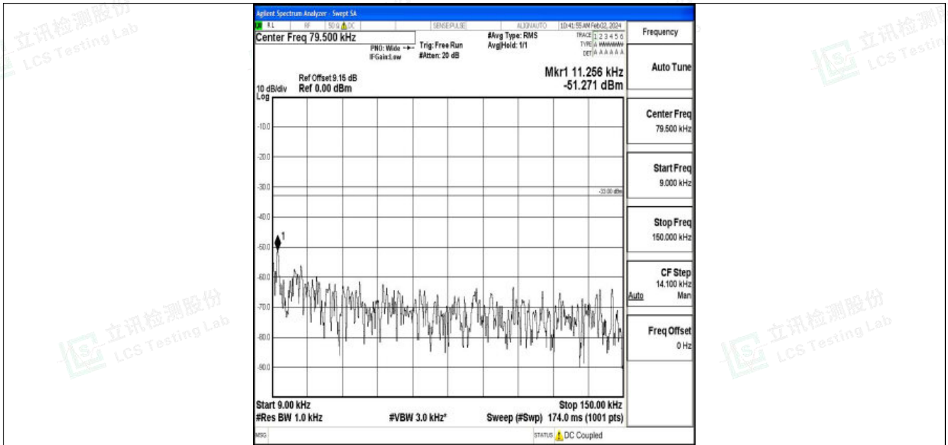
Band26_5MHz_QPSK_26765_1RB#0_0.009~0.15_0.009~0.15
