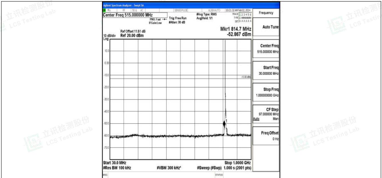
Band26_3MHz_QPSK_26775_1RB#0_30~1000_30~1000
