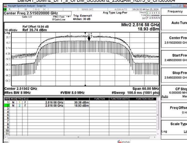
Band41 30MHz DFT s OFDM SCS30kHz 256QAM RB75_0 CH503004
