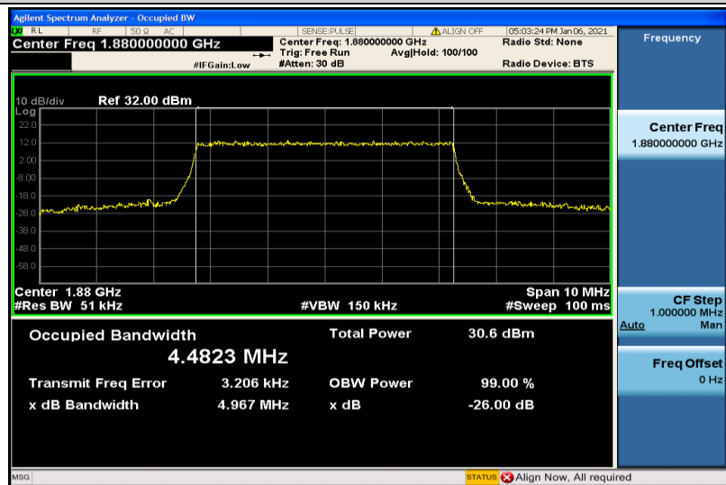
Band2-5MHz-16QAM-18900-25RB#0-4.4823
