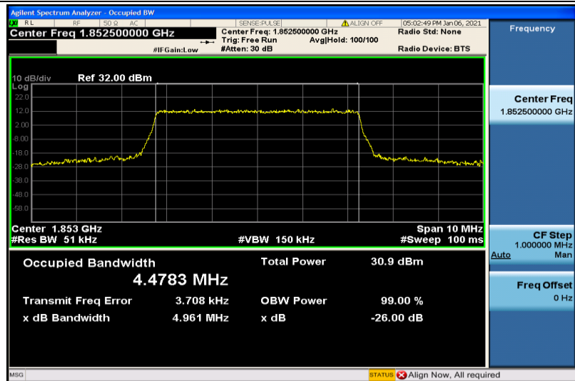
Band2-5MHz-16QAM-18625-25RB#0-4.4783
