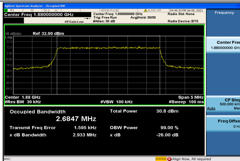
Band2-3MHz-QPSK-18900-15RB#0-2.6847
