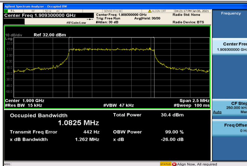
Band2-1.4MHz-QPSK-19193-6RB#0-1.0825
