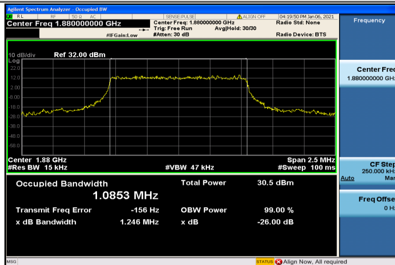
Band2-1.4MHz-QPSK-18900-6RB#0-1.0853
