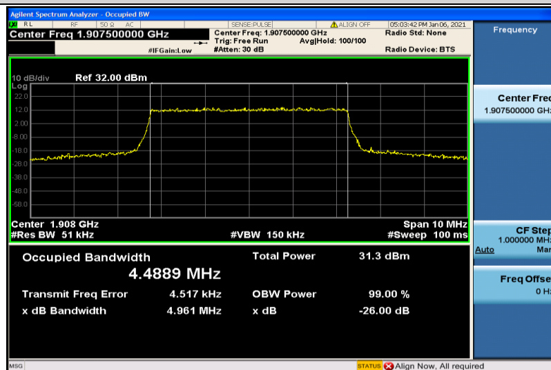
Band2-5MHz-QPSK-19175-25RB#0-4.4889
