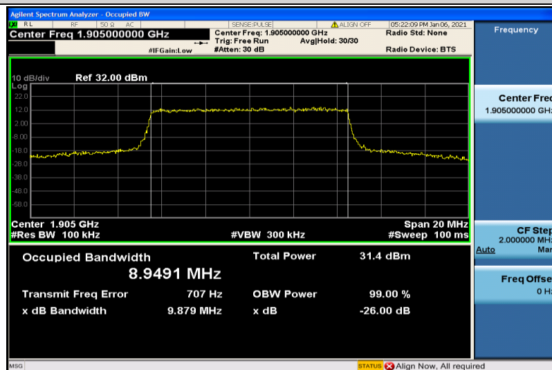
Band2-10MHz-QPSK-19150-50RB#0-8.9491
