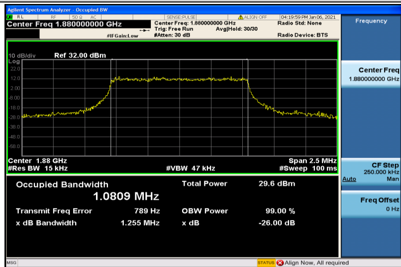
Band2-1.4MHz-16QAM-18900-6RB#0-1.0809
