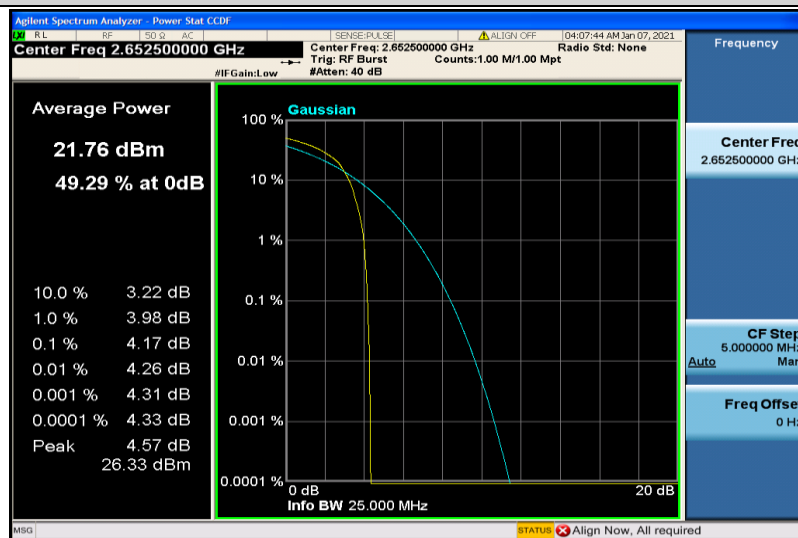
Band41-5MHz-16QAM-41215-1RB#0
