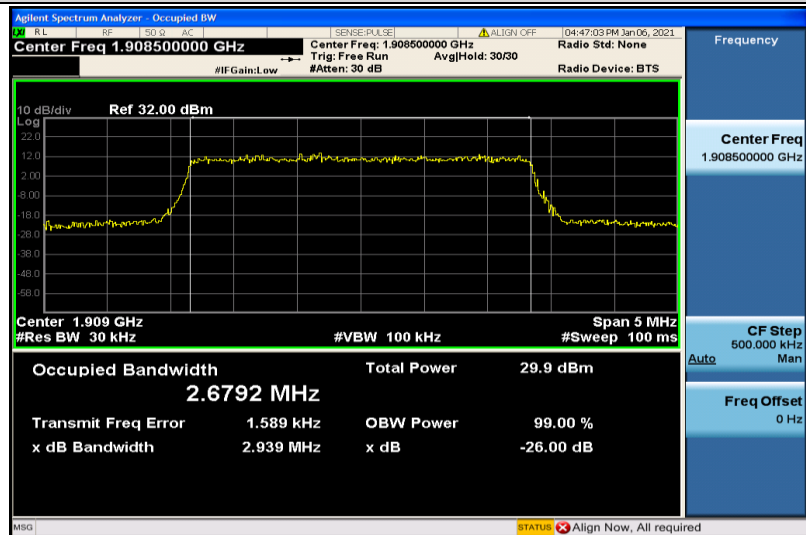
Band2-3MHz-16QAM-19185-15RB#0-2.6792
