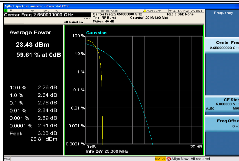
Band41-10MHz-QPSK-41190-1RB#0
