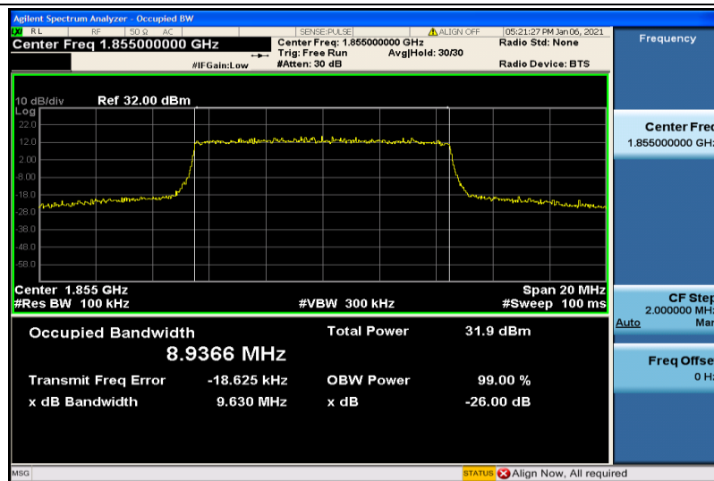
Band2-10MHz-QPSK-18650-50RB#0-8.9366
