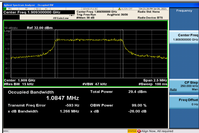
Band2-1.4MHz-16QAM-19193-6RB#0-1.0847
