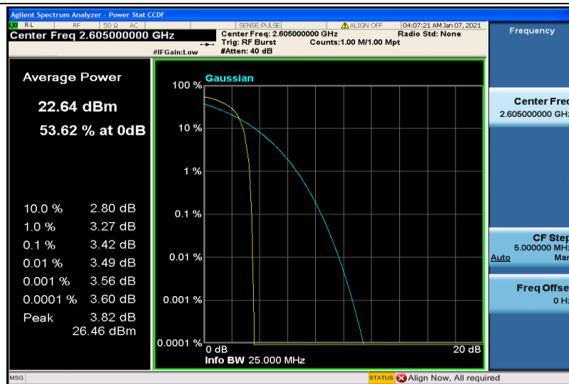
Band41-5MHz-16QAM-40740-1RB#0
