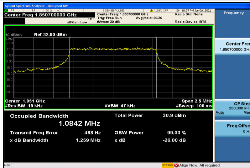
Band2-1.4MHz-QPSK-18607-6RB#0-1.0842
