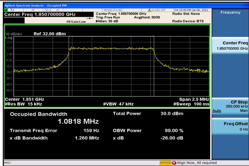
Band2-1.4MHz-16QAM-18607-6RB#0-1.0818
