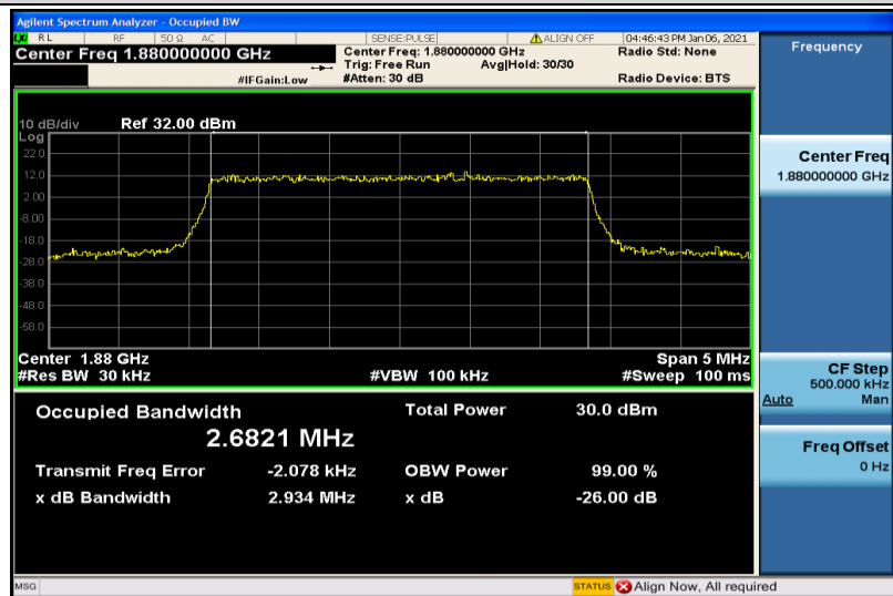
Band2-3MHz-16QAM-18900-15RB#0-2.6821
