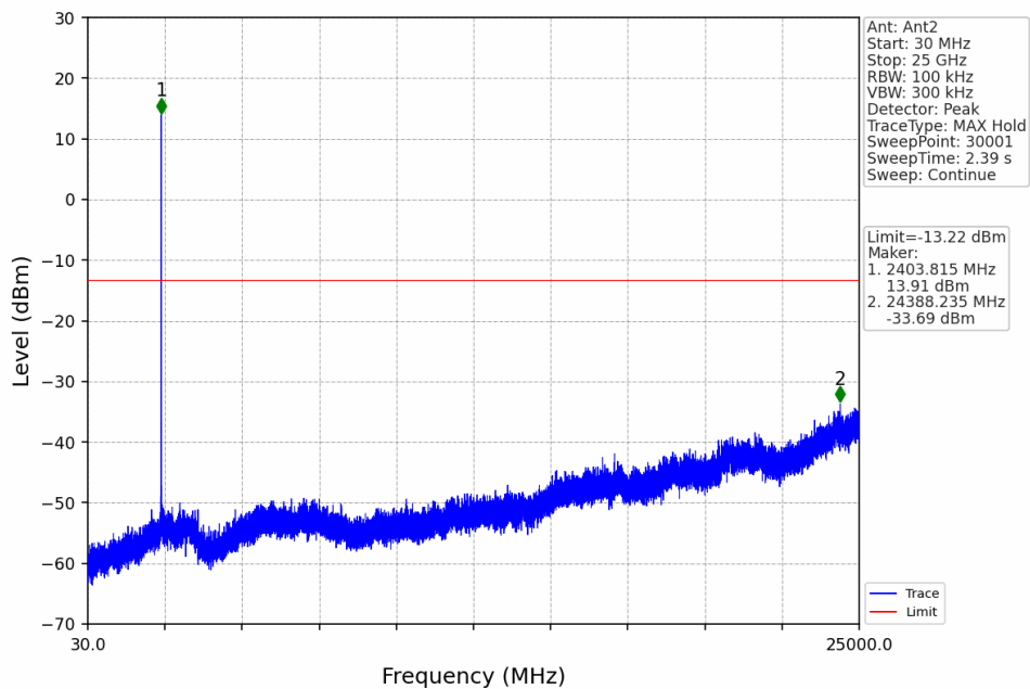
1.4M_LCH_2403.5MHz_Ant2_NTNV
