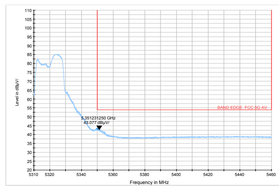
802.11a-Channel 64: Average
