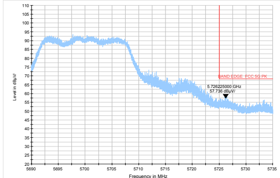
802.11a-Channel 140: Peak
