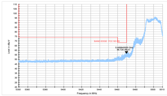
802.11a-Channel 100: Average
