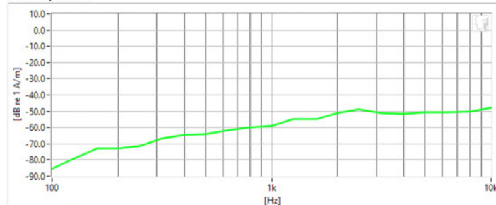
Frequency Response
