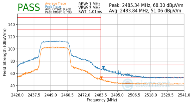
Plot 7-175. Radiated Restricted Upper Band Edge Measurement Ant 2 (Peak & Average – RU242)
