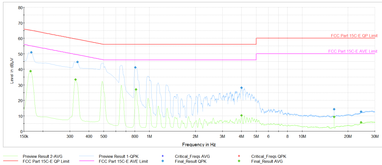
Plot 7-196. AC Line Conducted Emissions with 802.11ax (RU26) Ch.6 (L1, with AC/DC Adapter)
