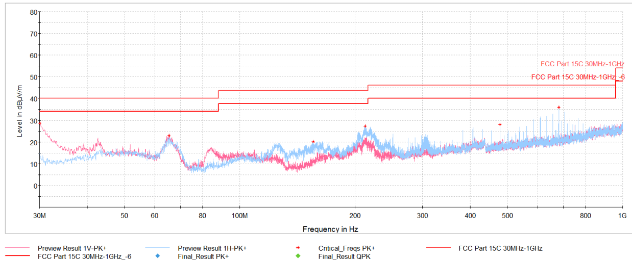
Plot 7-194. Radiated Spurious Emissions below 1GHz CDD Ch.6 (RU26), with AC/DC Adapter
