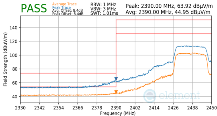
Plot 7-171. Radiated Restricted Lower Band Edge Measurement Ant 2 (Peak & Average – RU242)
