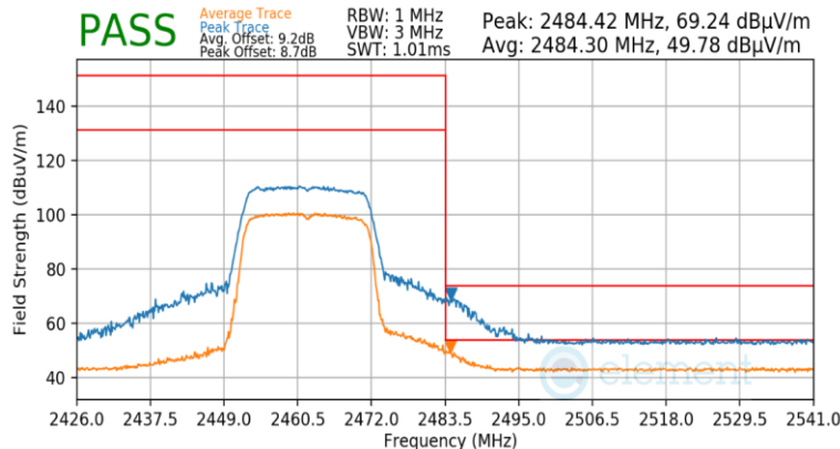
Plot 7-177. Radiated Restricted Upper Band Edge Measurement Ant 2 (Peak & Average – RU242)
