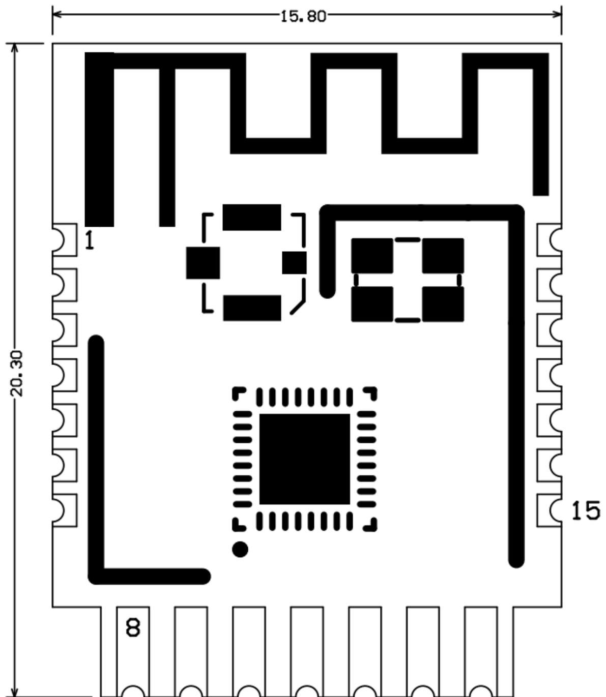
Top View
