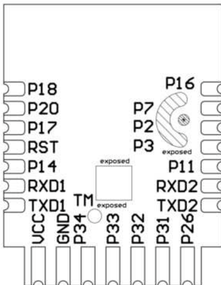
Bottom View
