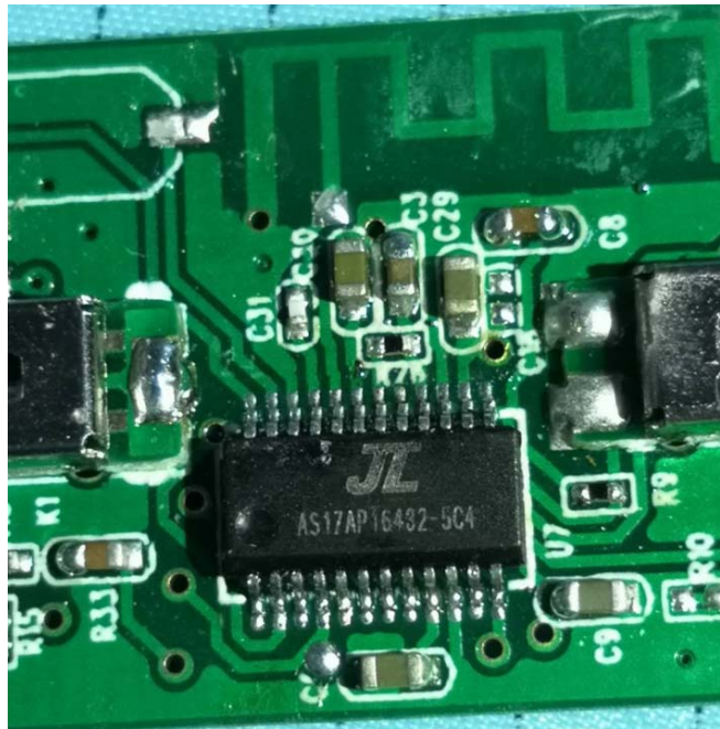
EUT – Main Chip 1 View
