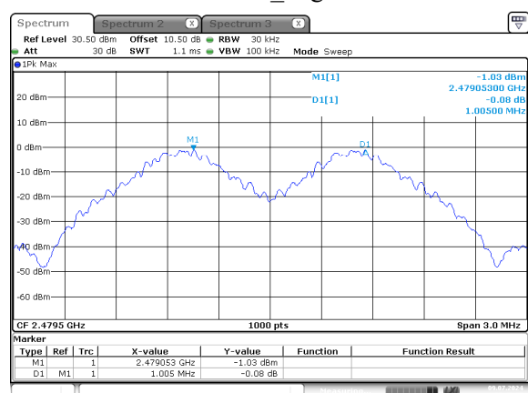
GFSK_High
