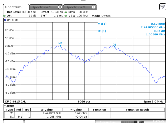
GFSK_Middle
