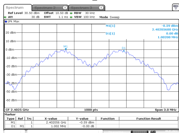
GFSK_Low
