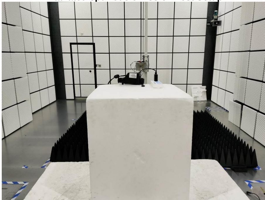
Radiated spurious emission Test Setup
