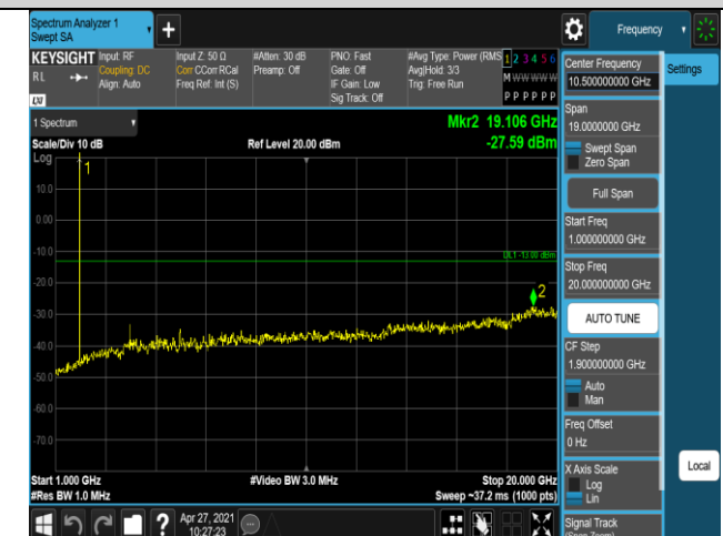
Band2-1.4MHz-QPSK-19193-1RB#0-Range2:1000~20
