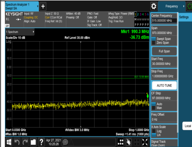
Band2-1.4MHz-QPSK-18900-1RB#0-Range1:30~10
