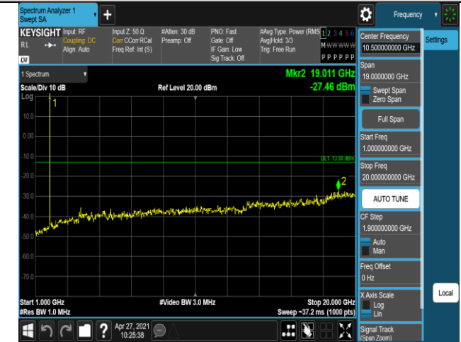
Band2-1.4MHz-QPSK-18900-1RB#0-Range2:1000~20
