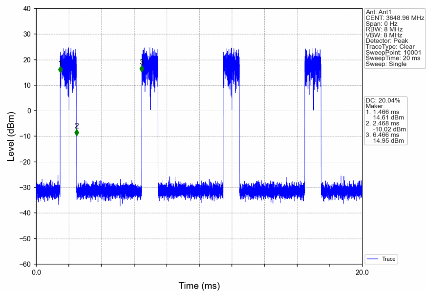
n78d_30kHz_SISO_NTNV_100MHz_CP-OFDM_QPSK_3600MHz_Edge_1RB_Right
