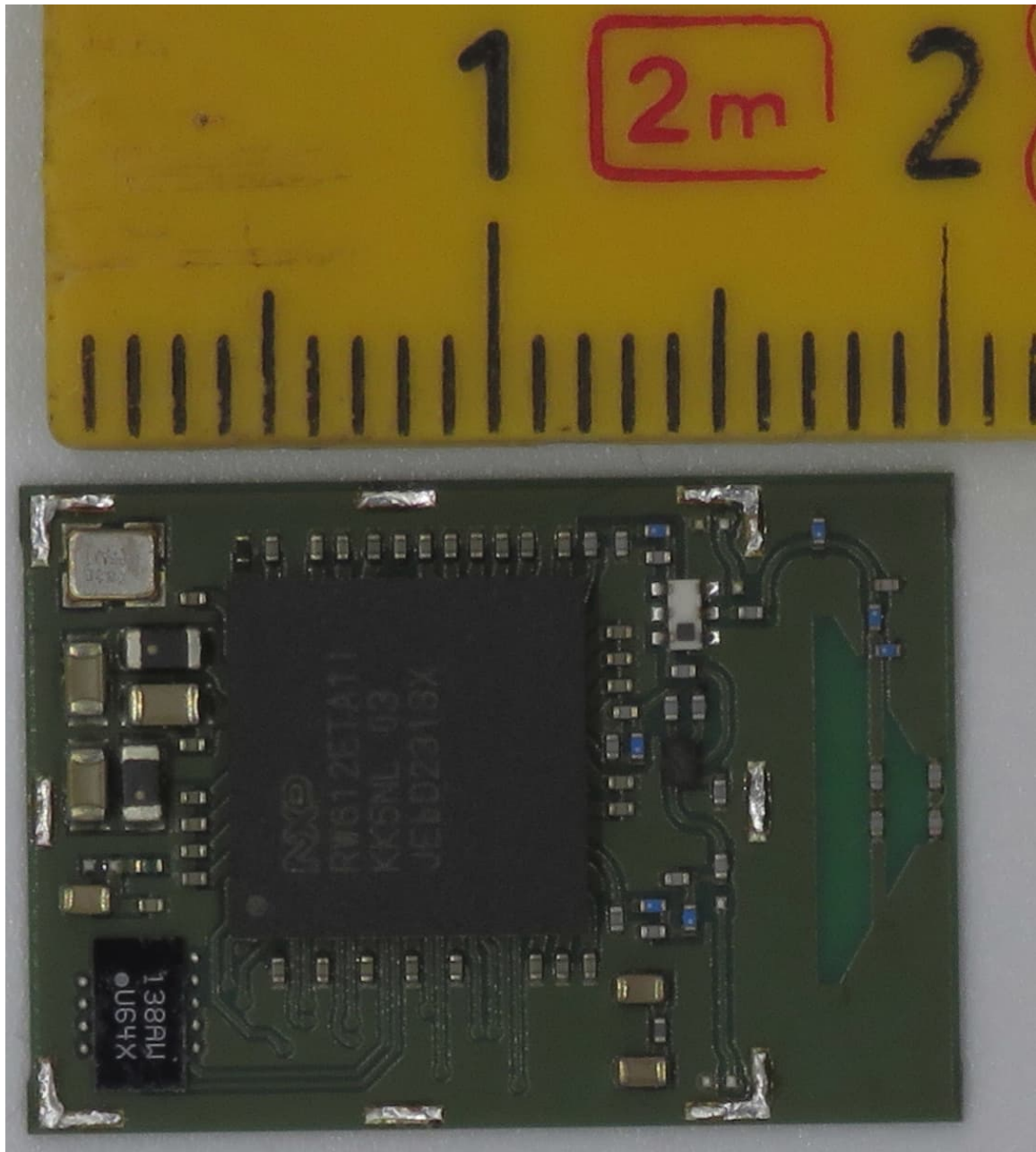
IRIS-W106-00B – shielding removed
