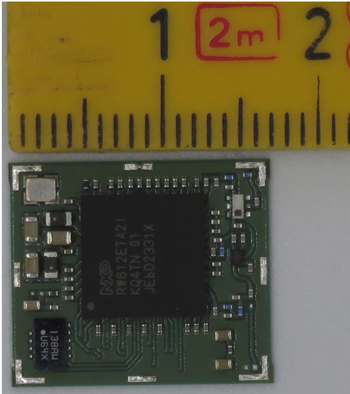
IRIS-W101-00B – shielding removed
