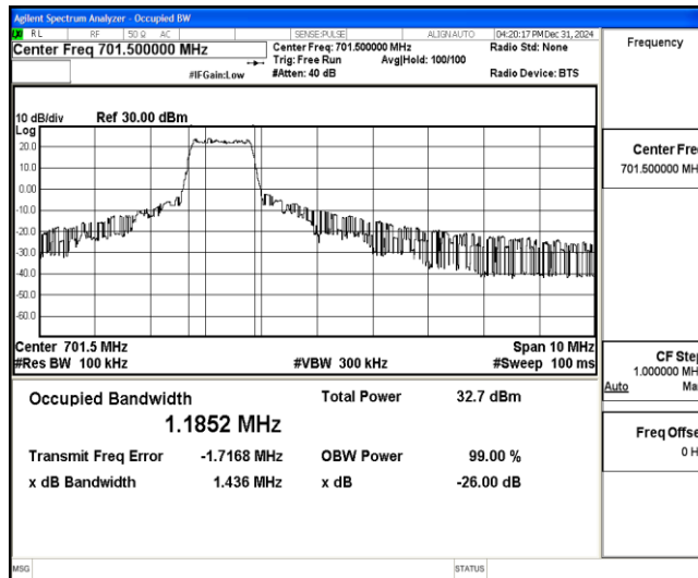
Band12-5MHz-QPSK-23035-6-0-Low-1.1852-1.436-PASS
