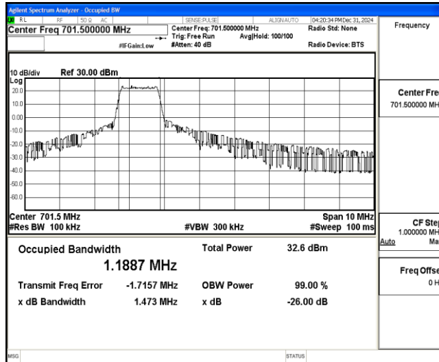
Band12-5MHz-16QAM-23035-6-0-Low-1.1887-1.473-PASS
