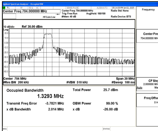
Band12-10MHz-QPSK-23060-6-0-Low-1.3293-2.014-PASS
