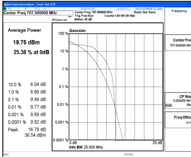
Band12-5MHz-16QAM-23095-6-0-Low-9.49-&lt;=13-PASS
