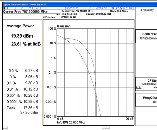
Band12-5MHz-QPSK-23095-6-0-Low-9.80-&lt;=13-PASS
