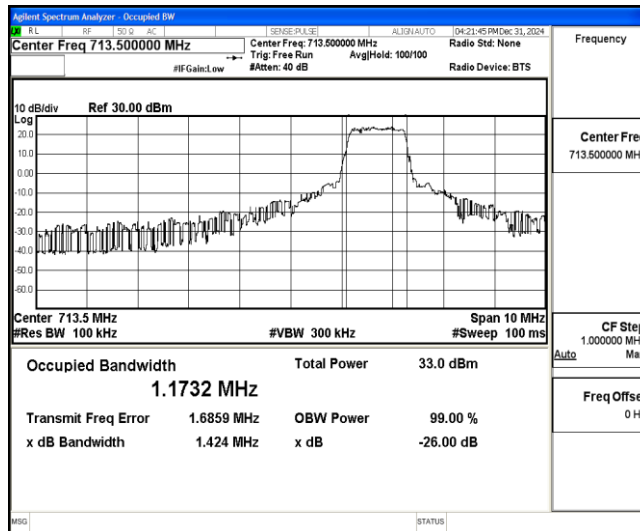
Band12-5MHz-16QAM-23155-6-0-High-1.1732-1.424-PASS
