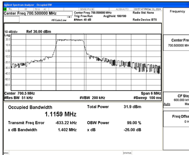
Band12-3MHz-16QAM-23025-6-0-Low-1.1159-1.402-PASS
