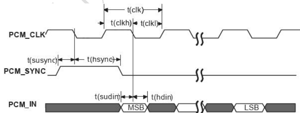
Figure 20: PCM_SYNC timing
