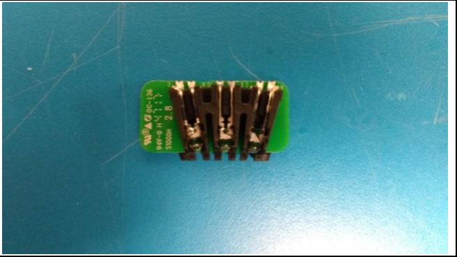
Ribbon Color Sensor Bottom View
