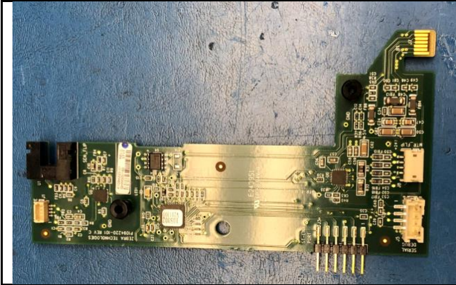
Feeder Board Top View
