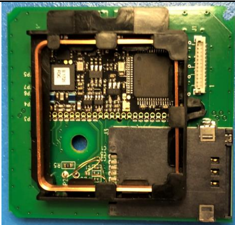
Smart Card Encoder Top View
