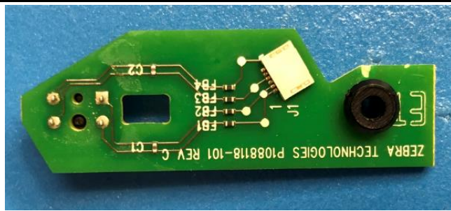
Head Can Sensor Board Top View
