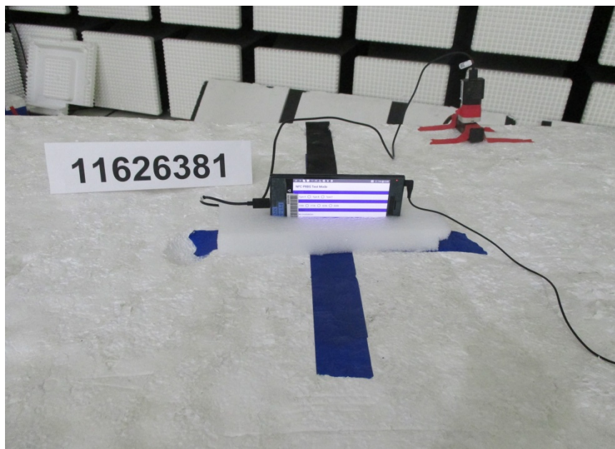
Y-AXIS ORIENTATION
