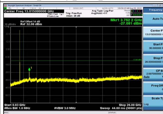
FDD02_MidRange_15MHz_30MHz~26GHz
