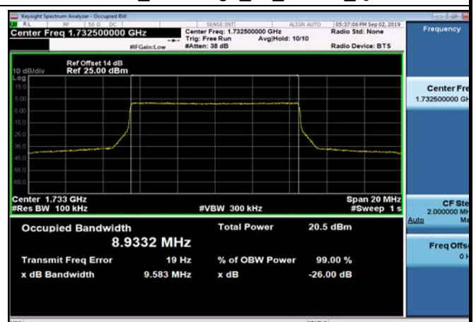
FDD04_MidRange_10_1732.5_Q16
