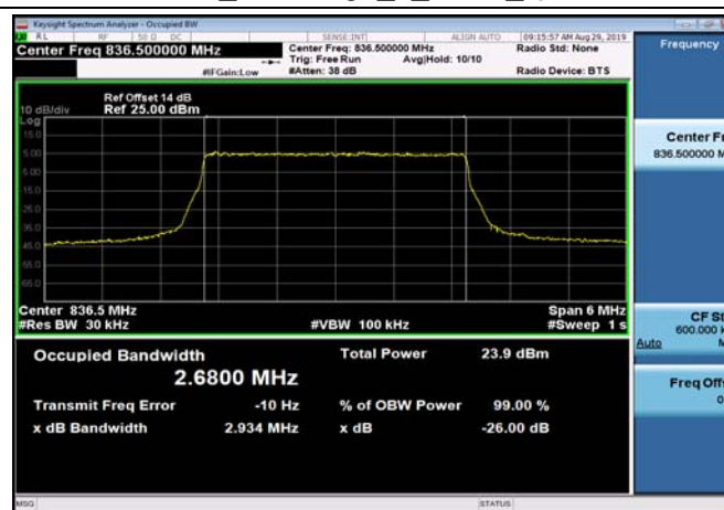
FDD05_MidRange_5_836.5_QPSK
