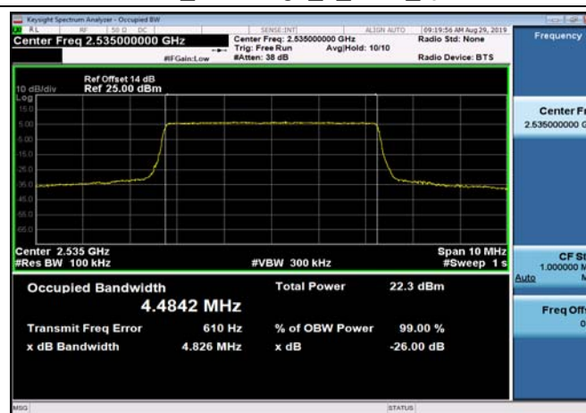
FDD07_MidRange_10_2535_QPSK
