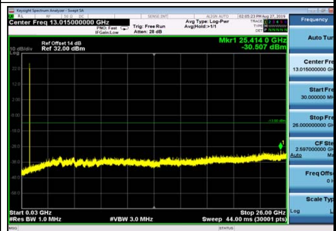
FDD07_HighRange_20MHz_30MHz~26GHz
