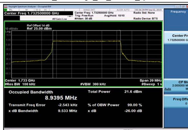
FDD04_MidRange_10_1732.5_QPSK
