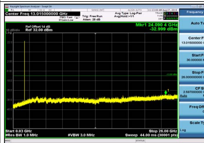
FDD02_MidRange_10MHz_30MHz~26GHz
