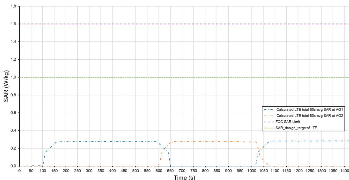
Total Time Averaged SAR for LTE Antenna Switching Spatial TAS Tech: LTE, Band 66, Antenna B / LTE, Band 25, Antenna F
