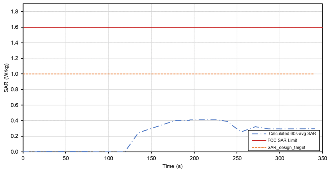
Total Time-Averaged SAR LTE ULCA Tech: LTE, Band 41, Ant B
