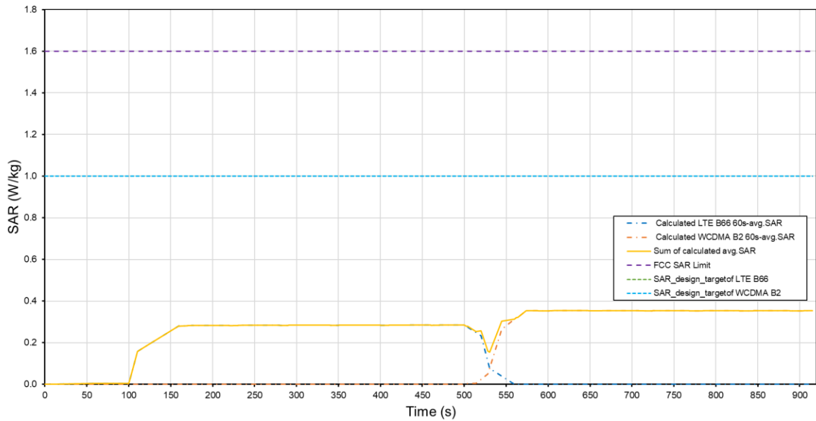
Total Time Averaged SAR for LTE to WCDMA IRAT Re-selection Tech: LTE, Band 66, Antenna B / WCDMA, Band 2, Antenna B
