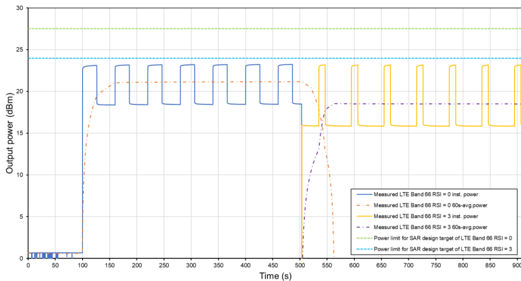
Conducted Tx Power for Change in Operating State Tech: LTE Band 66, Antenna B, RSI = 0 to RSI = 3
