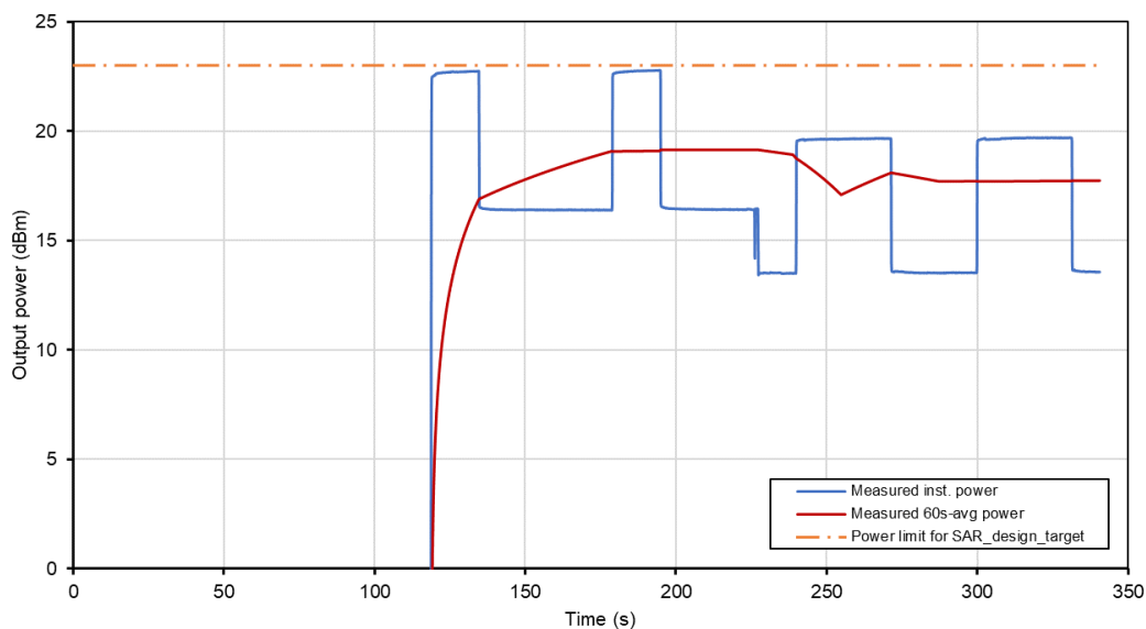
Time-Averaged Conducted Power LTE ULCA Tech: LTE, Band 41, Ant B
