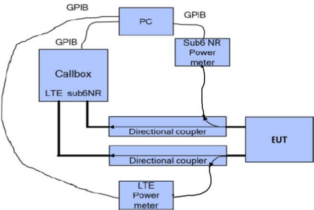
(c) Appendix A – Test Setup Photo 5, 9
