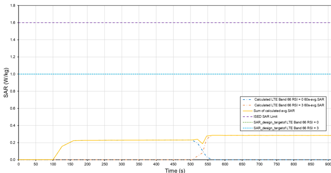
Total Time Averaged SAR for Change in Operating State Tech: LTE Band 66, Antenna B, RSI = 0 to RSI = 3
