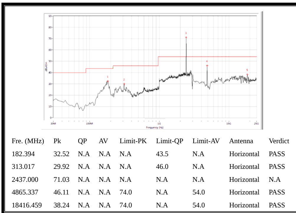
(Plot B.2: Antenna Horizontal, 30MHz to 25GHz)
