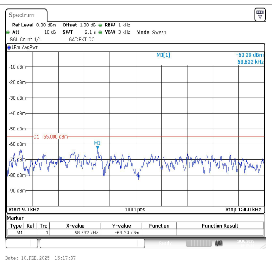
Band41_15MHz_16QAM_41515_1RB#0_0.009~0.15
