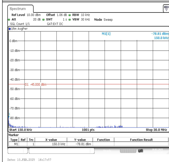
Band41_15MHz_16QAM_41515_1RB#0_0.15~3
