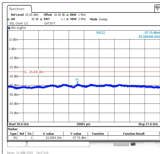
Band41_15MHz_QPSK_41515_1RB#0_20000~27000
