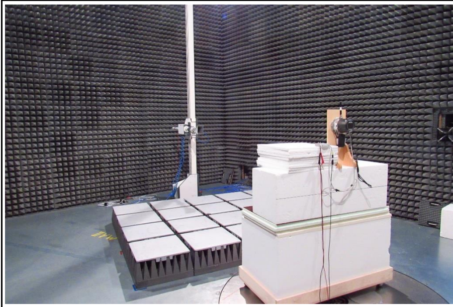
Setup 6.5 to 18 GHz EUT vertical
