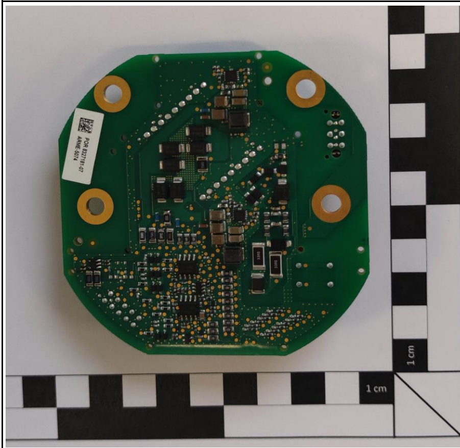
Main PCB bottom side view without casting compound
