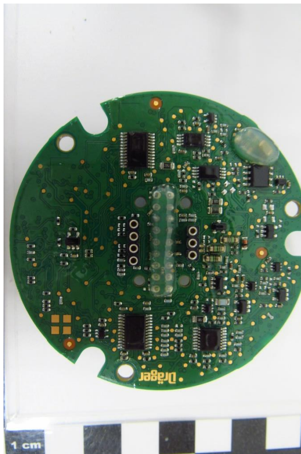
Sensor logic PCB bottom side view
