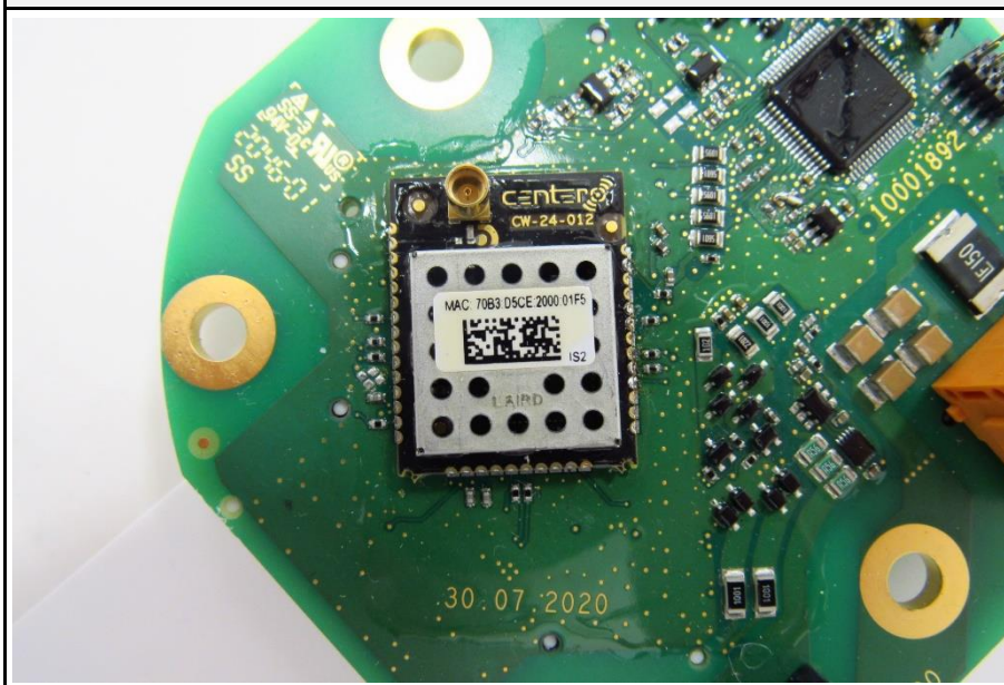
Zigbee radio
