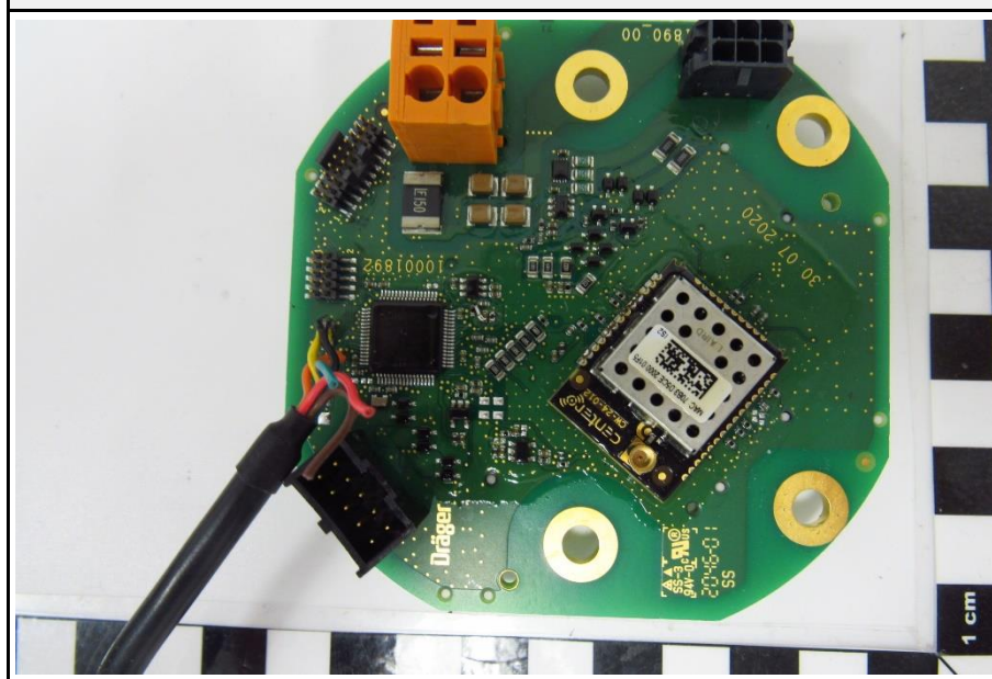
Main PCB top side view
