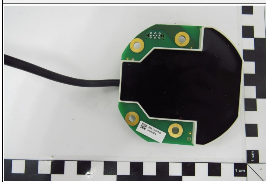
Main PCB bottom side view
