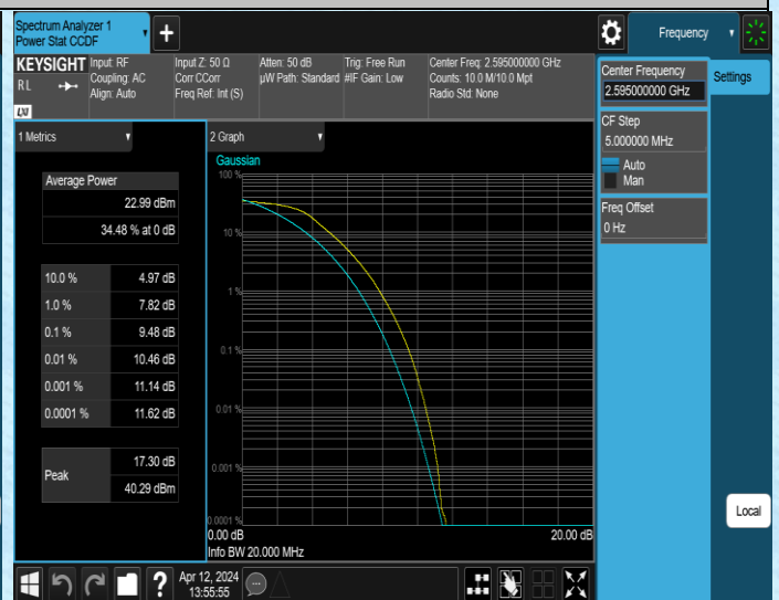
Band38-20MHz-QPSK-38000-100RB#0-PASS
