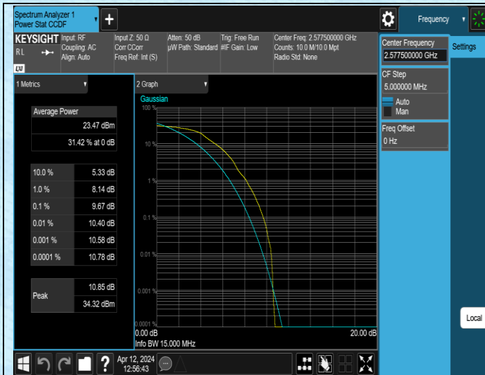
Band38-15MHz-QPSK-37825-1RB#0-PASS
