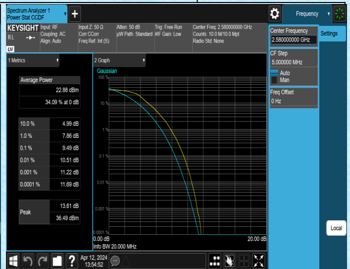
Band38-20MHz-QPSK-37850-100RB#0-PASS
