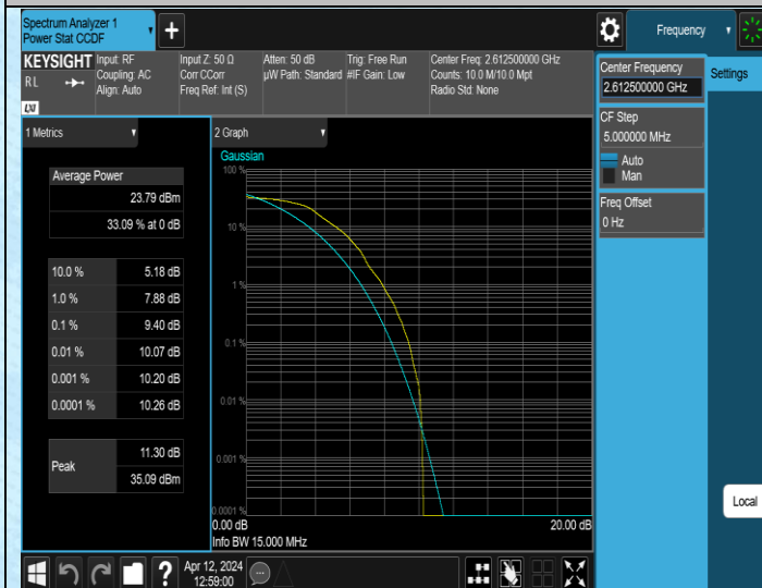
Band38-15MHz-QPSK-38175-1RB#0-PASS
