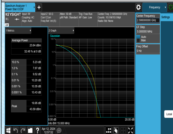
Band38-15MHz-QPSK-38000-1RB#0-PASS
