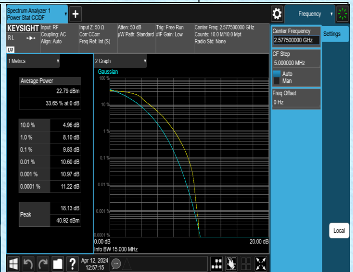
Band38-15MHz-QPSK-37825-75RB#0-PASS
