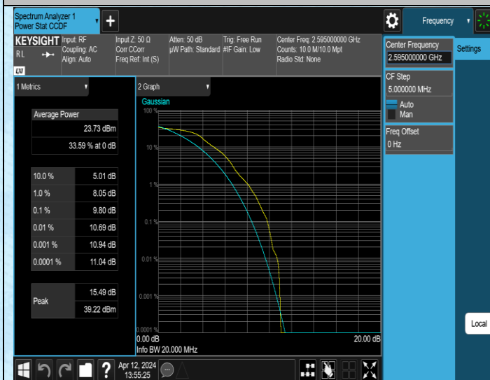
Band38-20MHz-QPSK-38000-1RB#0-PASS
