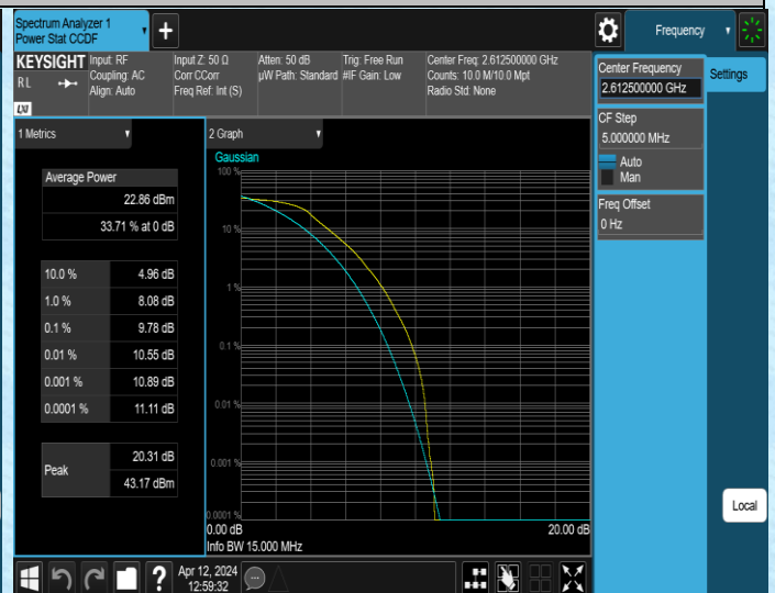
Band38-15MHz-QPSK-38175-75RB#0-PASS
