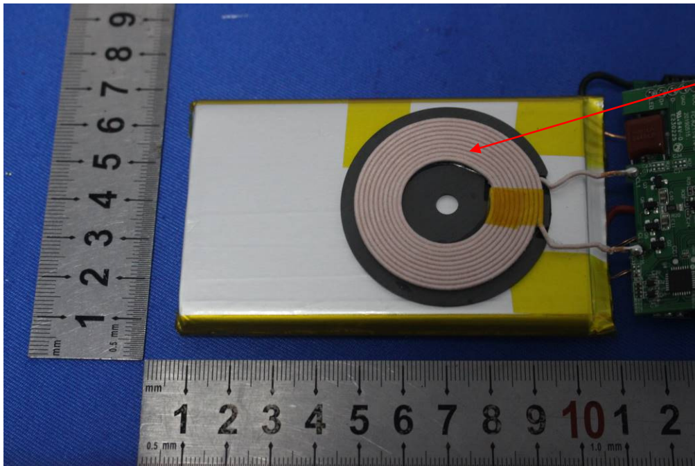
Transmitter antenna
