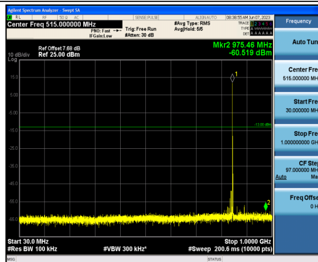
Band5-1.4MHz-16QAM-20643-1-0-Low-30-1000--60.52-PASS
