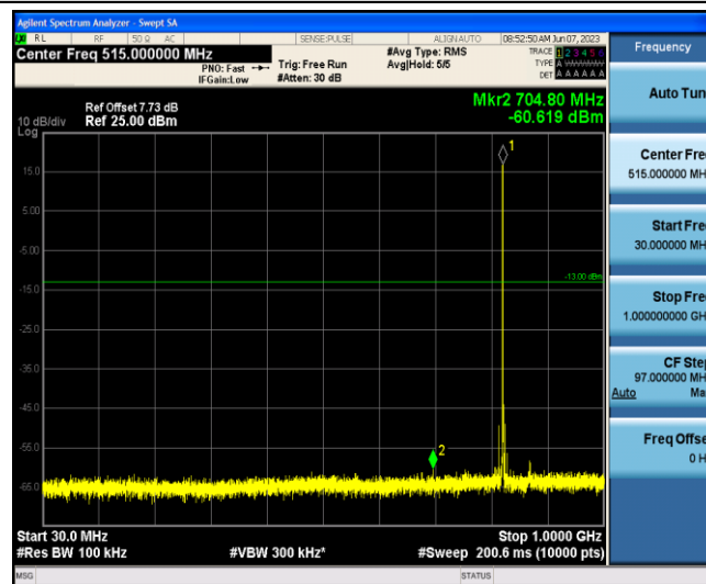
Band5-3MHz-16QAM-20415-1-0-Low-30-1000--60.62-PASS
