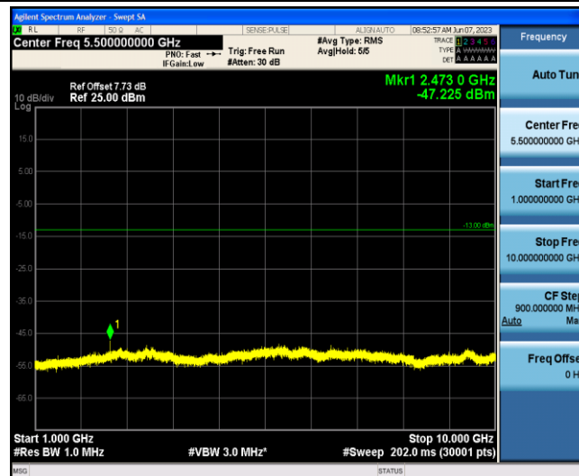
Band5-3MHz-16QAM-20415-1-0-Low-1000-10000--47.23-PASS
