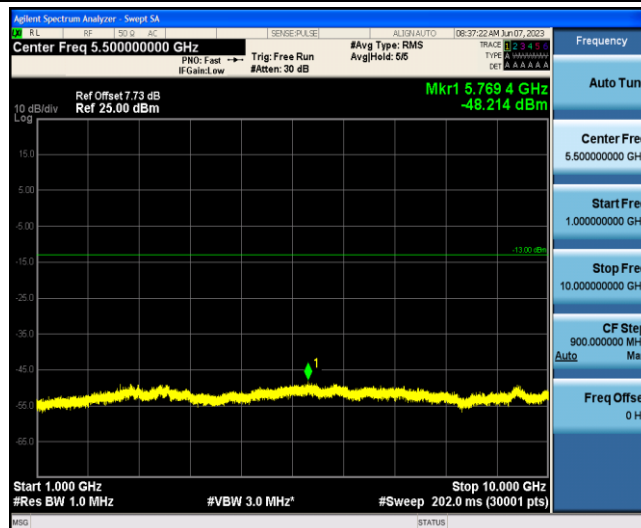
Band5-1.4MHz-QPSK-20407-1-0-Low-1000-10000--48.21-PASS
