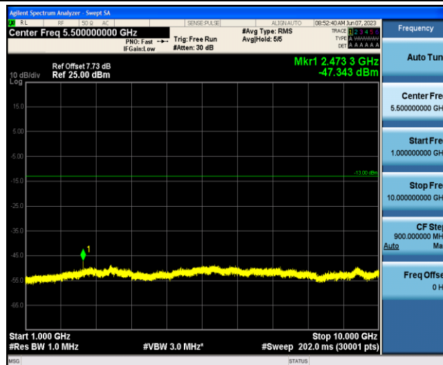
Band5-3MHz-QPSK-20415-1-0-Low-1000-10000--47.34-PASS
