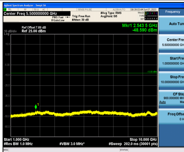
Band5-1.4MHz-16QAM-20643-1-0-Low-1000-10000--48.59-PASS
