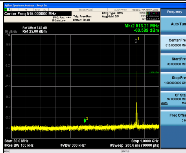
Band5-1.4MHz-QPSK-20643-1-0-Low-30-1000--60.59-PASS
