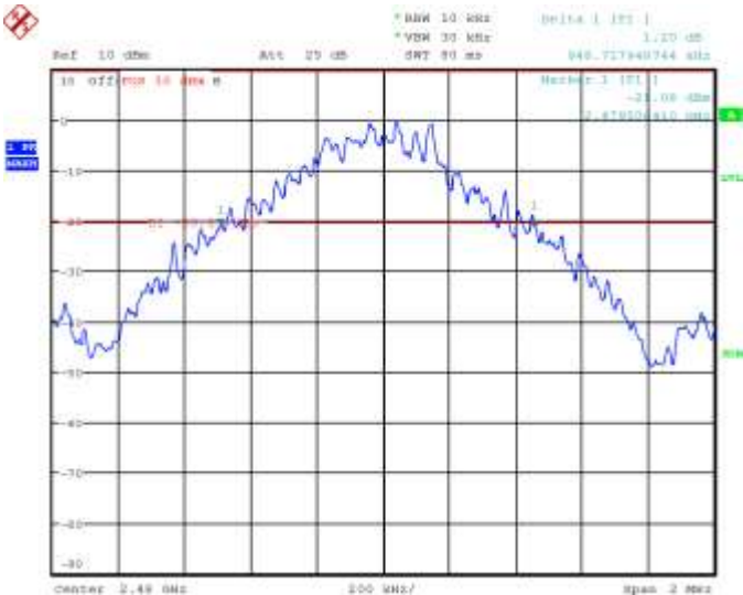
Figure 5-3: 20 dB Bandwidth Single freq., Static PBRs, DH5
