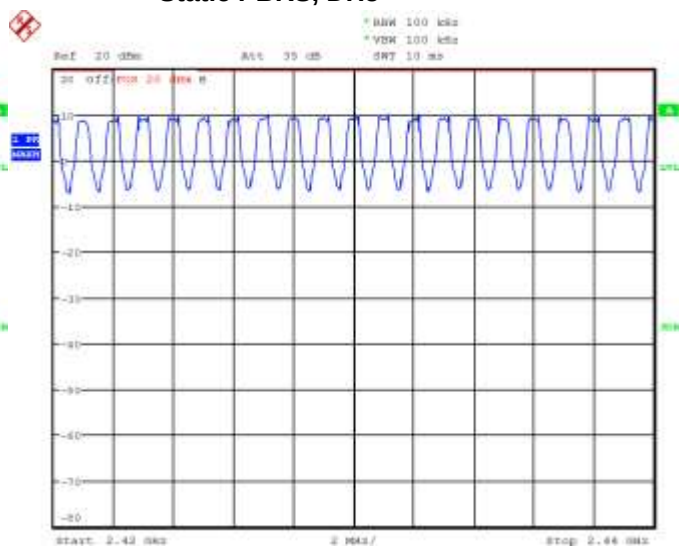
Figure 5-14: Number of Hopping Frequencies Static PBRs, DH5
