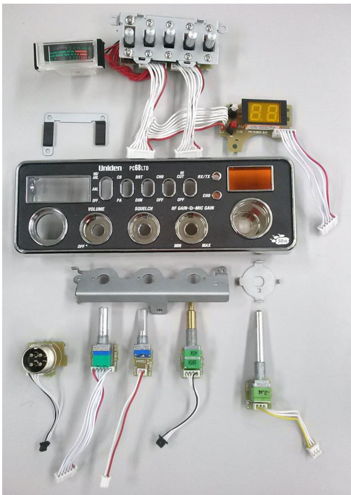
PC68LTD Front Top
