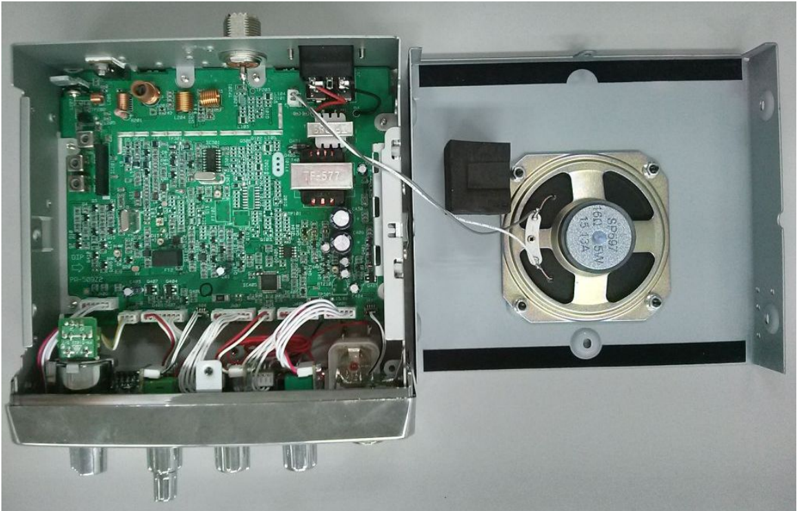
PC68LTD Main Top View w/ Speaker Wiring
