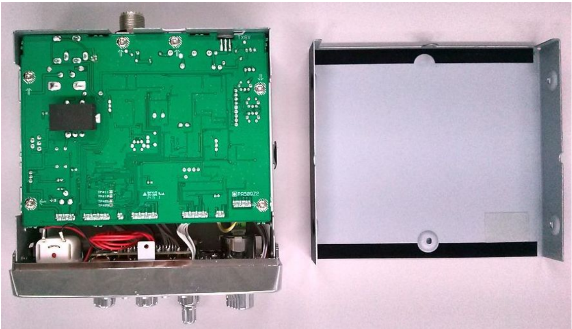
PC68LTD Main Bottom View w/ Cover
