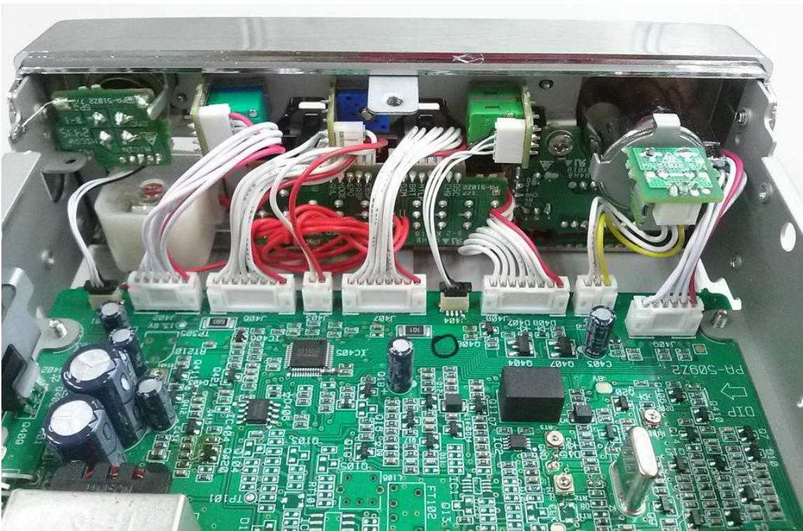
PC68LTD Front Inner View
