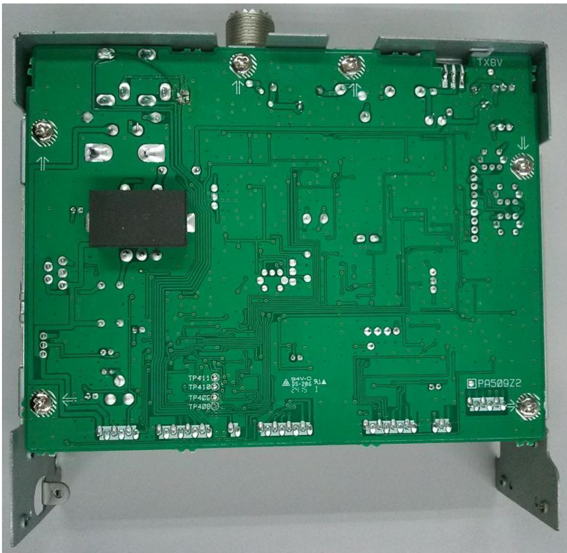
PC68LTD Main Bottom View
