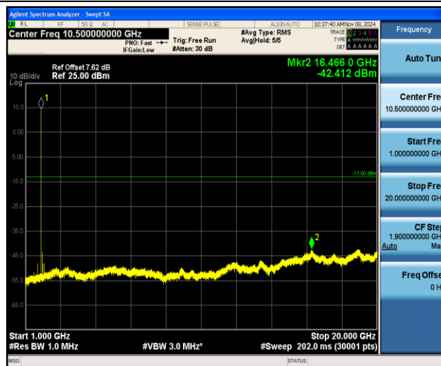
Band25-10MHz-16QAM-26090-1-0-Low-1000-20000--42.41-PASS
