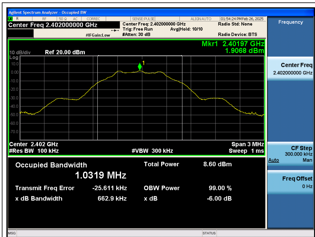
Test_Graph_LE1M_ANT1_2402_1Mbps_DTSBW
