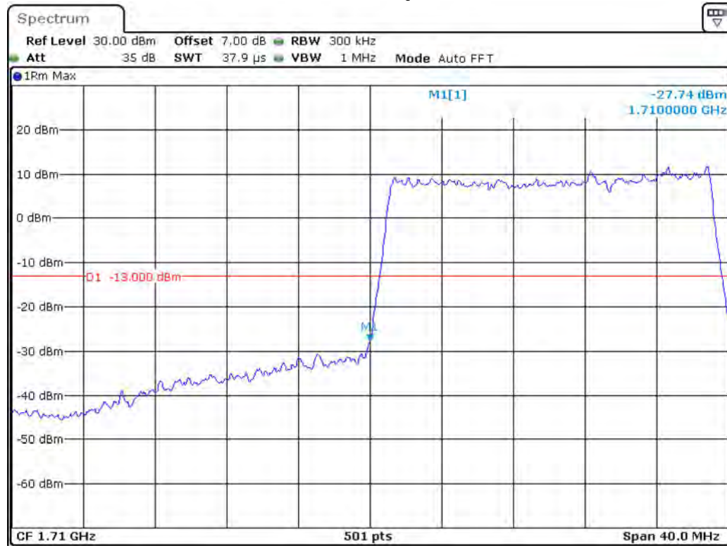
Band 4_20 MHz_Low_QPSK_RB100#0
