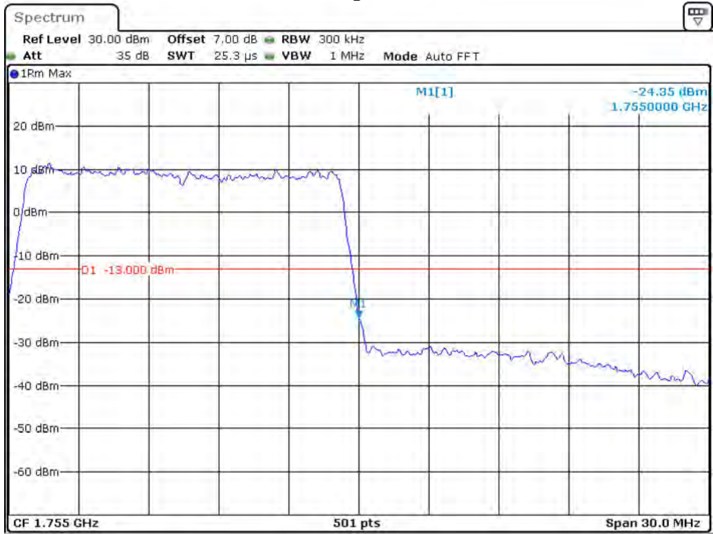
Band 4_15 MHz_High_16QAM_RB75#0
