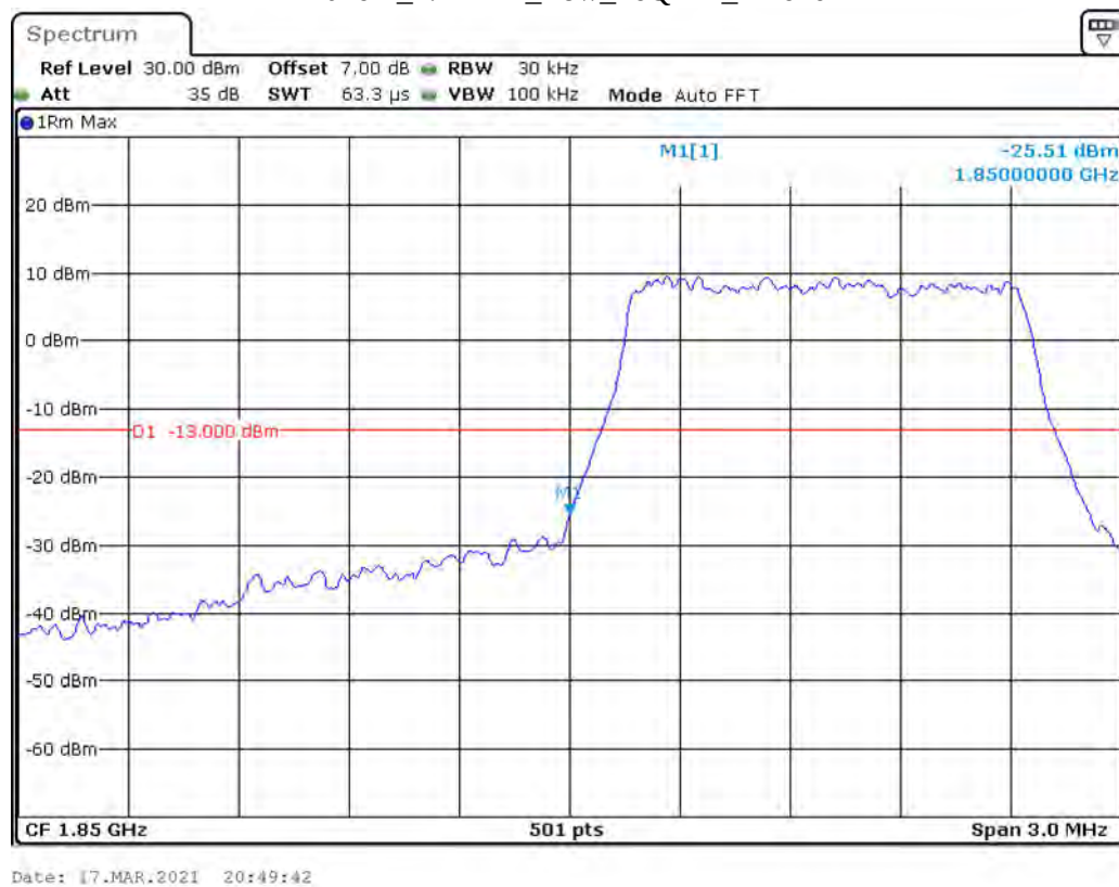
Band 2_1.4 MHz_Low_16QAM_RB6#0
