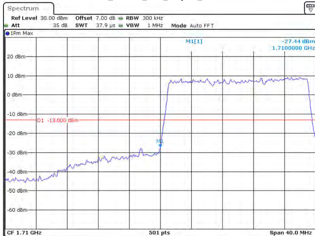
Band 4_20 MHz_Low_16QAM_RB100#0
