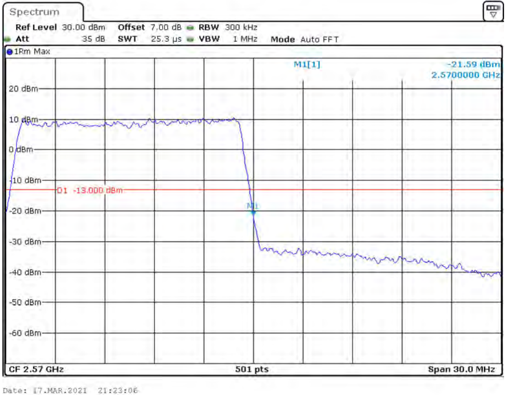
Band 7_15 MHz_High_QPSK_RB75#0
