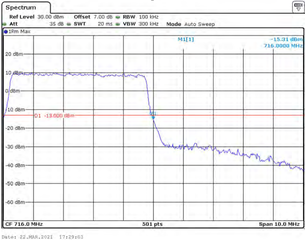
Band 17_5 MHz_High_16QAM_RB25#0
