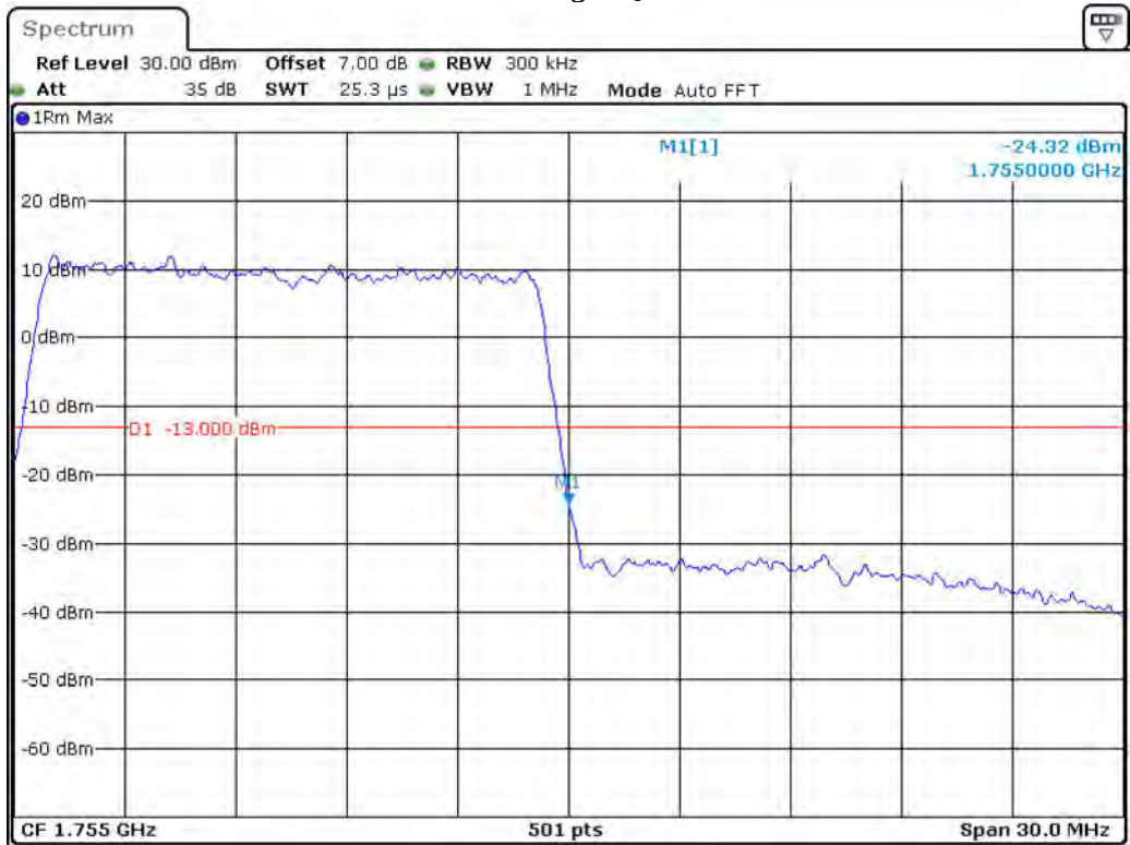
Band 4_15 MHz_High_QPSK_RB75#0
