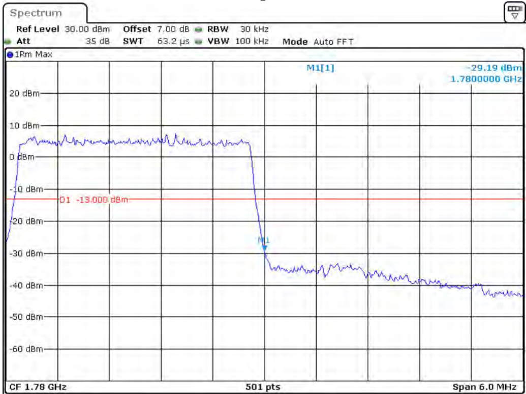
Band 66_3 MHz_High_16QAM_RB15#0
