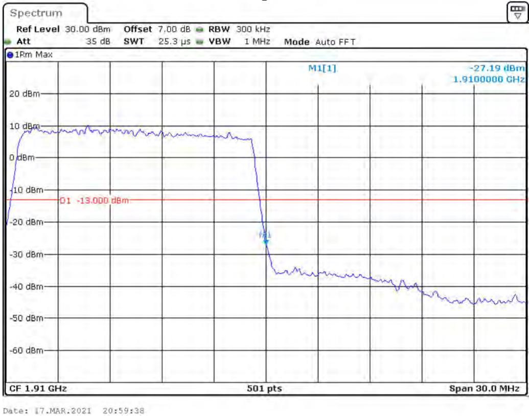
Band 2_15 MHz_High_16QAM_RB75#0
