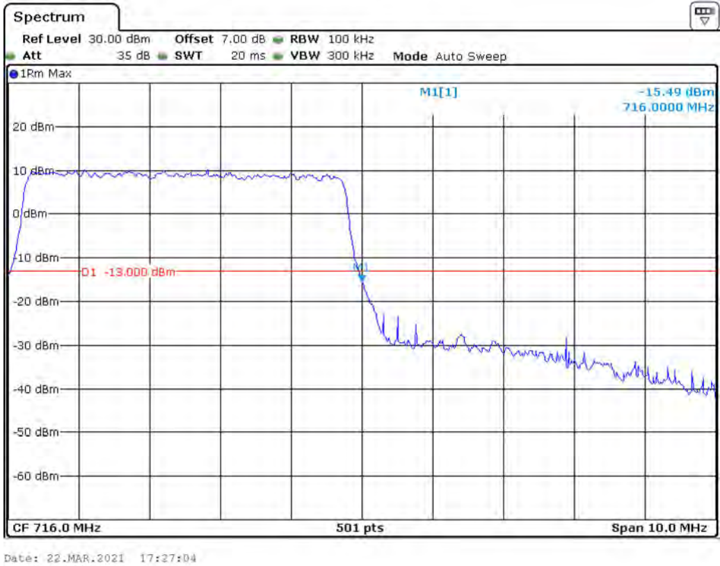
Band 17_5 MHz_High_QPSK_RB25#0
