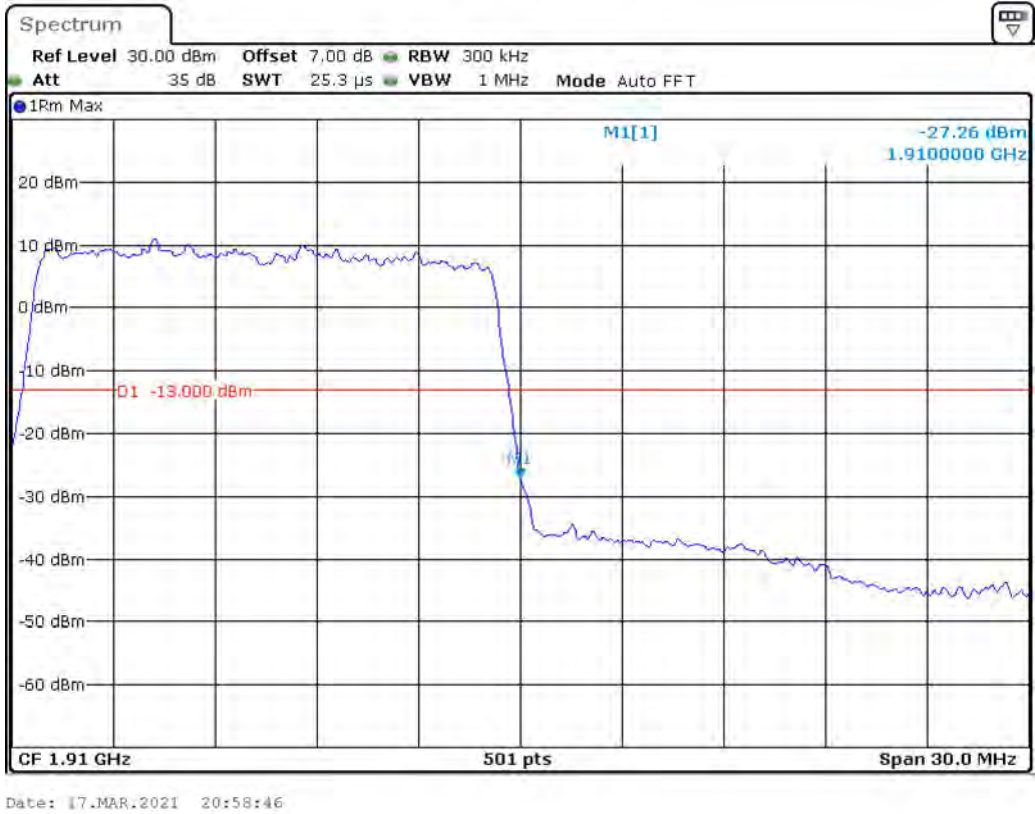
Band 2_15 MHz_High_QPSK_RB75#0
