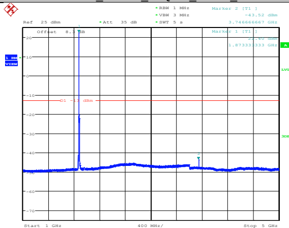
Band2_15MHz_16QAM_18900_1RB#0
