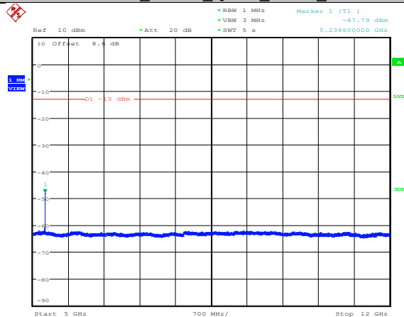
Band4_10MHz_QPSK_20350_1RB#0
