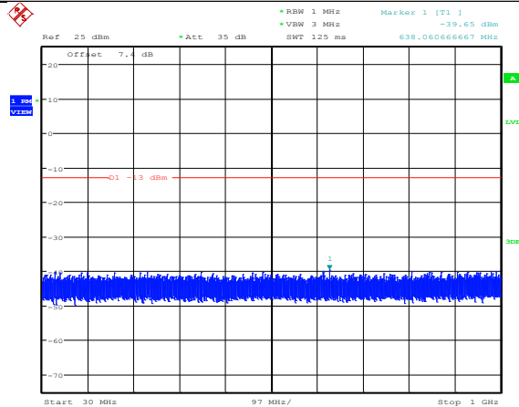
Band4_1.4MHz_16QAM_20175_1RB#0
