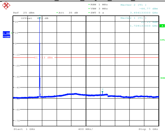
Band4_10MHz_16QAM_20175_1RB#0
