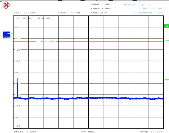
Band4_5MHz_16QAM_20175_1RB#0
