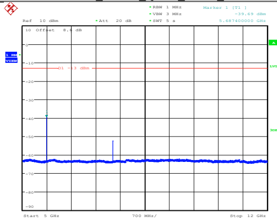
Band2_15MHz_QPSK_19125_1RB#0
