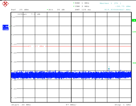
Band2_3MHz_16QAM_18900_1RB#0
