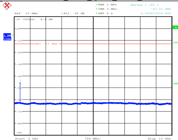
Band4_5MHz_QPSK_20375_1RB#0
