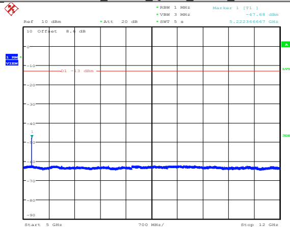
Band4_15MHz_QPSK_20325_1RB#0
