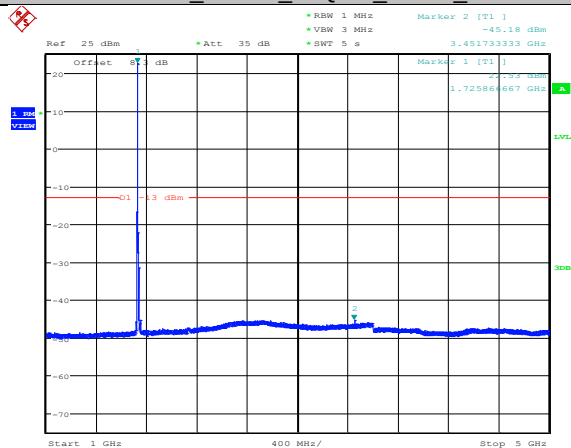
Band4_15MHz_16QAM_20175_1RB#0
