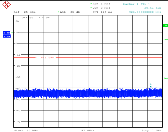
Band4_5MHz_QPSK_19975_1RB#0
