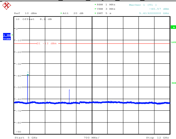
Band2_20MHz_16QAM_18900_1RB#0
