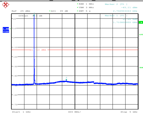
Band4_15MHz_QPSK_20025_1RB#0
