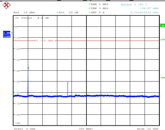
Band2_10MHz_QPSK_19150_1RB#0
