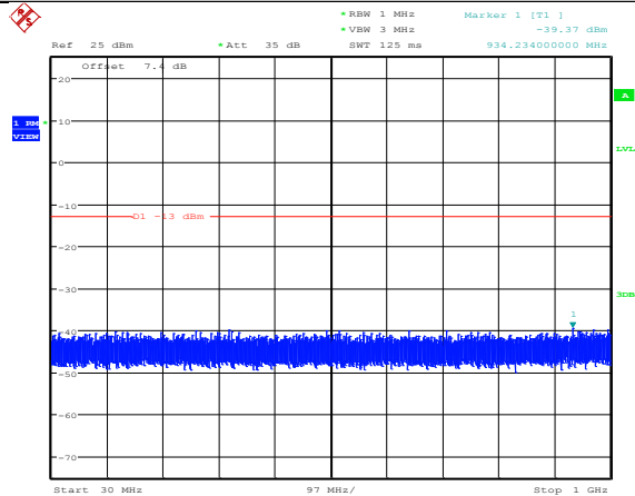
Band4_1.4MHz_QPSK_20393_1RB#0
