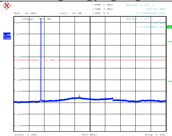
Band4_1.4MHz_QPSK_19957_1RB#0
