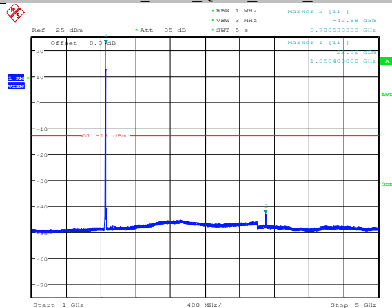
Band2_5MHz_QPSK_18625_1RB#0
