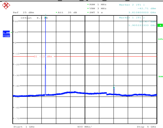
Band2_5MHz_QPSK_19175_1RB#0
