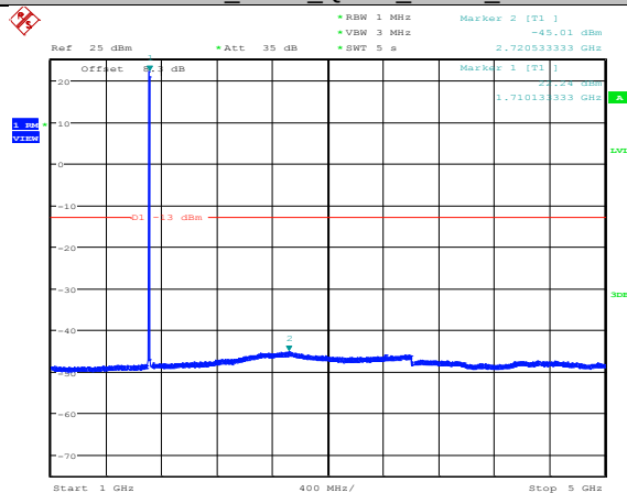
Band4_3MHz_QPSK_19965_1RB#0
