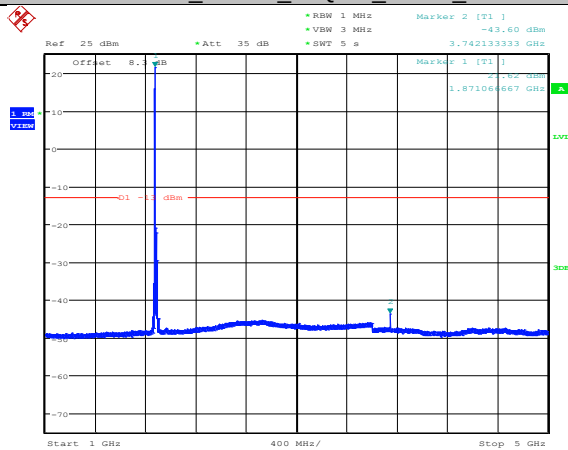
Band2_20MHz_16QAM_18900_1RB#0
