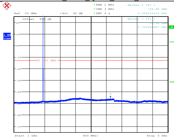
Band4_3MHz_QPSK_20385_1RB#0
