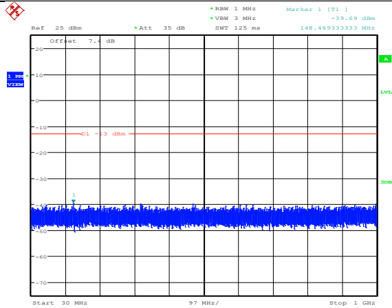
Band4_10MHz_16QAM_20175_1RB#0
