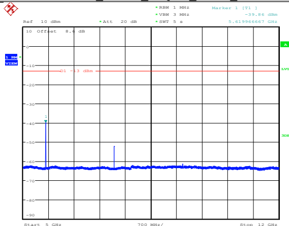
Band2_15MHz_16QAM_18900_1RB#0
