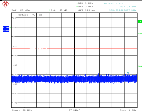
Band2_5MHz_16QAM_18900_1RB#0
