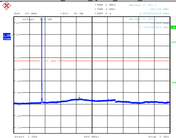
Band4_10MHz_QPSK_20000_1RB#0
