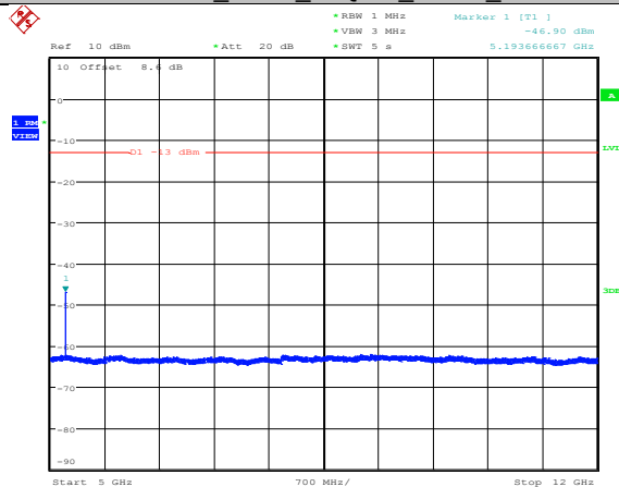
Band4_3MHz_16QAM_20175_1RB#0
