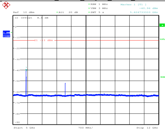
Band2_10MHz_16QAM_18900_1RB#0
