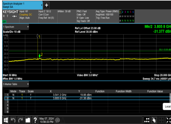
N78(10M)_DFT-s- OFDM_BPSK_Edge_1RB_Left_High_CH
