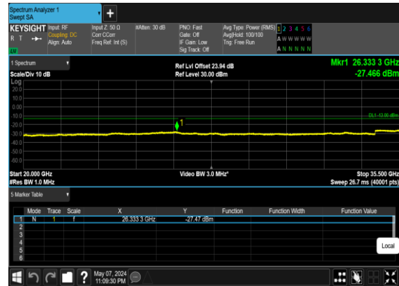
N78(100M)_DFT-s- OFDM_BPSK_Edge_1RB_Left_Mid_CH
