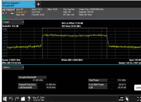
N78(50M)_CP- OFDM_QPSK_Outer_Full_Mid_CH
