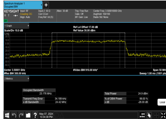
N78(25M)_CP-OFDM_16 QAM_Outer_Full_Mid_CH
