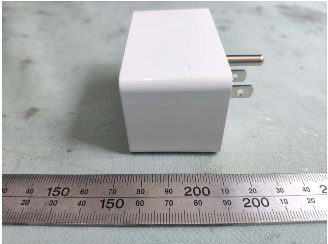
FIGURE 5 SMART PLUG (MODEL: CPLGSTDBLW1)(HVIN: CPLGSTDXCW1T) GENERAL APPEARANCE (RIGHT VIEW)
