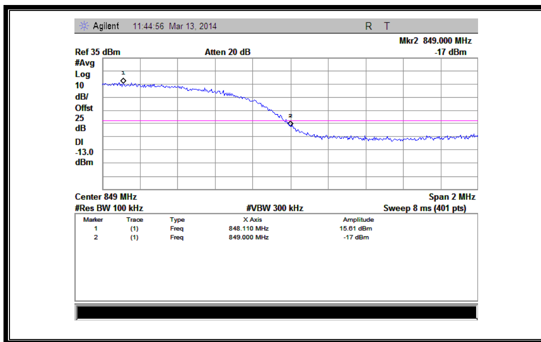
(Plot R: HSUPA850 Channel = 4233)
