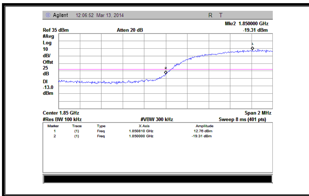
(Plot W: HSPA+ 1900 Channel = 9262)
