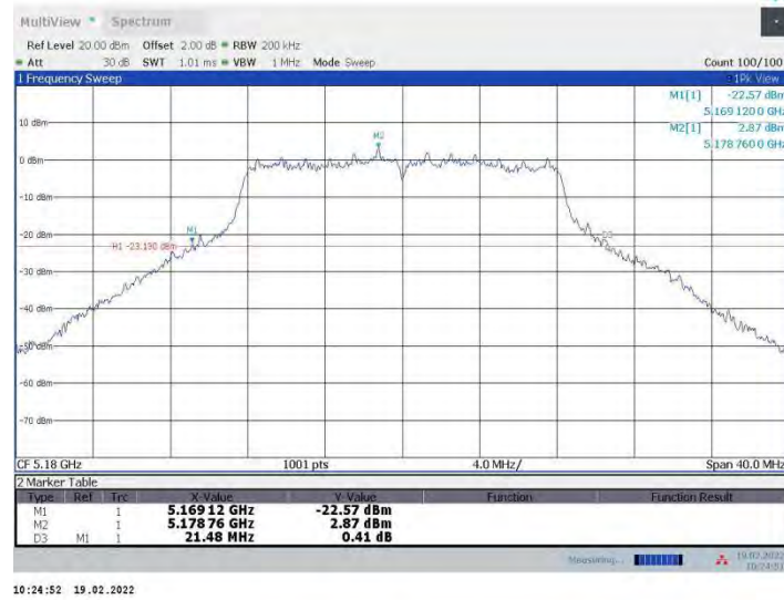
11a-CDD Ant3 5180
