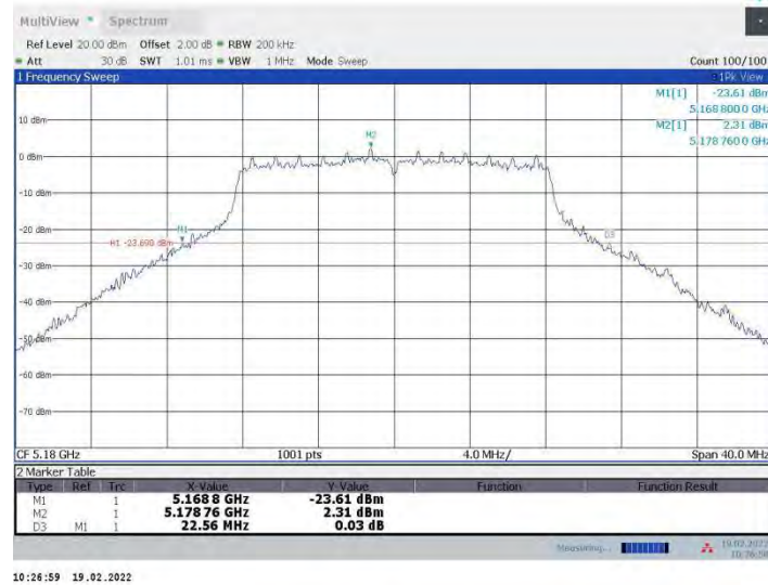
11a-CDD Ant2 5180
